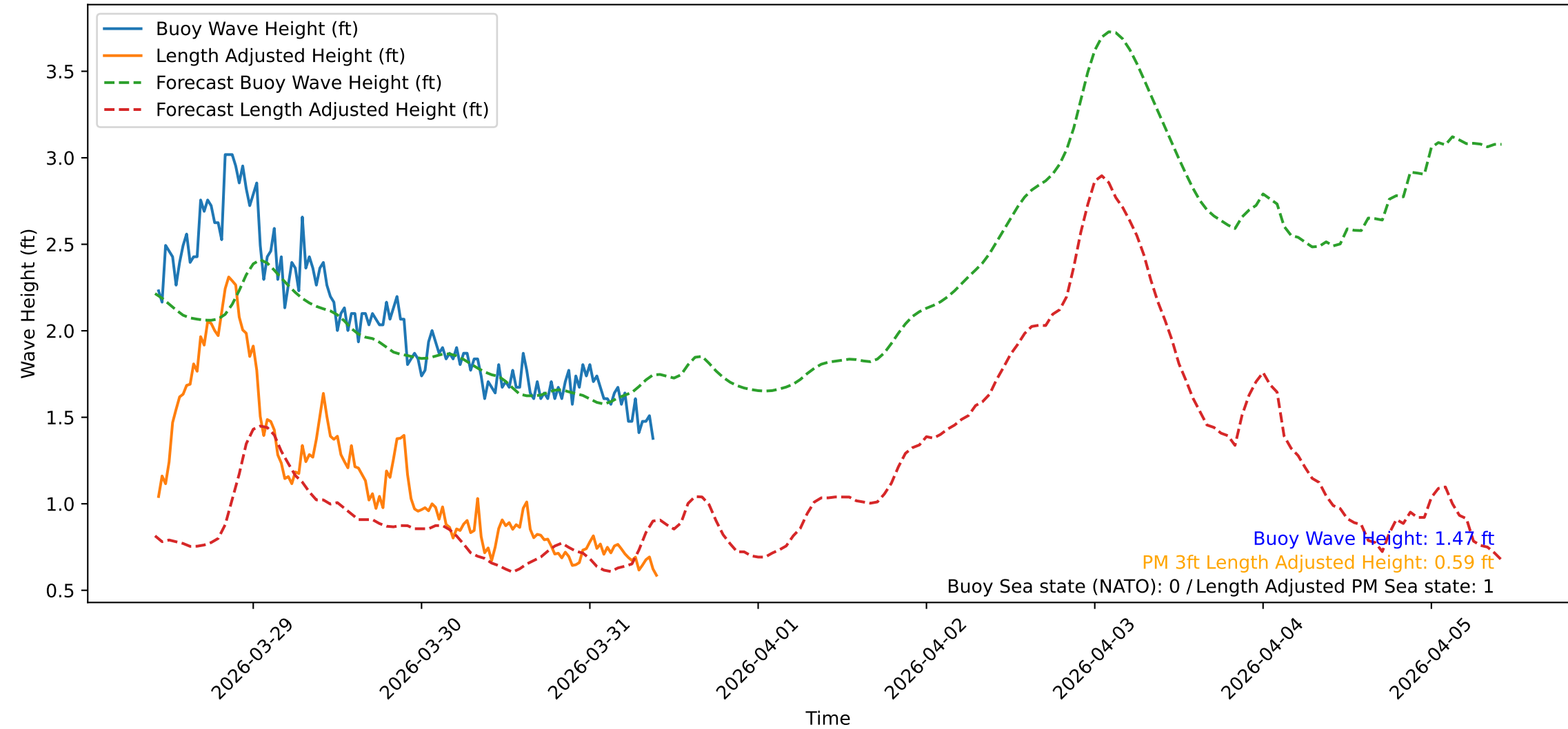
Wave Heights over Time for Red Beach at 2026-03-31 10:20:47
