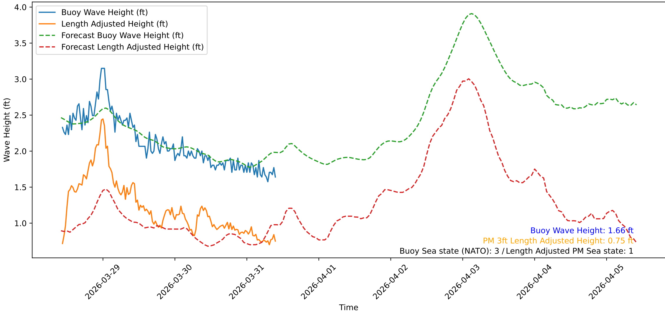
Wave Heights over Time for Oceanside Harbor at 2026-03-31 10:20:31
