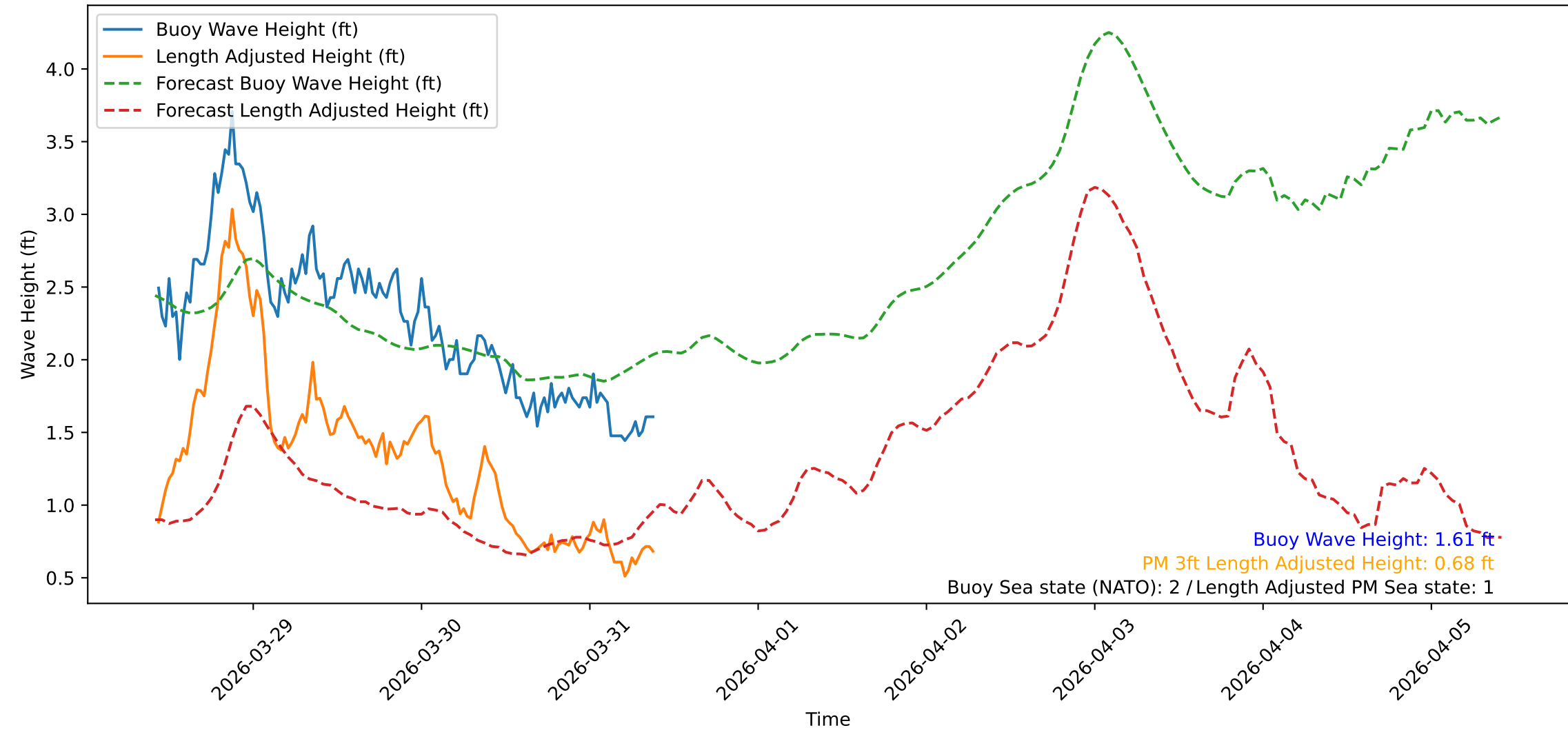
Wave Heights over Time for Green Beach at 2026-03-31 10:21:09
