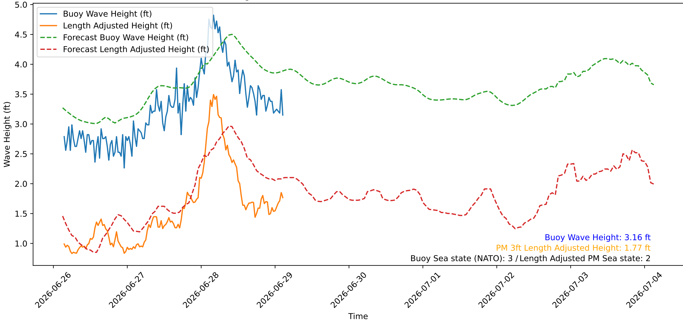
Wave Heights over Time for Green Beach at 2026-06-29 03:21:08
