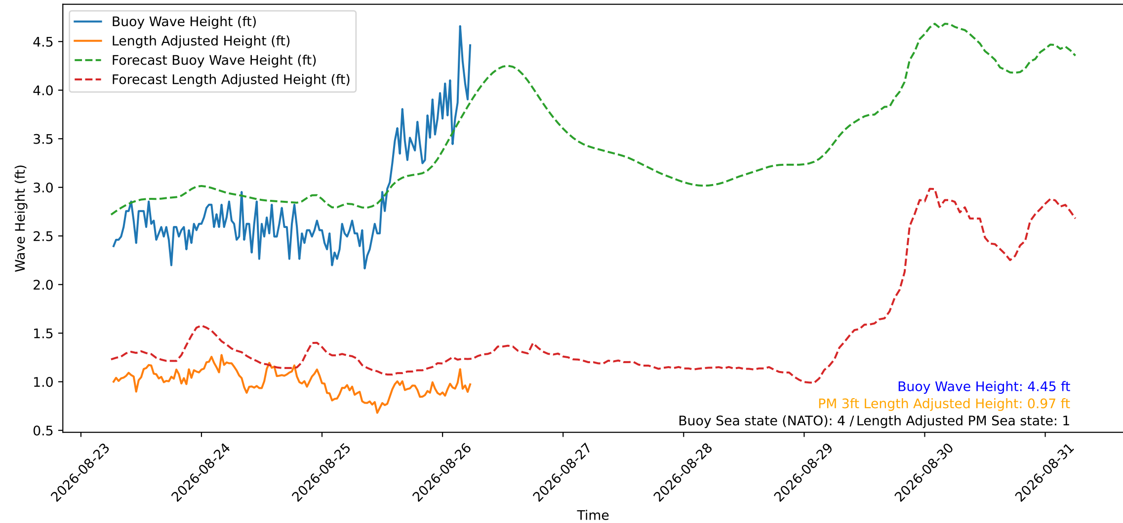
Wave Heights over Time for Red Beach at 2026-08-26 06:20:52
