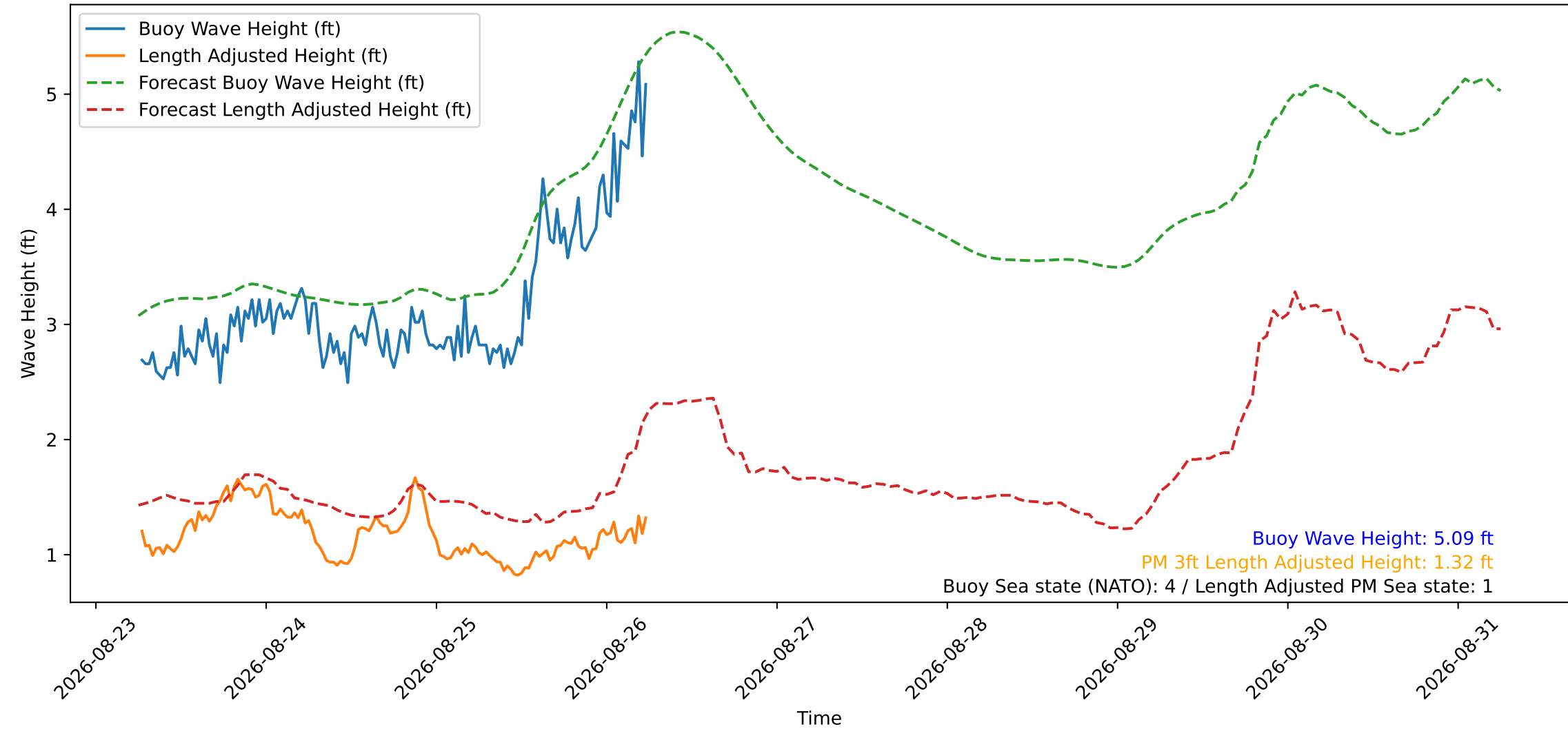
Wave Heights over Time for Green Beach at 2026-08-26 06:21:17
