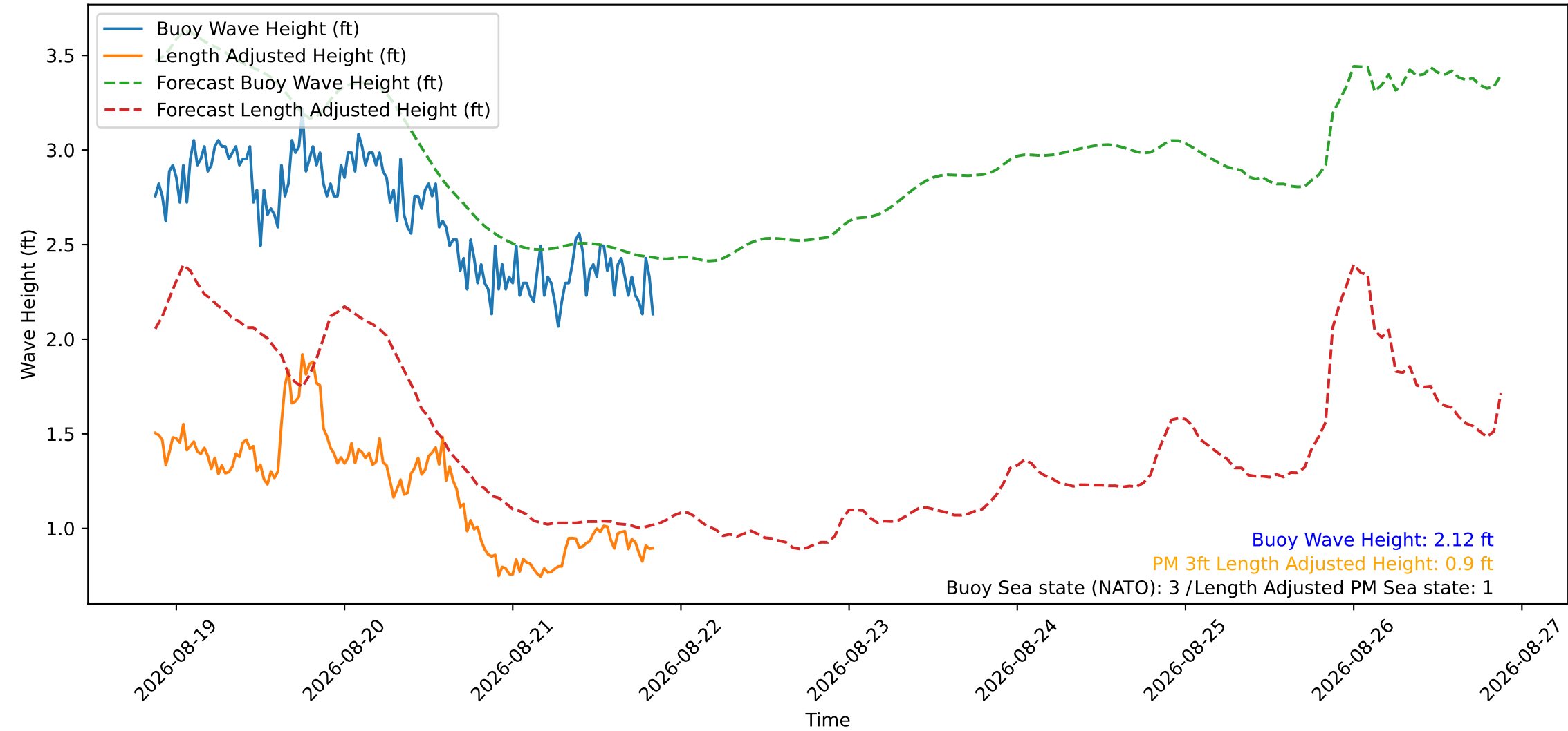
Wave Heights over Time for Red Beach at 2026-08-21 20:50:47
