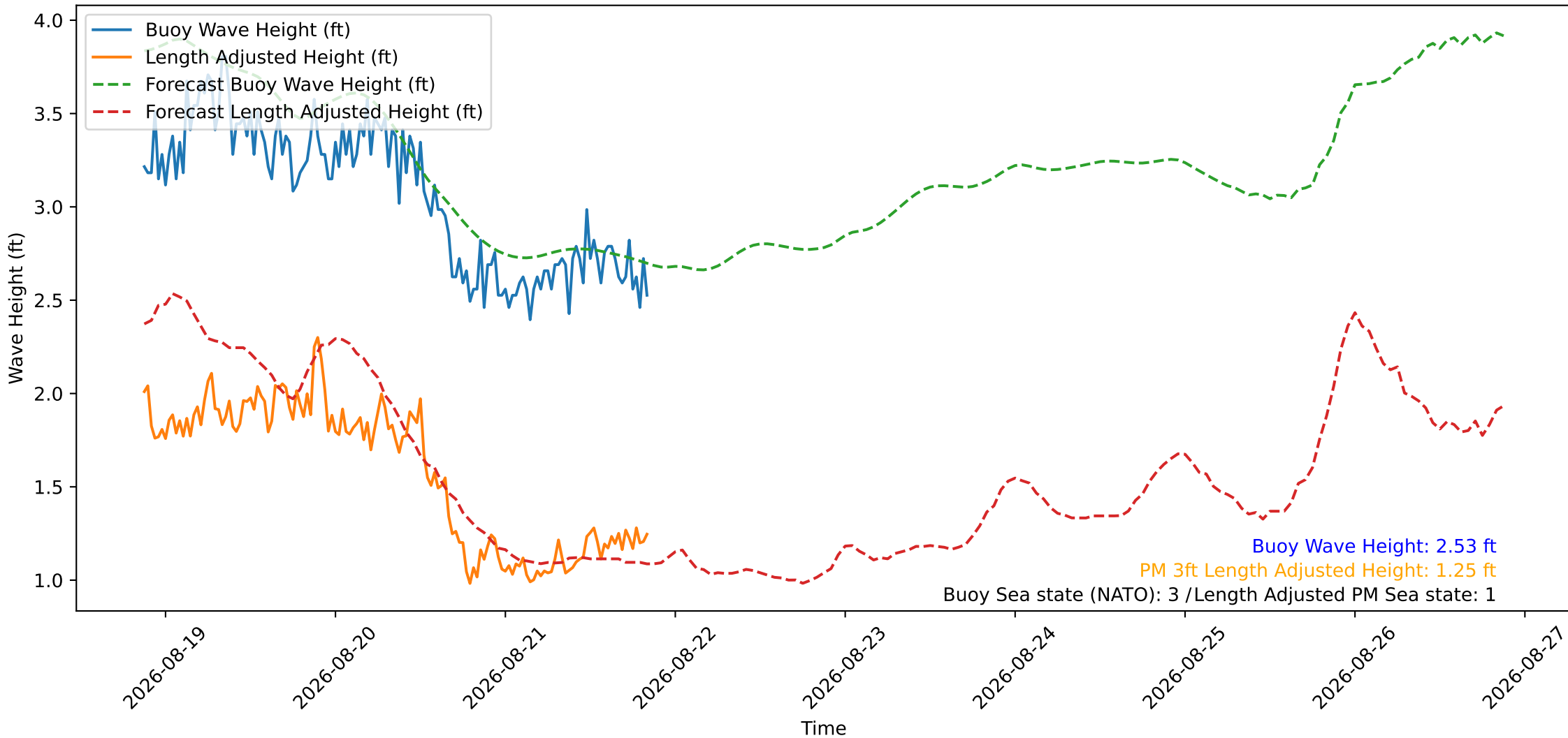
Wave Heights over Time for Oceanside Harbor at 2026-08-21 20:50:26
