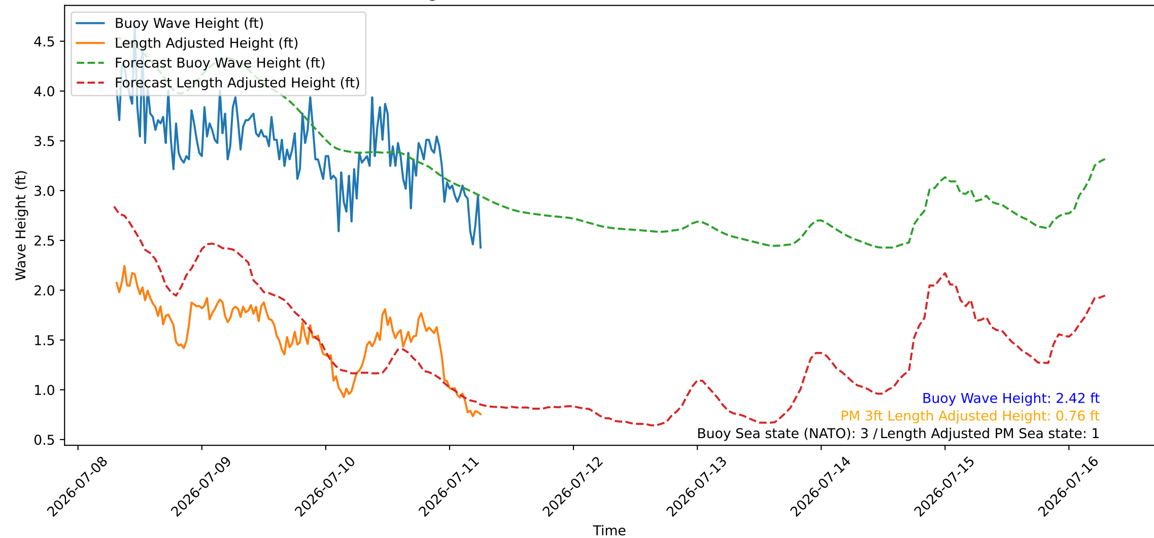
Wave Heights over Time for Red Beach at 2026-07-11 07:00:45
