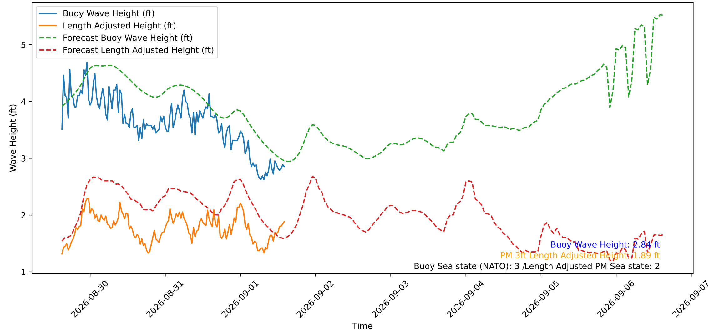
Wave Heights over Time for Red Beach at 2026-09-01 14:40:49
