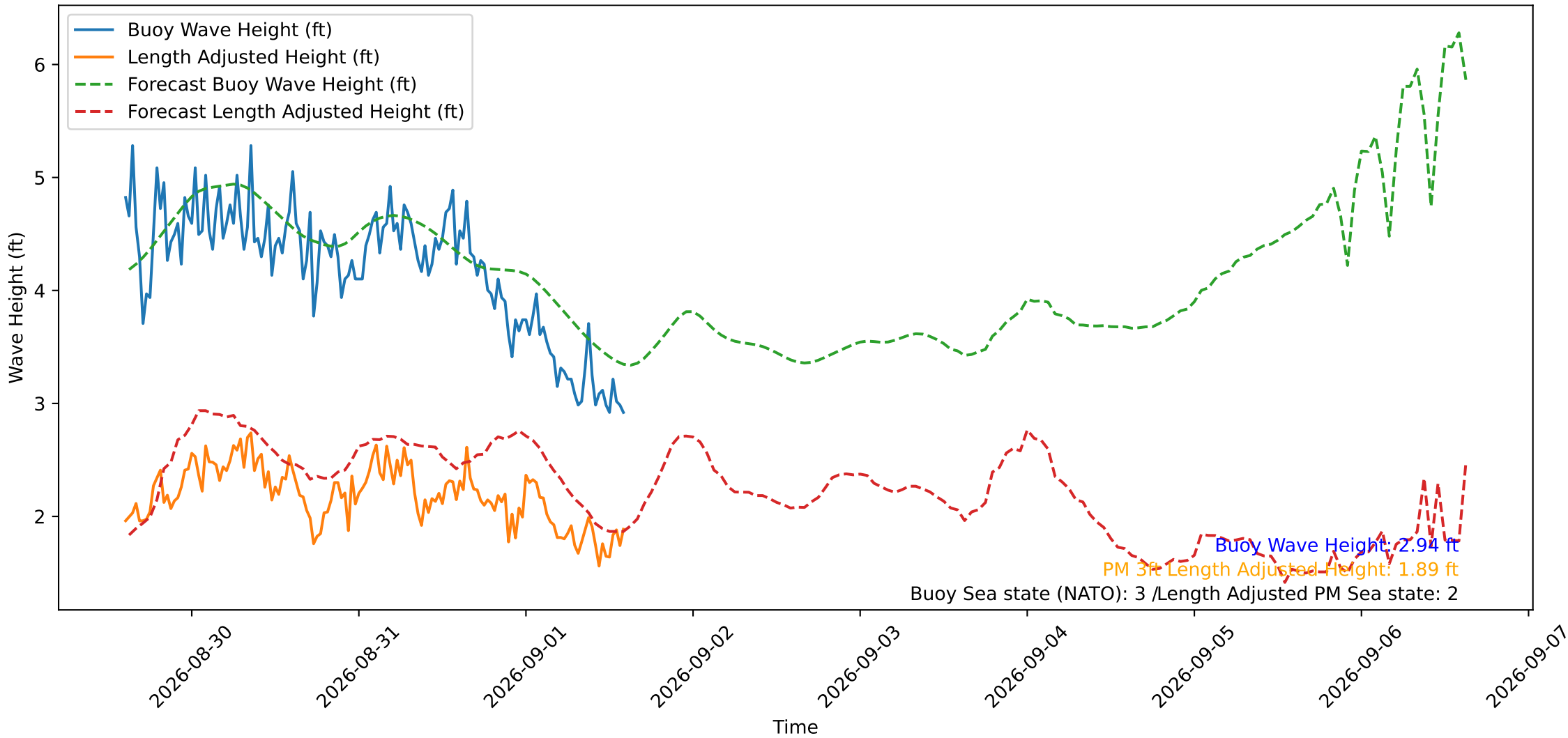
Wave Heights over Time for Oceanside Harbor at 2026-09-01 14:40:30
