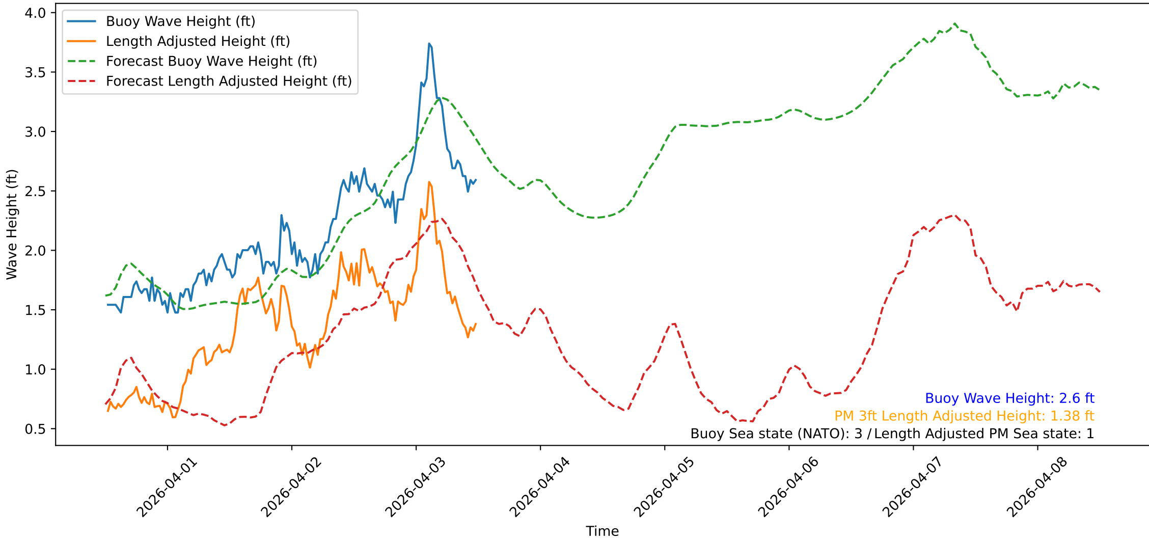
Wave Heights over Time for Red Beach at 2026-04-03 12:20:47
