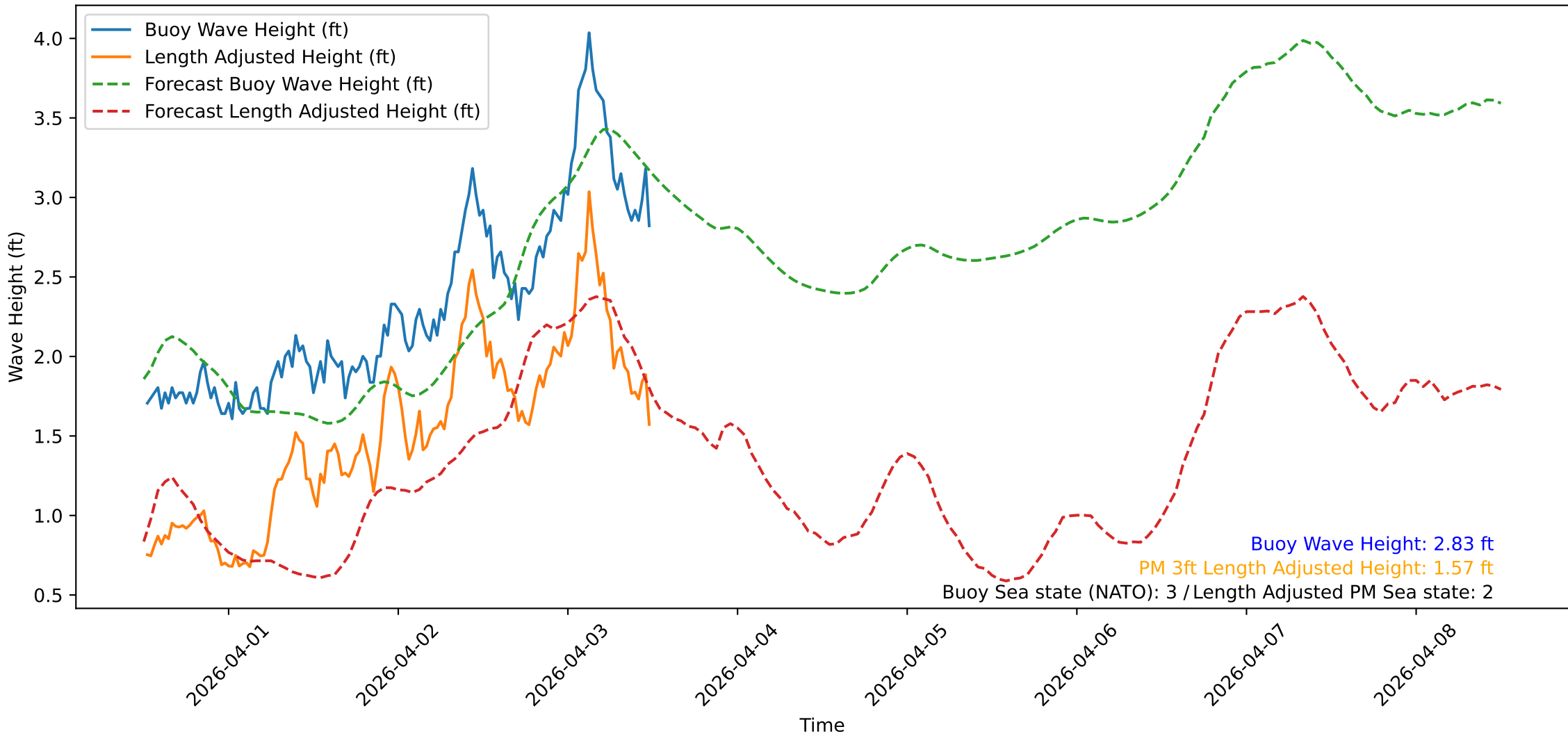
Wave Heights over Time for Oceanside Harbor at 2026-04-03 12:20:31
