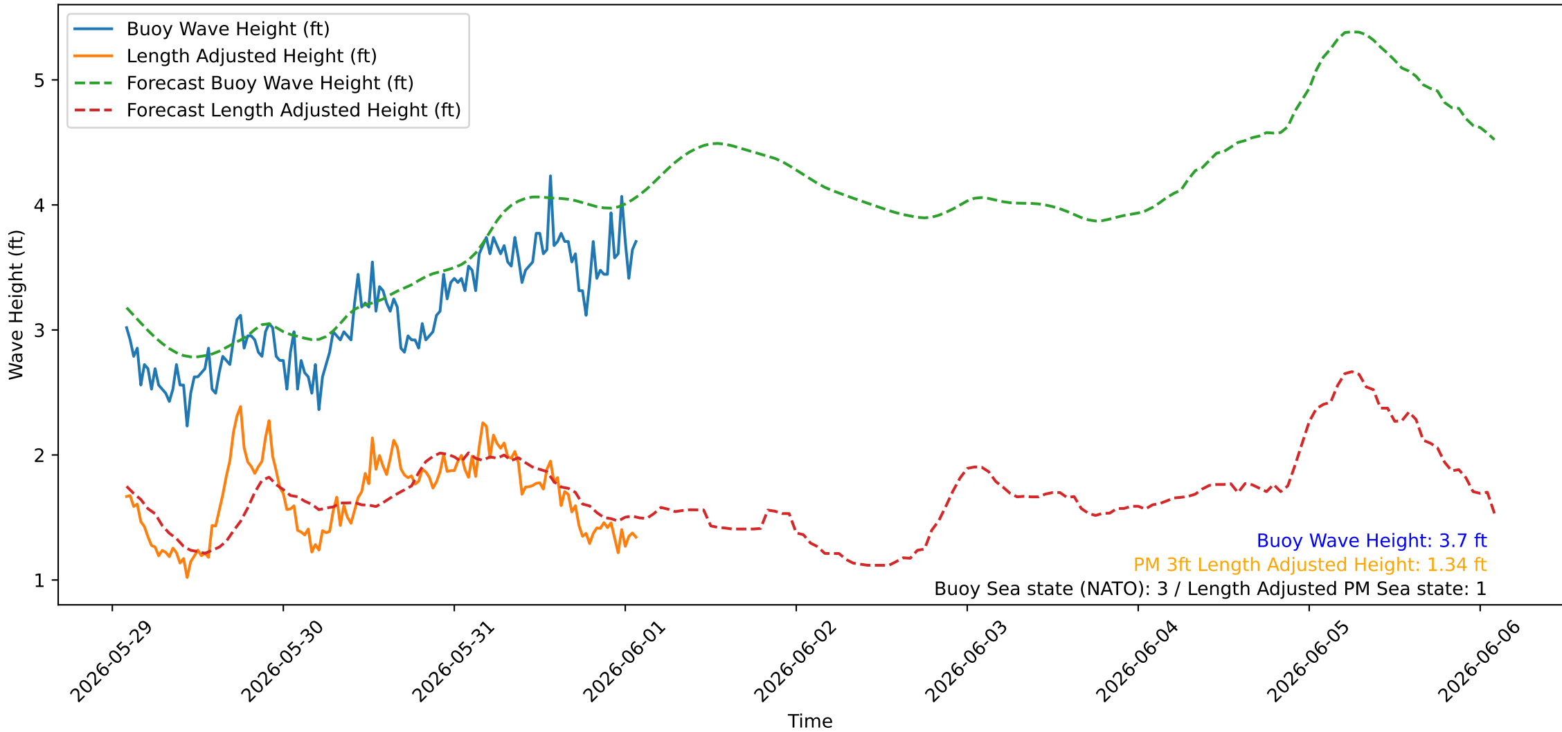
Wave Heights over Time for Oceanside Harbor at 2026-06-01 02:00:26
