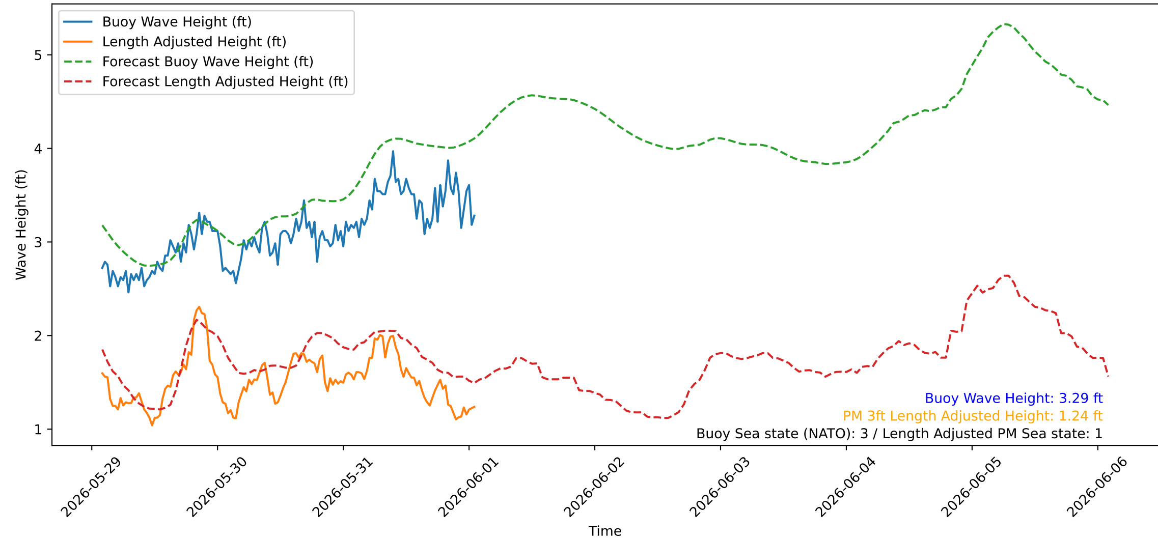
Wave Heights over Time for Green Beach at 2026-06-01 02:01:07
