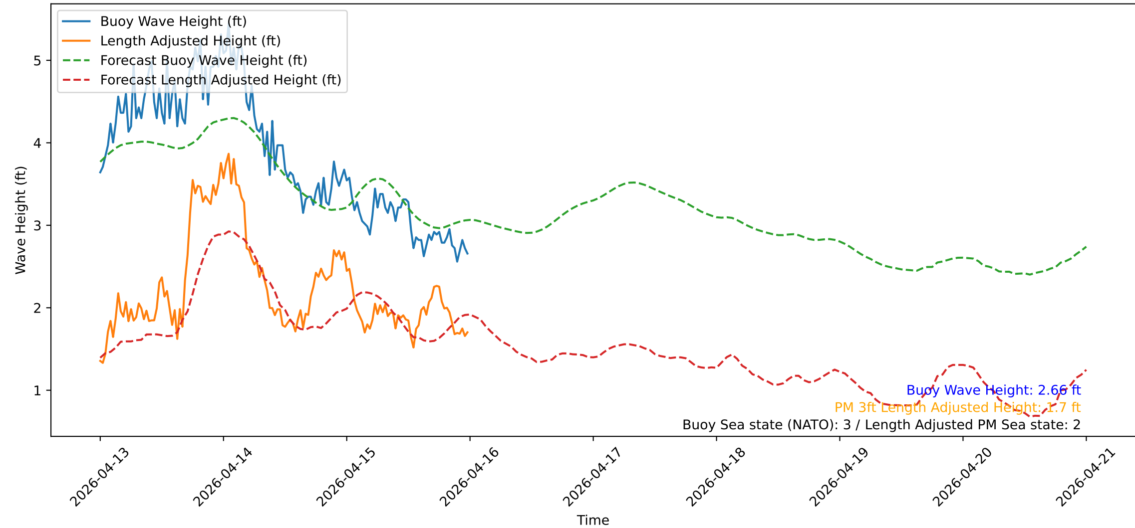
Wave Heights over Time for Oceanside Harbor at 2026-04-16 00:10:31
