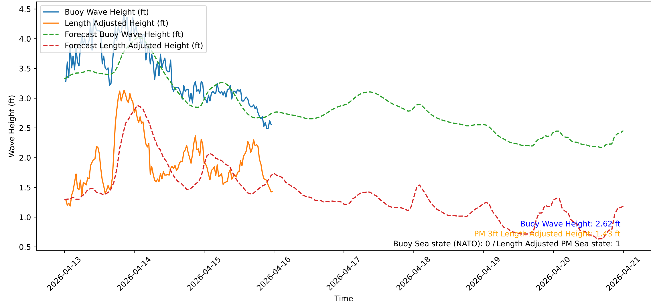
Wave Heights over Time for Red Beach at 2026-04-16 00:10:50
