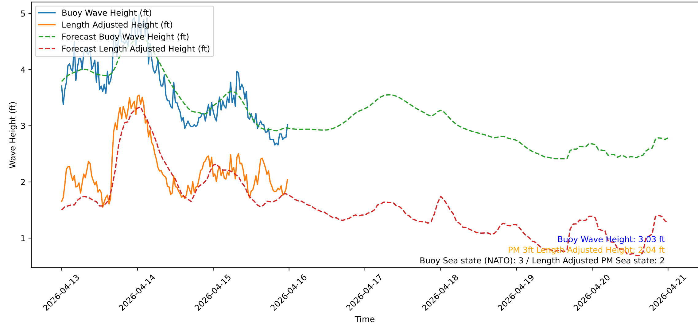
Wave Heights over Time for Green Beach at 2026-04-16 00:11:12
