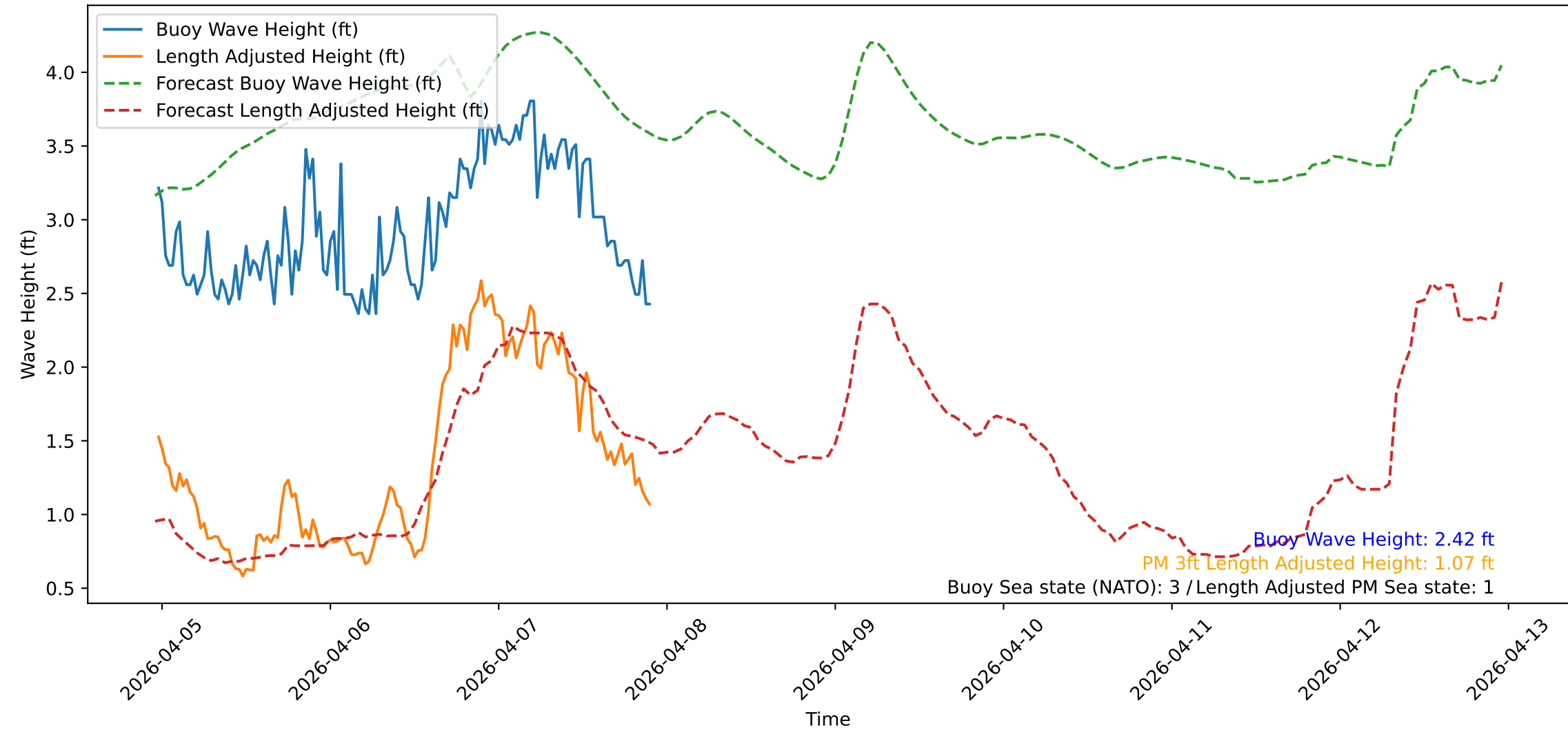
Wave Heights over Time for Green Beach at 2026-04-07 23:21:09
