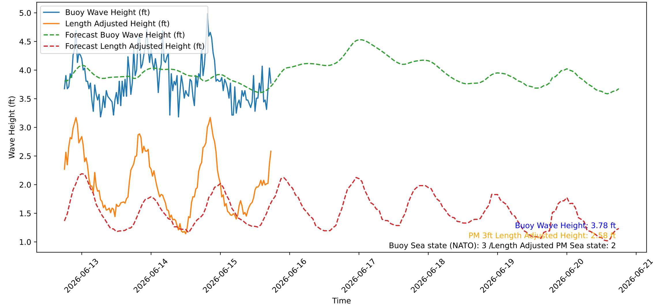
Wave Heights over Time for Oceanside Harbor at 2026-06-15 18:10:26
