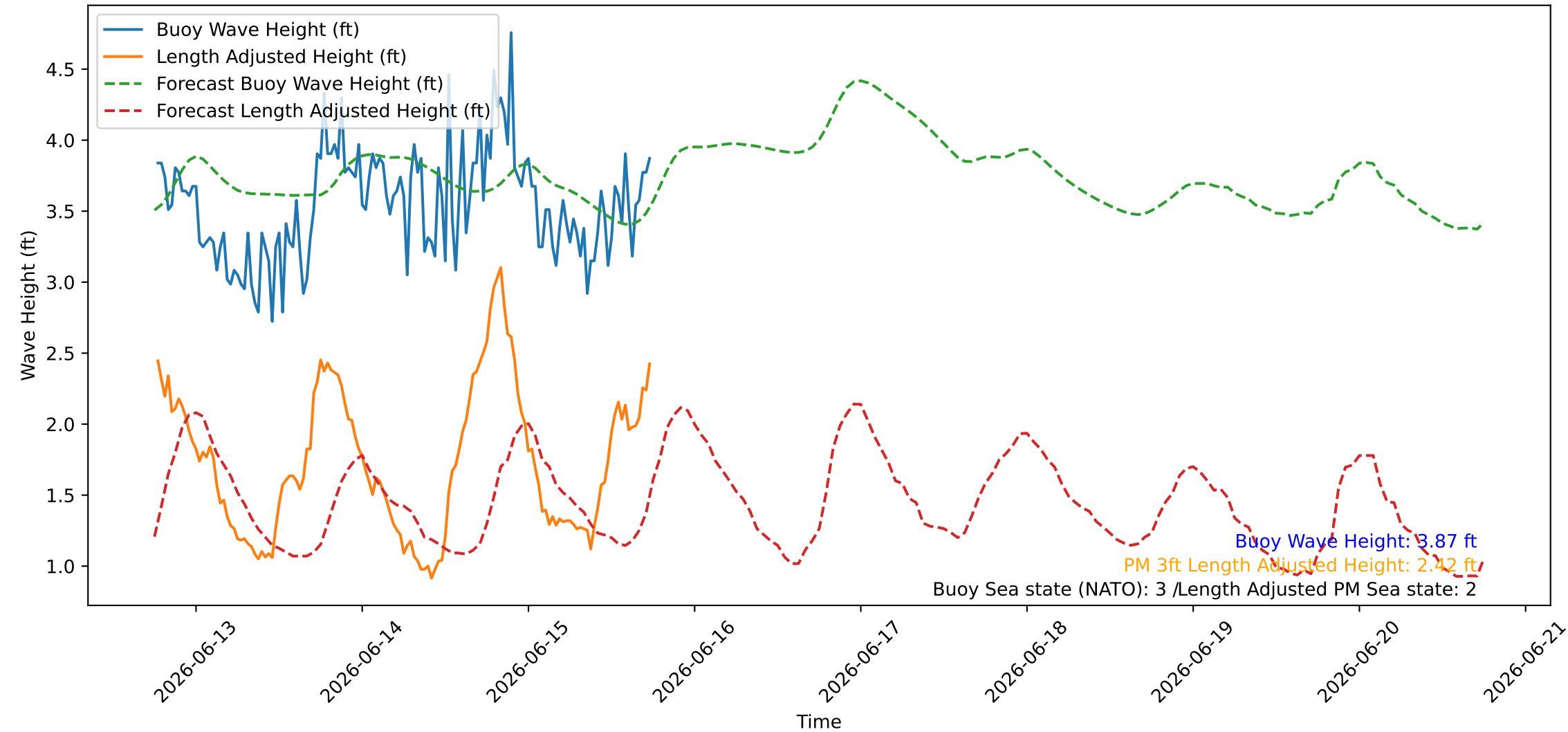
Wave Heights over Time for Red Beach at 2026-06-15 18:10:45
