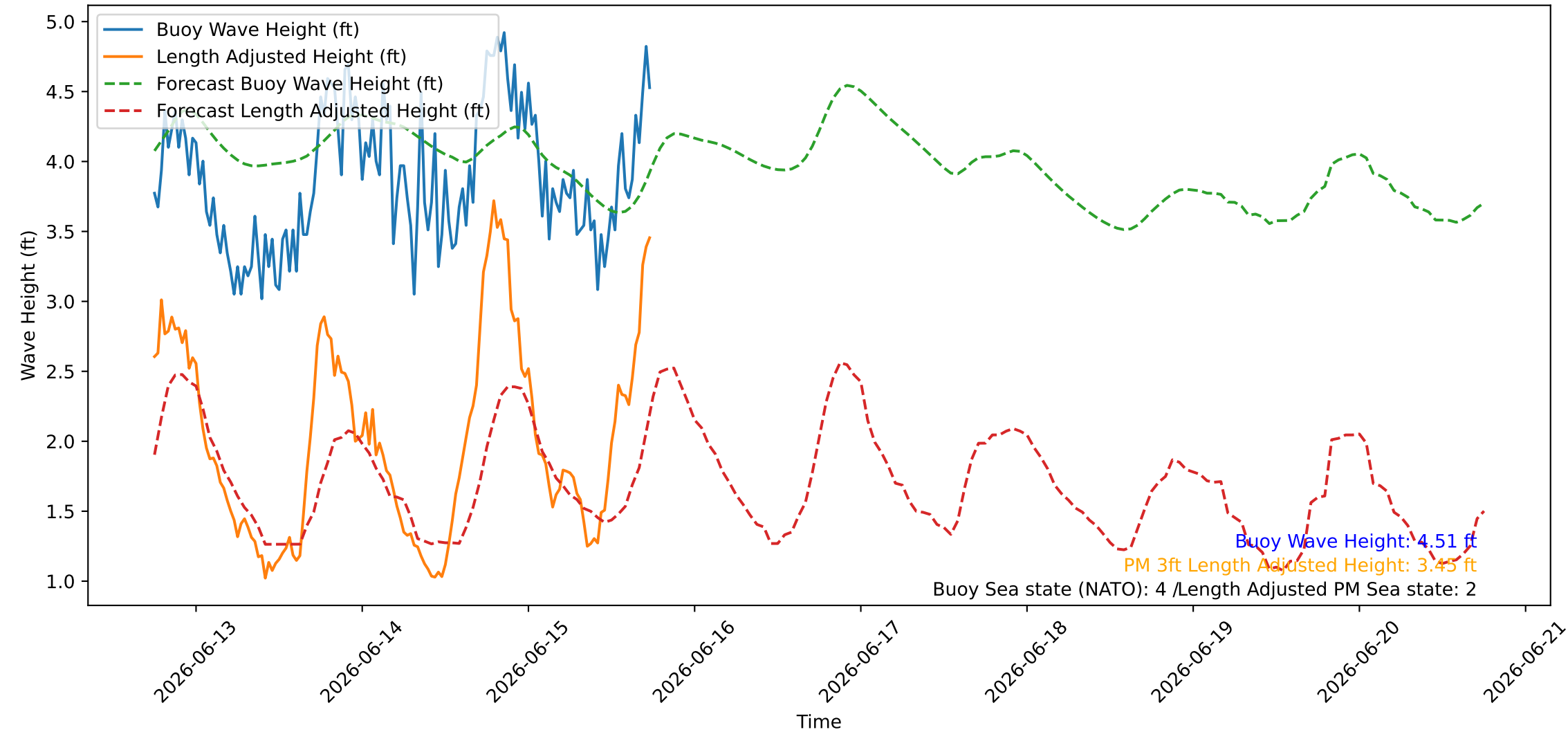
Wave Heights over Time for Green Beach at 2026-06-15 18:11:07
