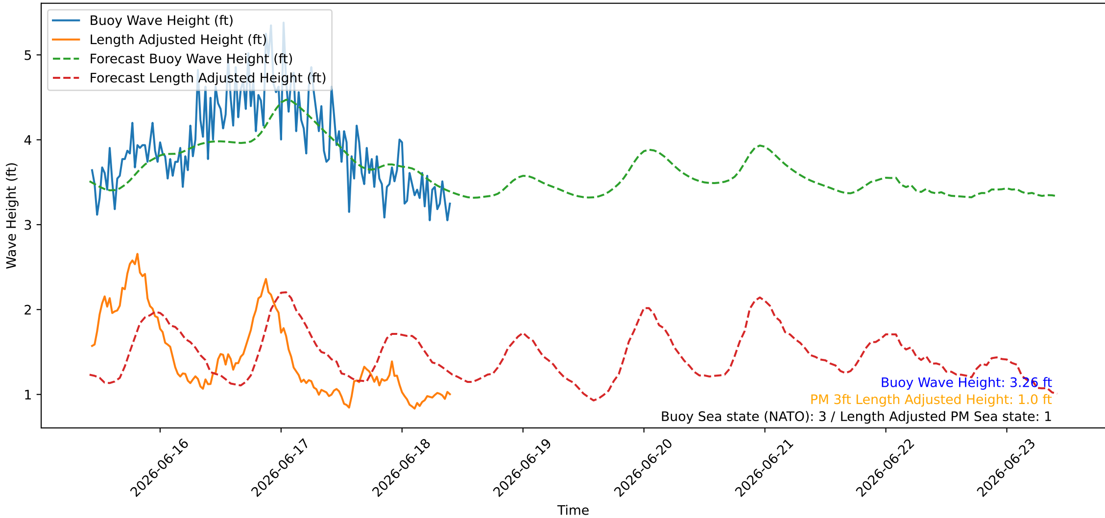
Wave Heights over Time for Red Beach at 2026-06-18 10:10:45
