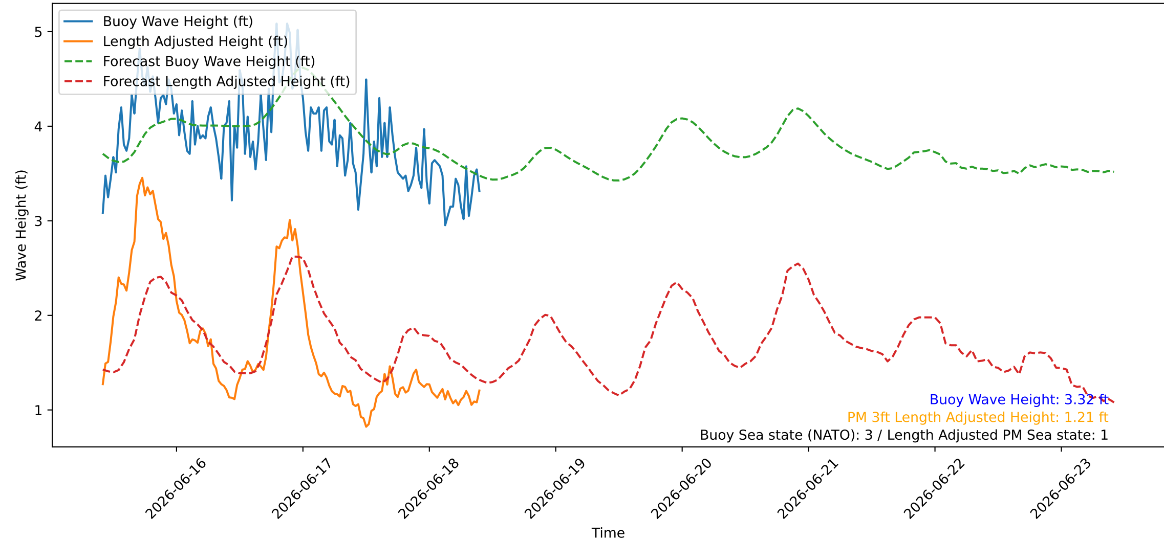
Wave Heights over Time for Green Beach at 2026-06-18 10:11:08
