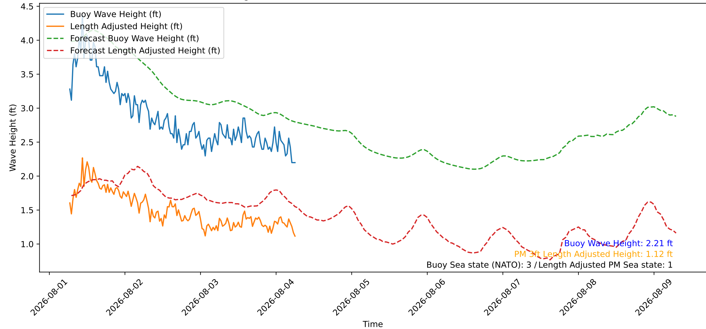
Wave Heights over Time for Oceanside Harbor at 2026-08-04 06:40:26
