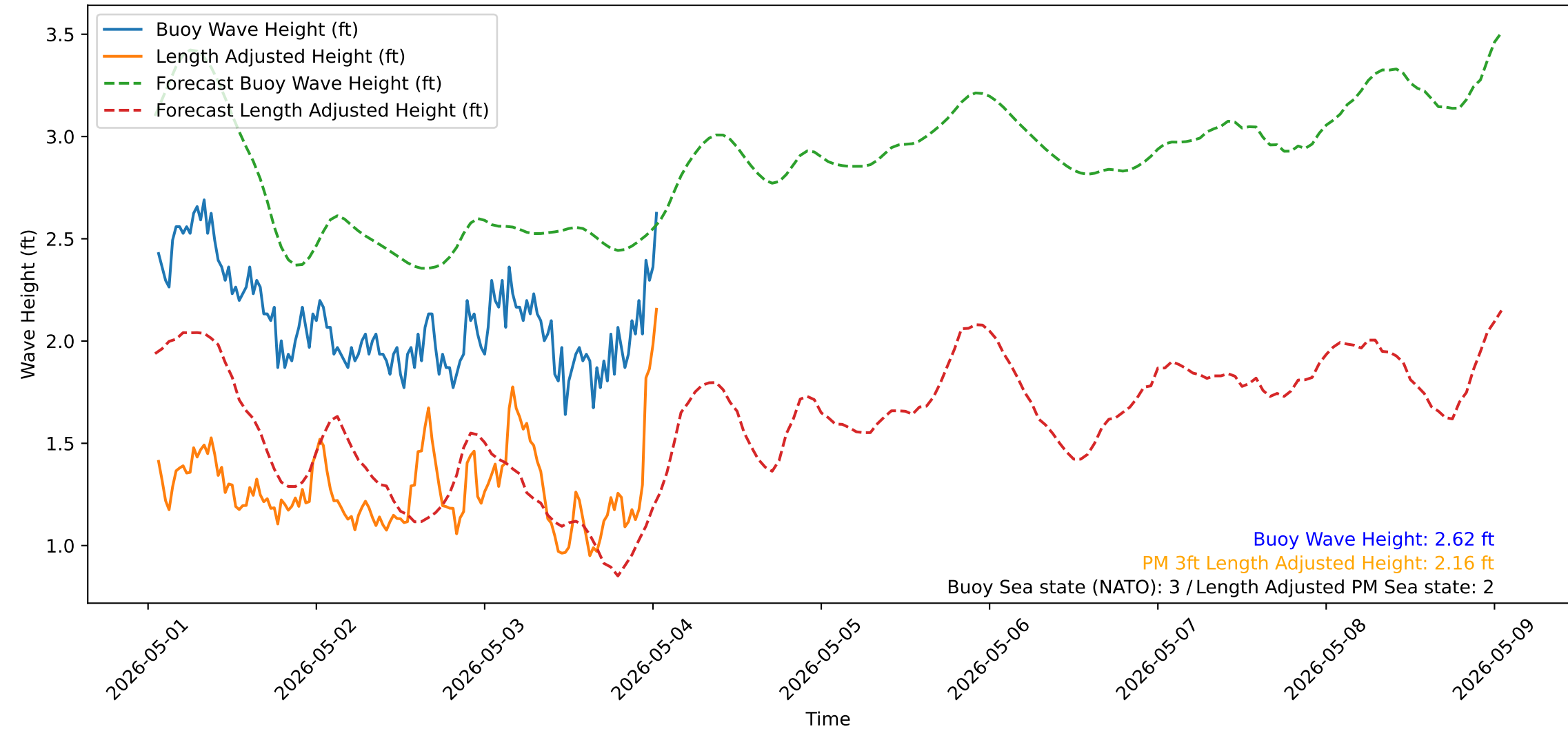
Wave Heights over Time for Oceanside Harbor at 2026-05-04 01:20:32
