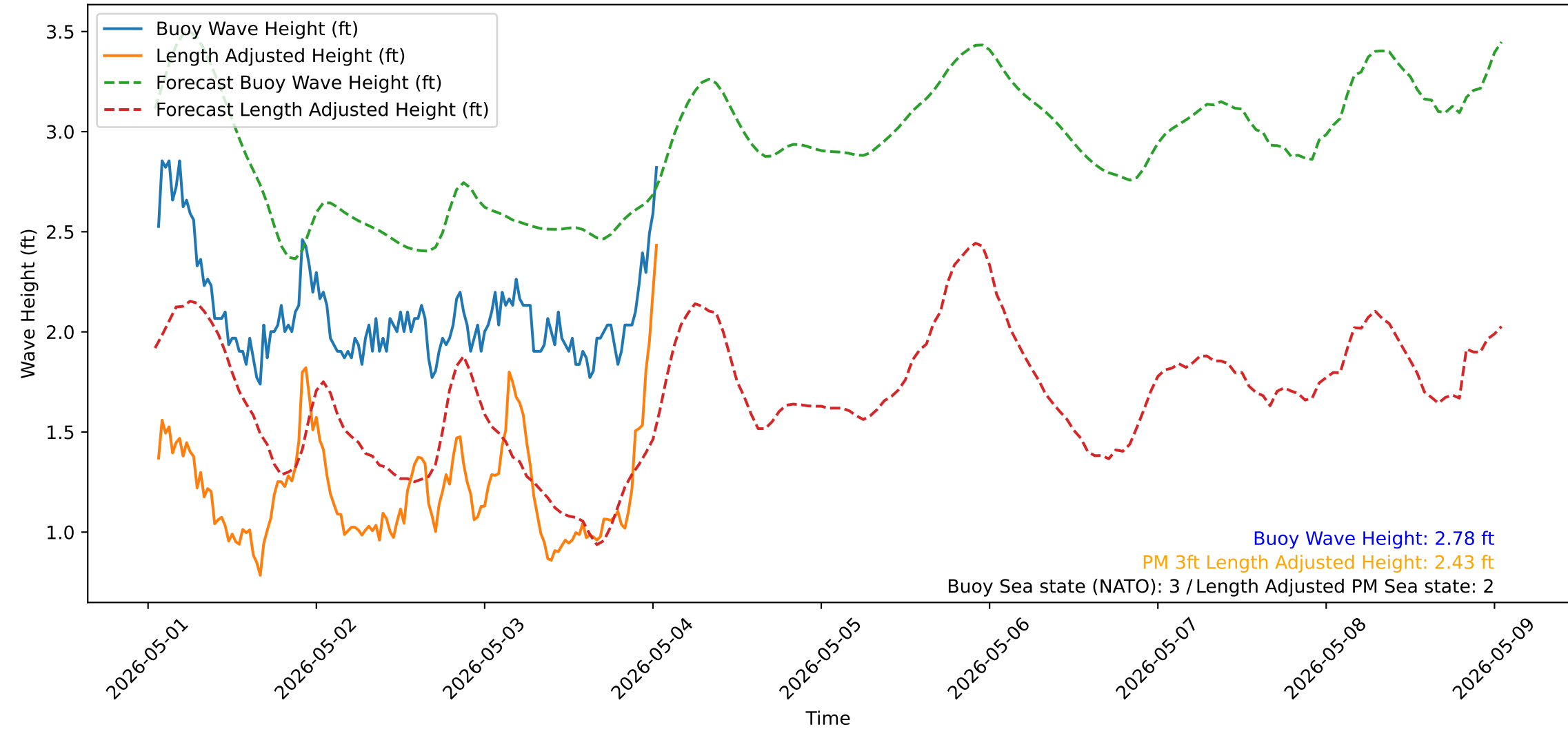
Wave Heights over Time for Green Beach at 2026-05-04 01:21:13
