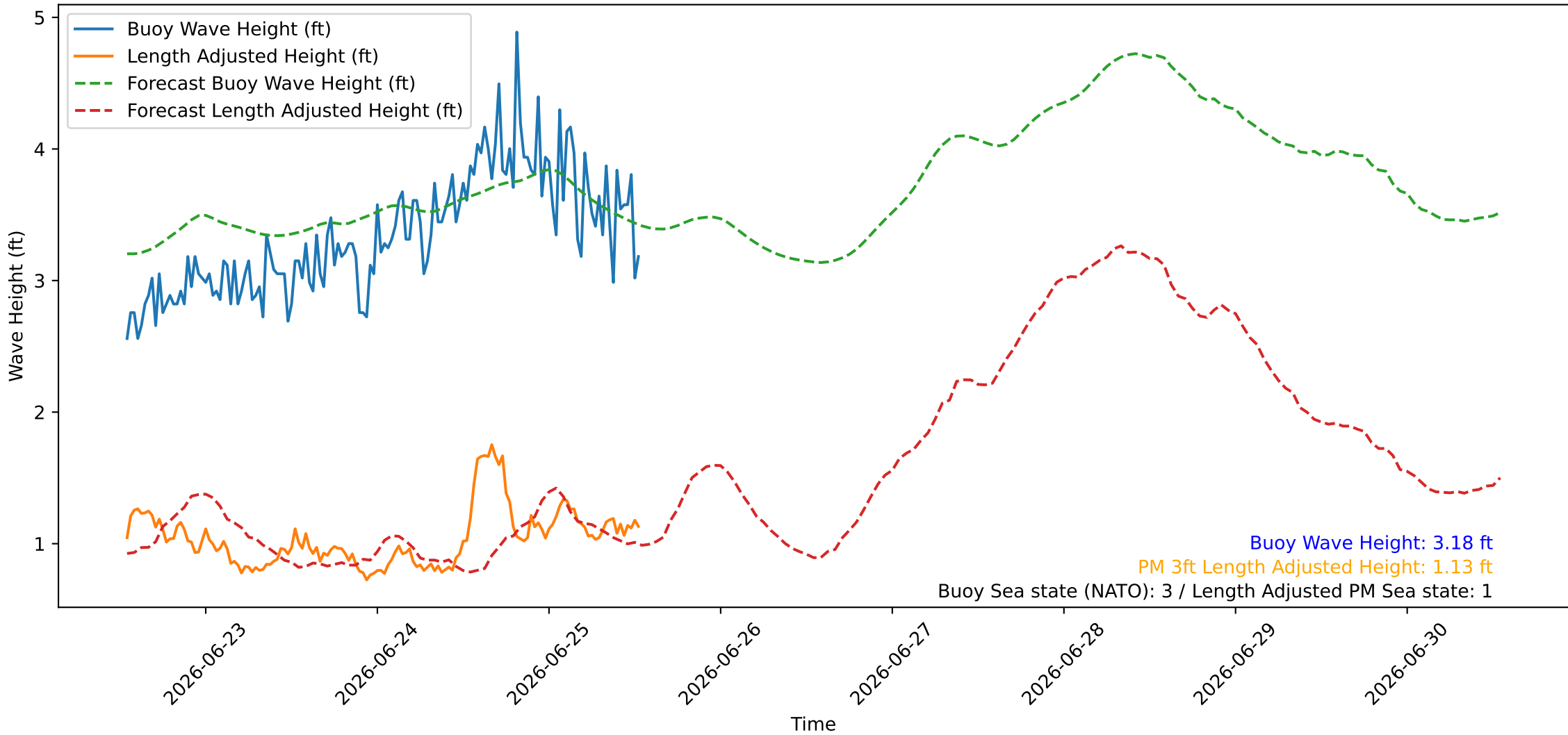
Wave Heights over Time for Oceanside Harbor at 2026-06-25 13:10:26
