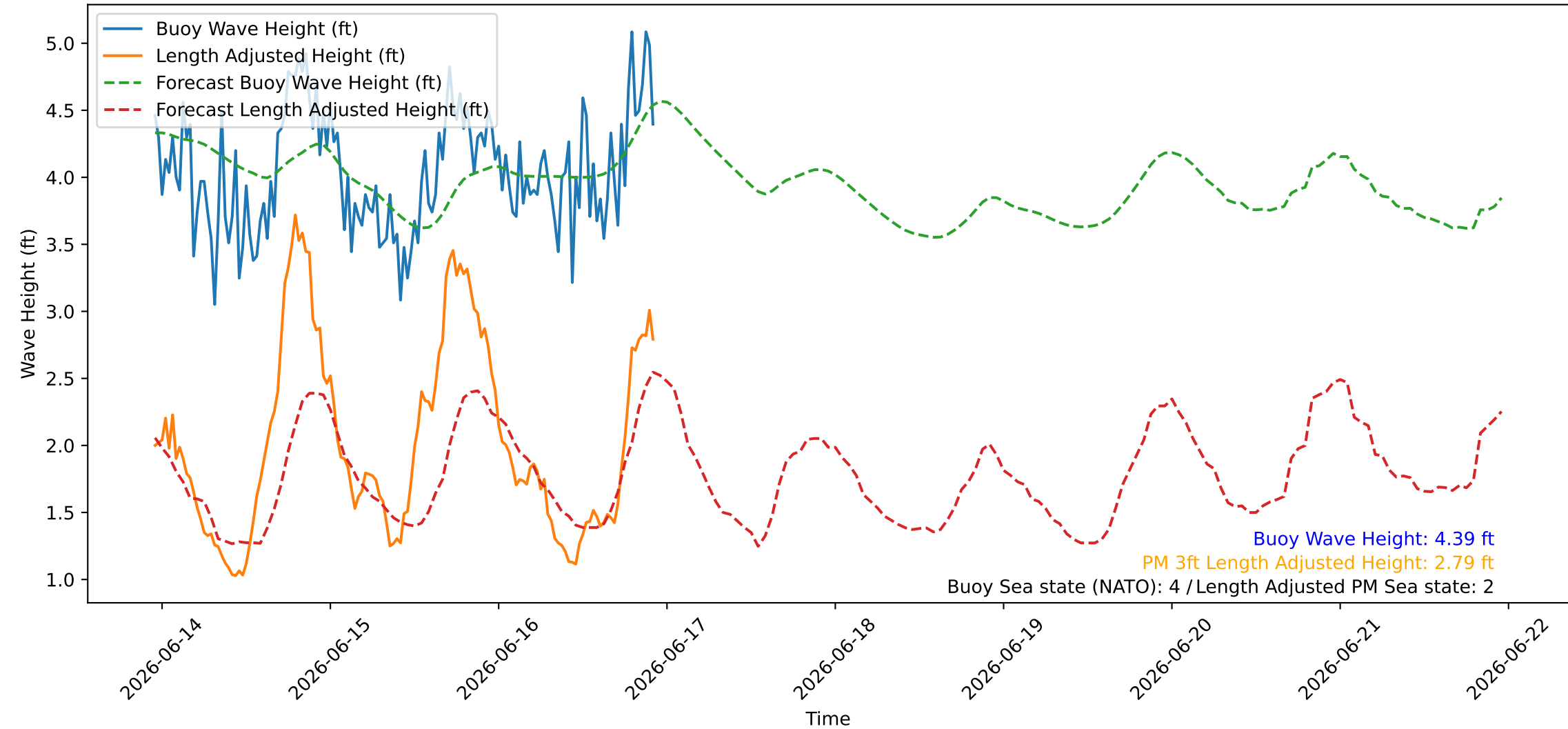
Wave Heights over Time for Green Beach at 2026-06-16 23:01:07
