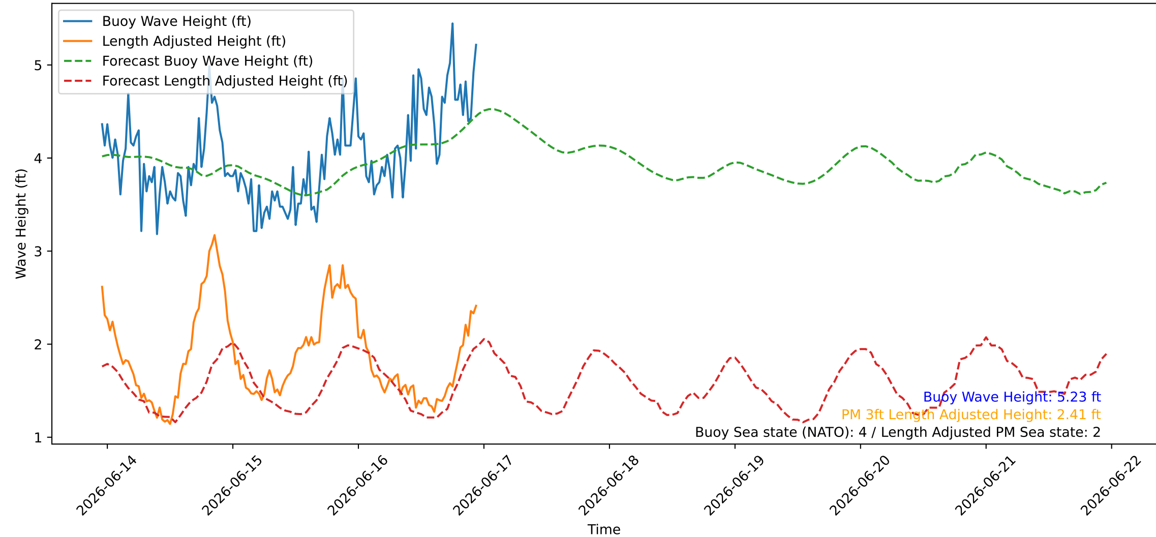
Wave Heights over Time for Oceanside Harbor at 2026-06-16 23:00:26
