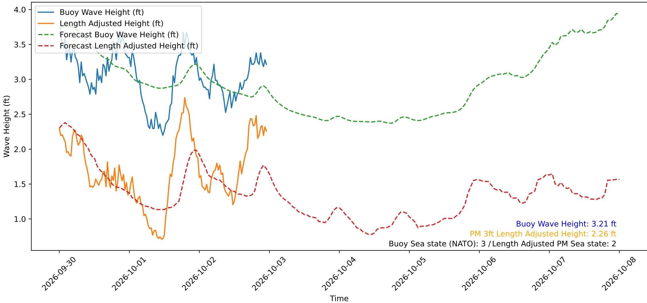
Wave Heights over Time for Green Beach at 2026-10-02 23:41:11
