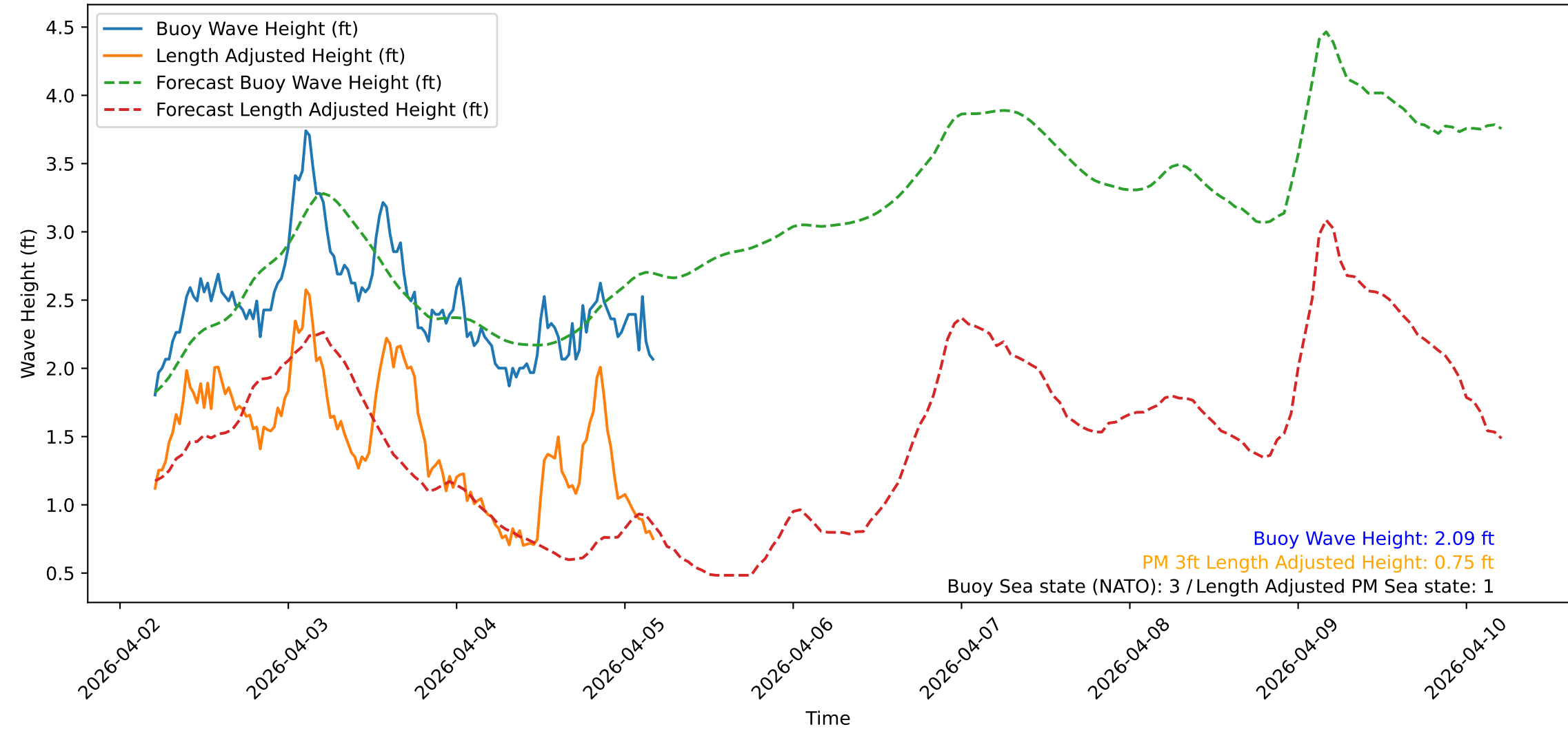
Wave Heights over Time for Red Beach at 2026-04-05 04:50:47
