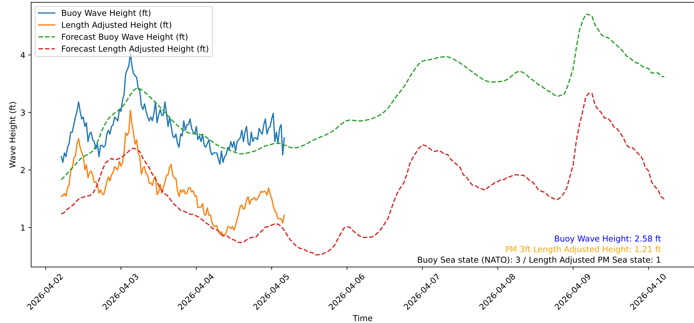
Wave Heights over Time for Oceanside Harbor at 2026-04-05 04:50:31
