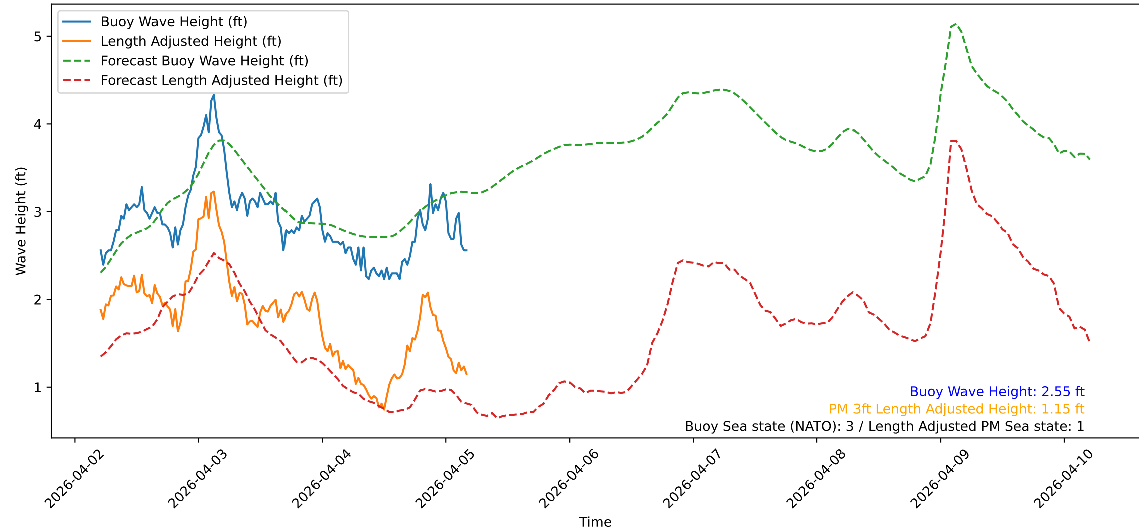
Wave Heights over Time for Green Beach at 2026-04-05 04:51:09
