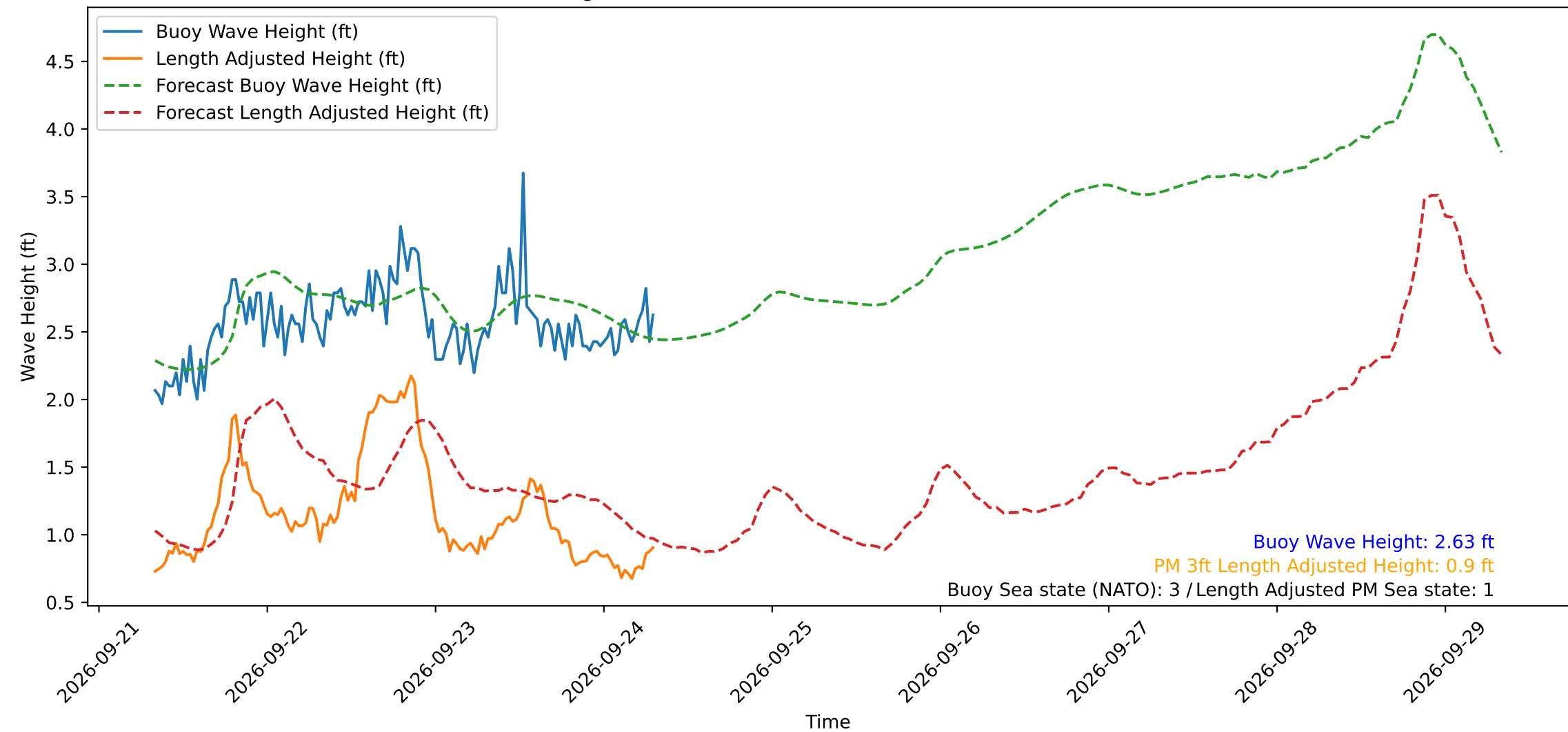
Wave Heights over Time for Red Beach at 2026-09-24 07:50:50
