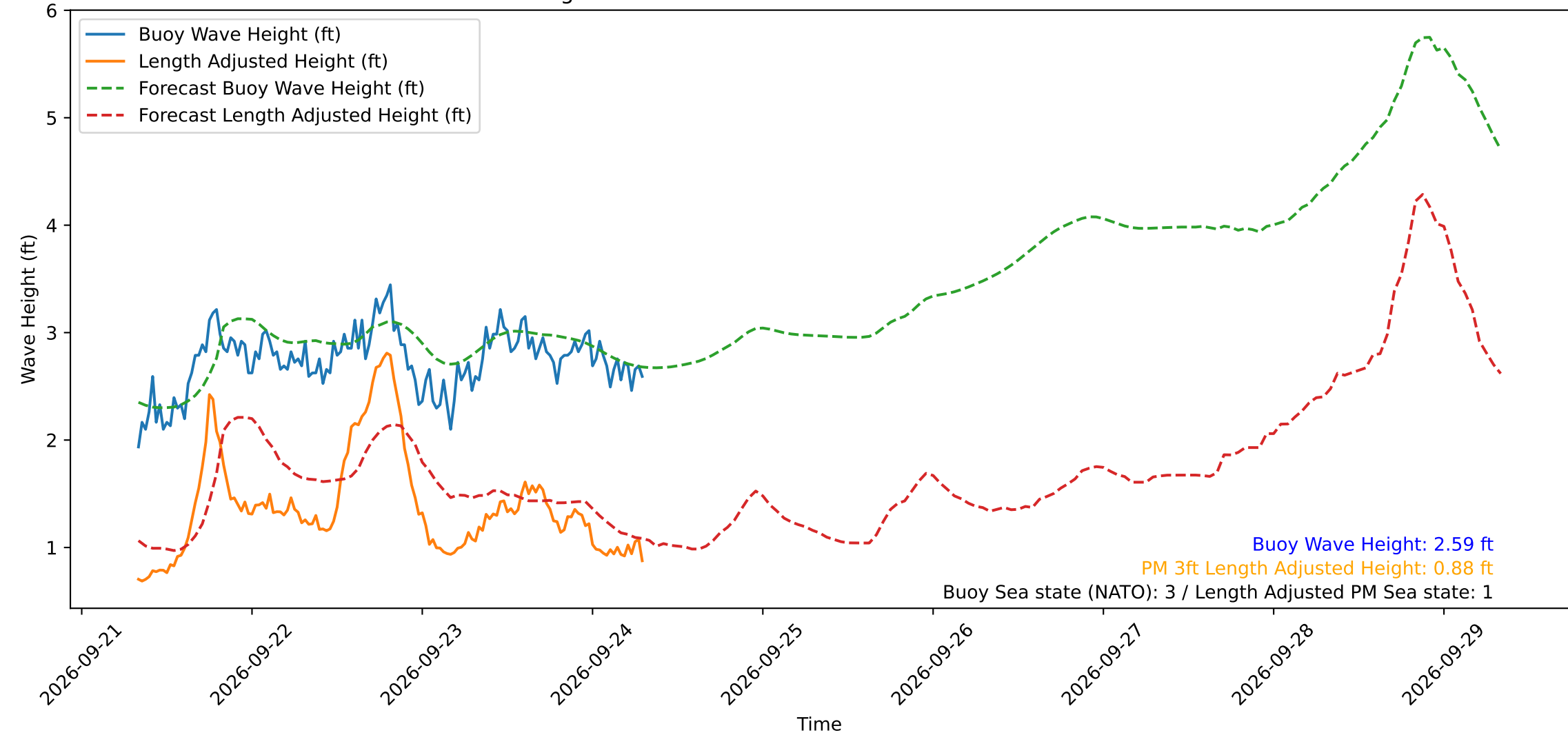
Wave Heights over Time for Green Beach at 2026-09-24 07:51:14
