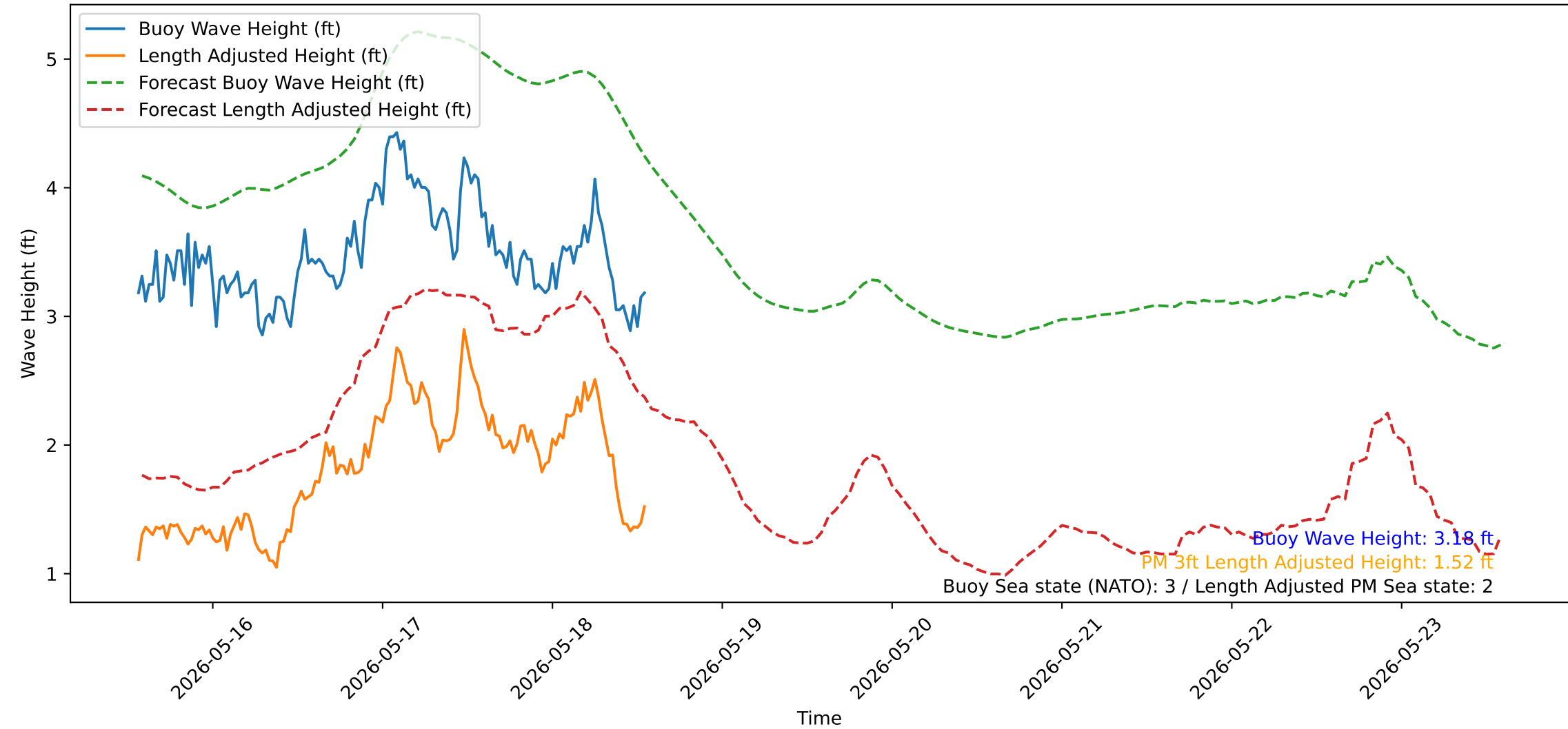
Wave Heights over Time for Green Beach at 2026-05-18 13:41:13
