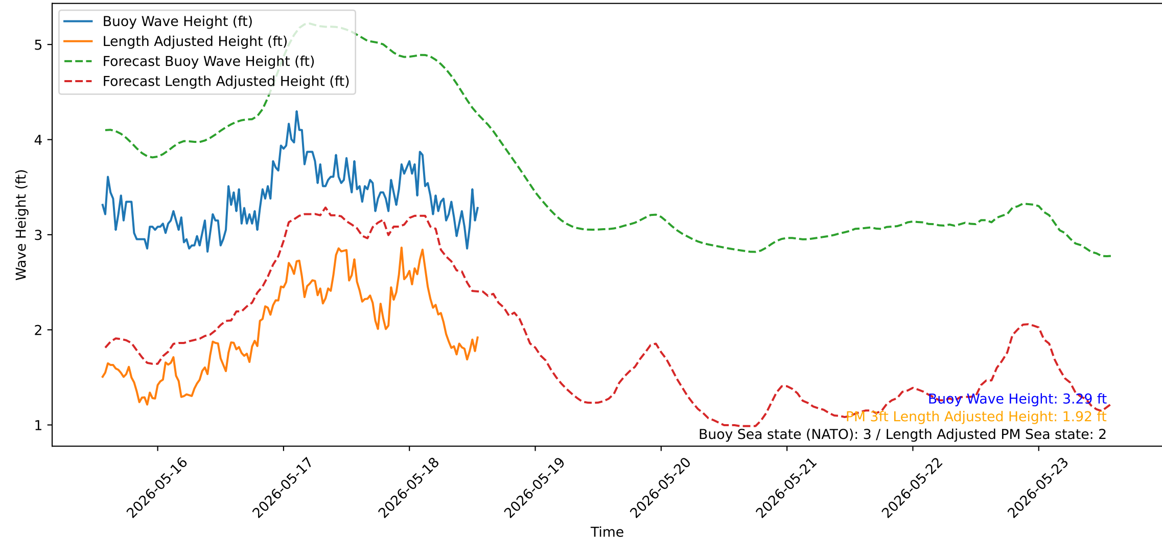
Wave Heights over Time for Oceanside Harbor at 2026-05-18 13:40:31
