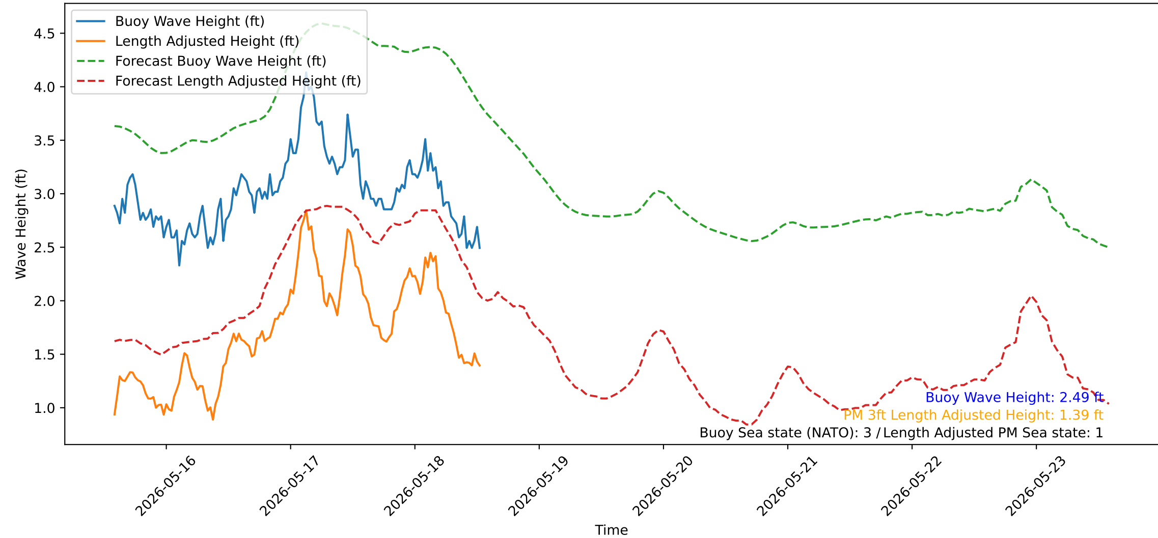
Wave Heights over Time for Red Beach at 2026-05-18 13:40:50
