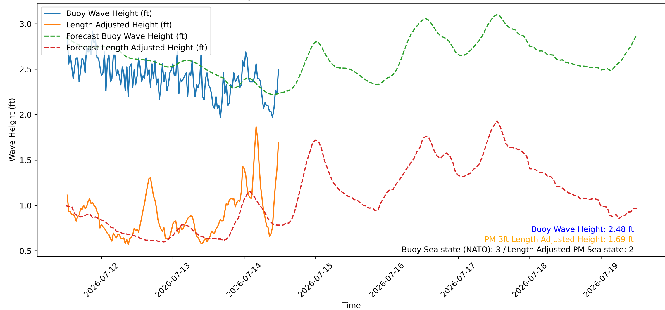
Wave Heights over Time for Red Beach at 2026-07-14 12:20:46
