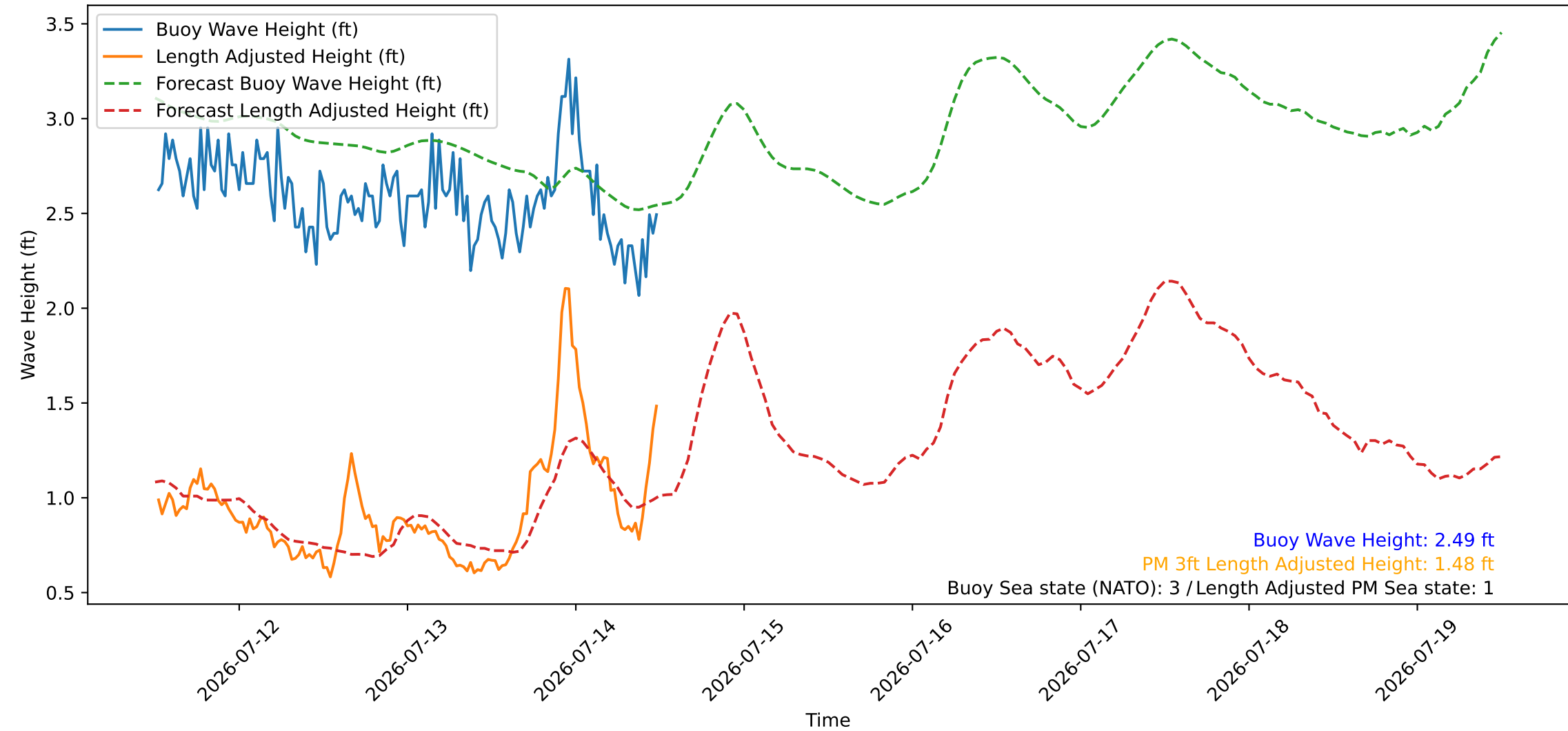
Wave Heights over Time for Green Beach at 2026-07-14 12:21:09
