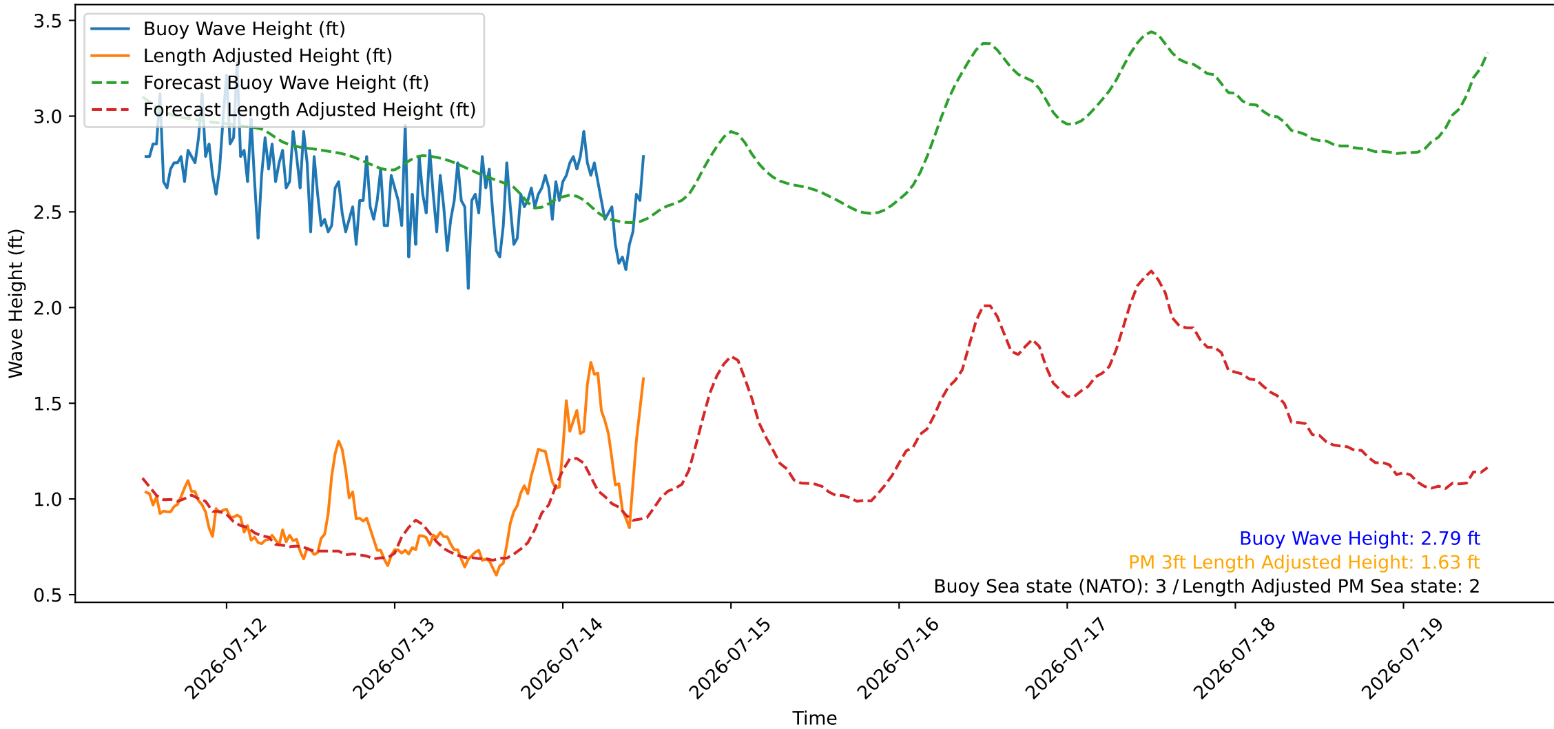
Wave Heights over Time for Oceanside Harbor at 2026-07-14 12:20:26
