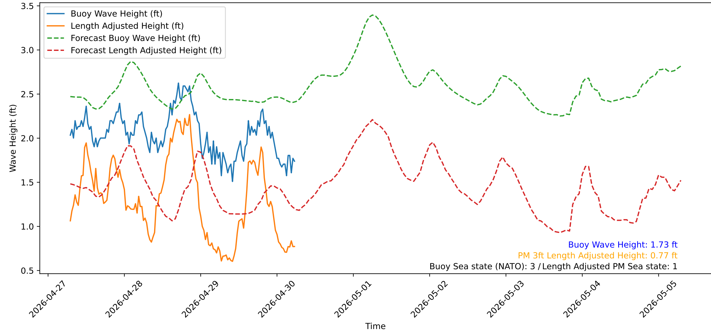
Wave Heights over Time for Red Beach at 2026-04-30 06:30:50
