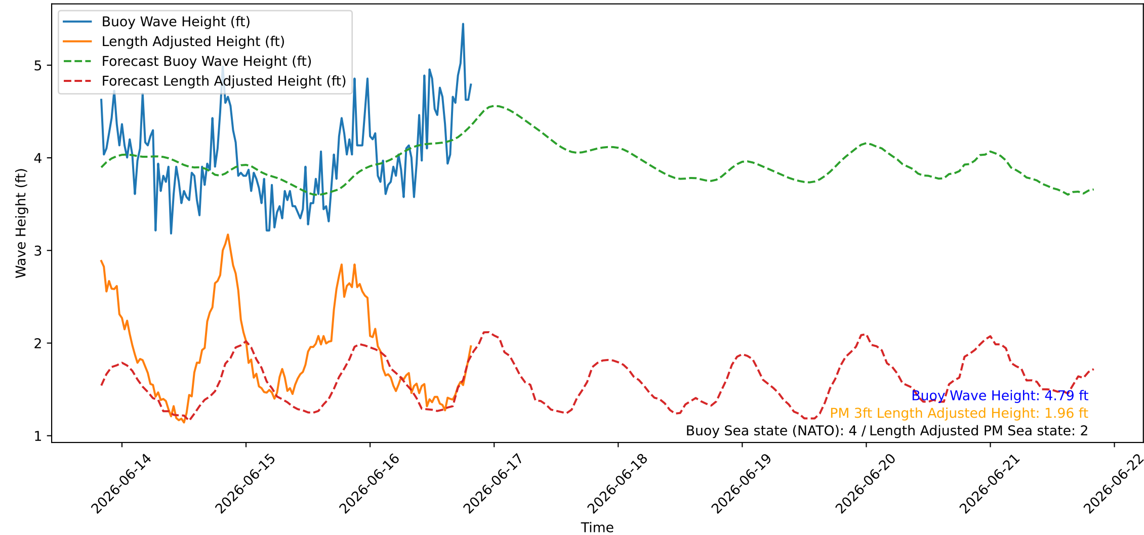
Wave Heights over Time for Oceanside Harbor at 2026-06-16 20:10:26
