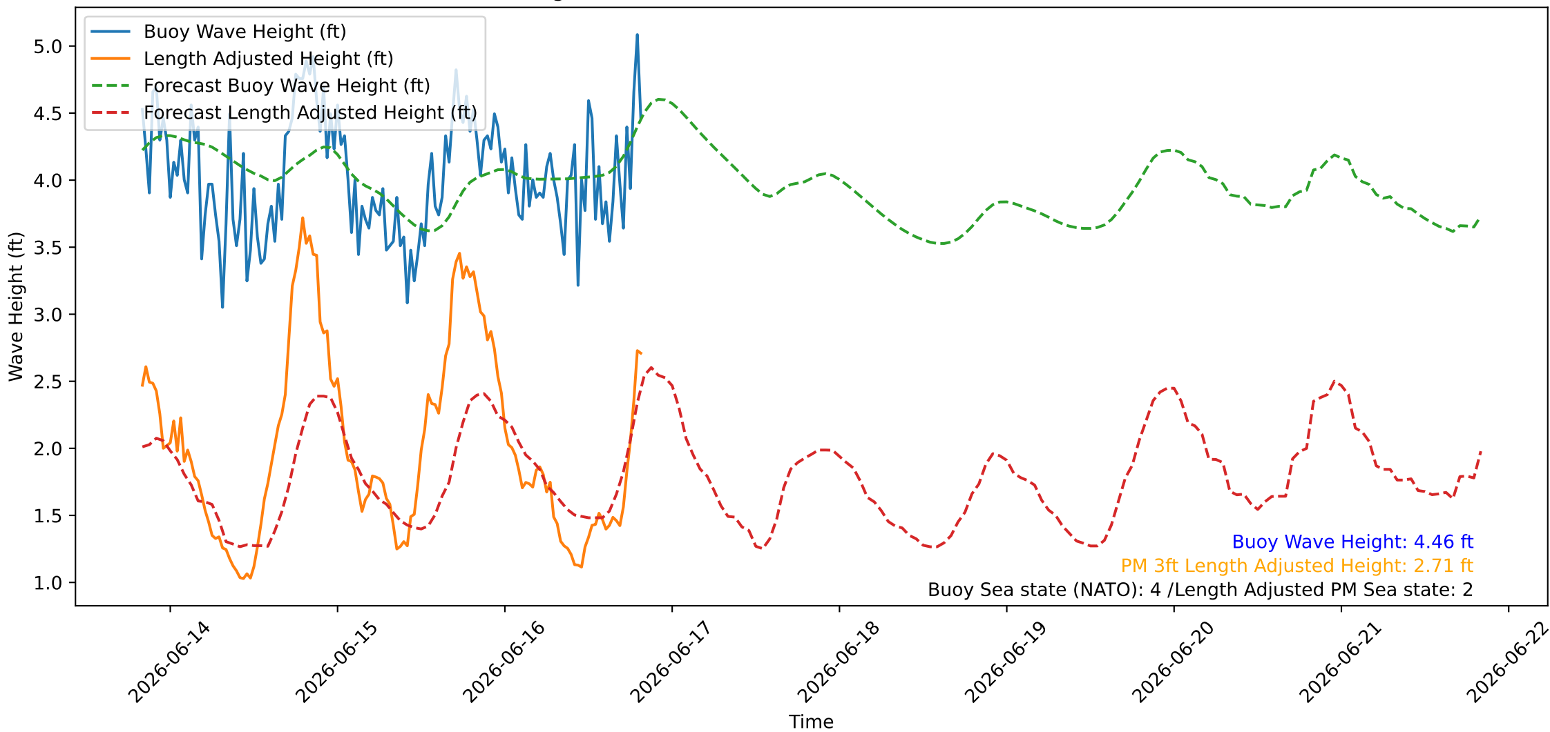
Wave Heights over Time for Green Beach at 2026-06-16 20:11:07
