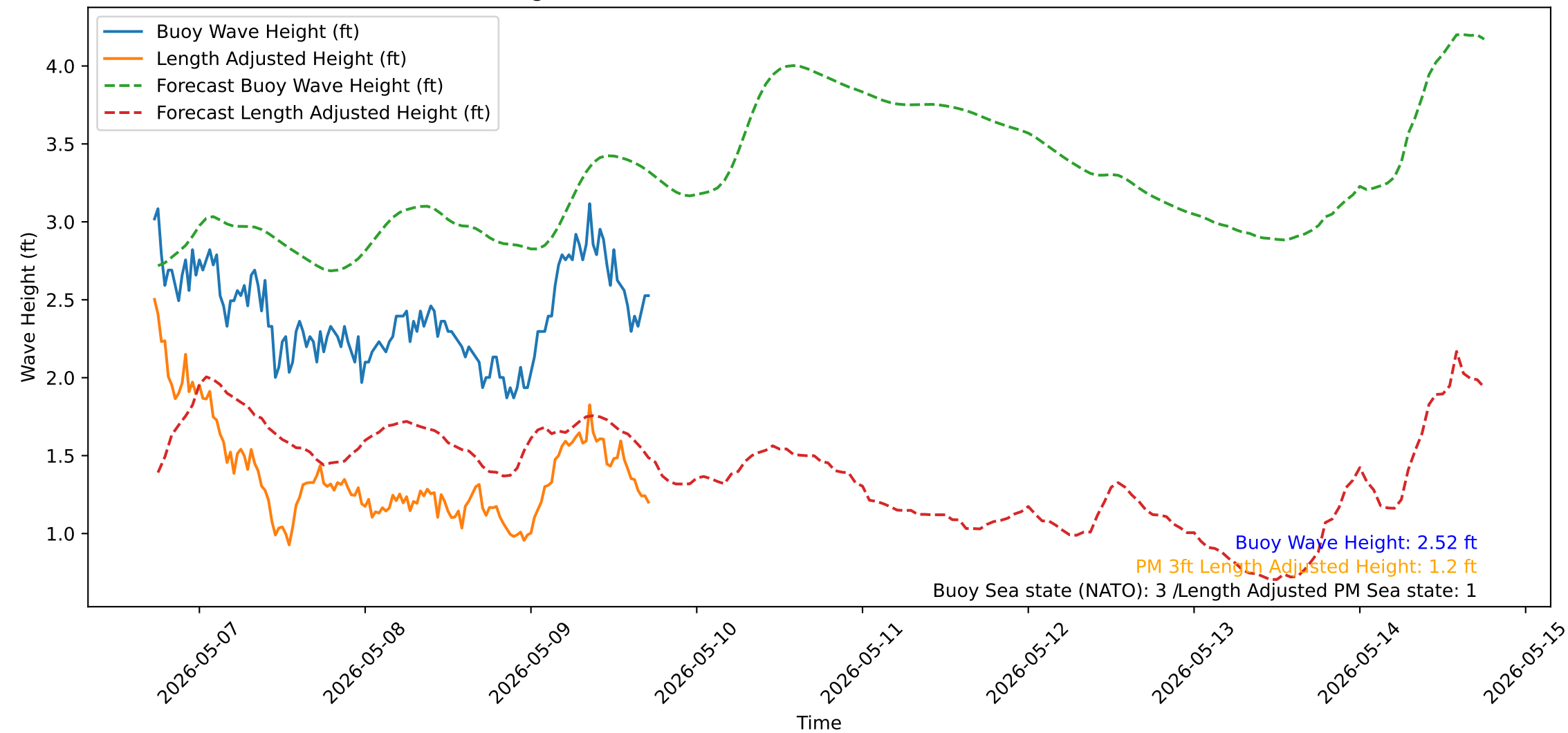
Wave Heights over Time for Oceanside Harbor at 2026-05-09 17:30:31
