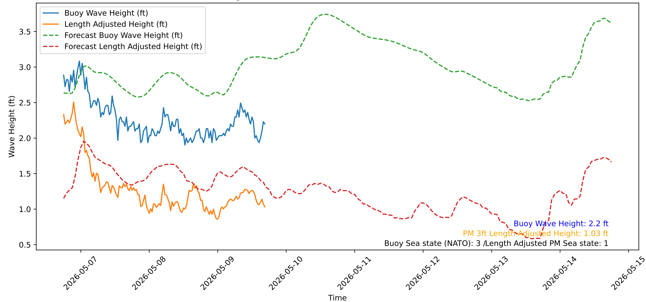
Wave Heights over Time for Red Beach at 2026-05-09 17:30:50
