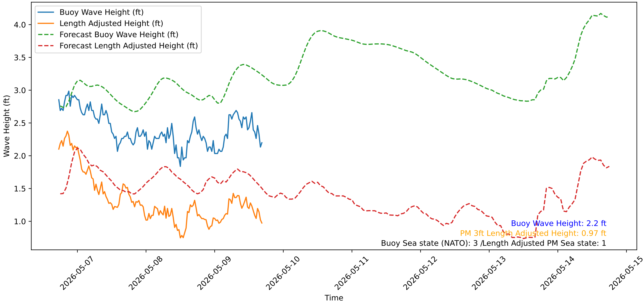
Wave Heights over Time for Green Beach at 2026-05-09 17:31:13
