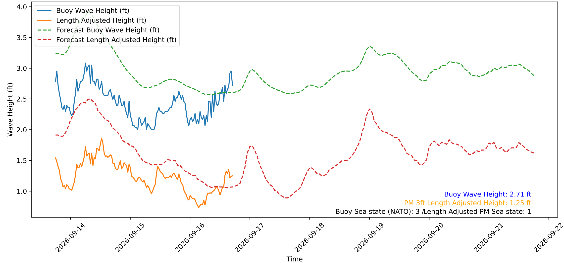
Wave Heights over Time for Red Beach at 2026-09-16 17:50:50
