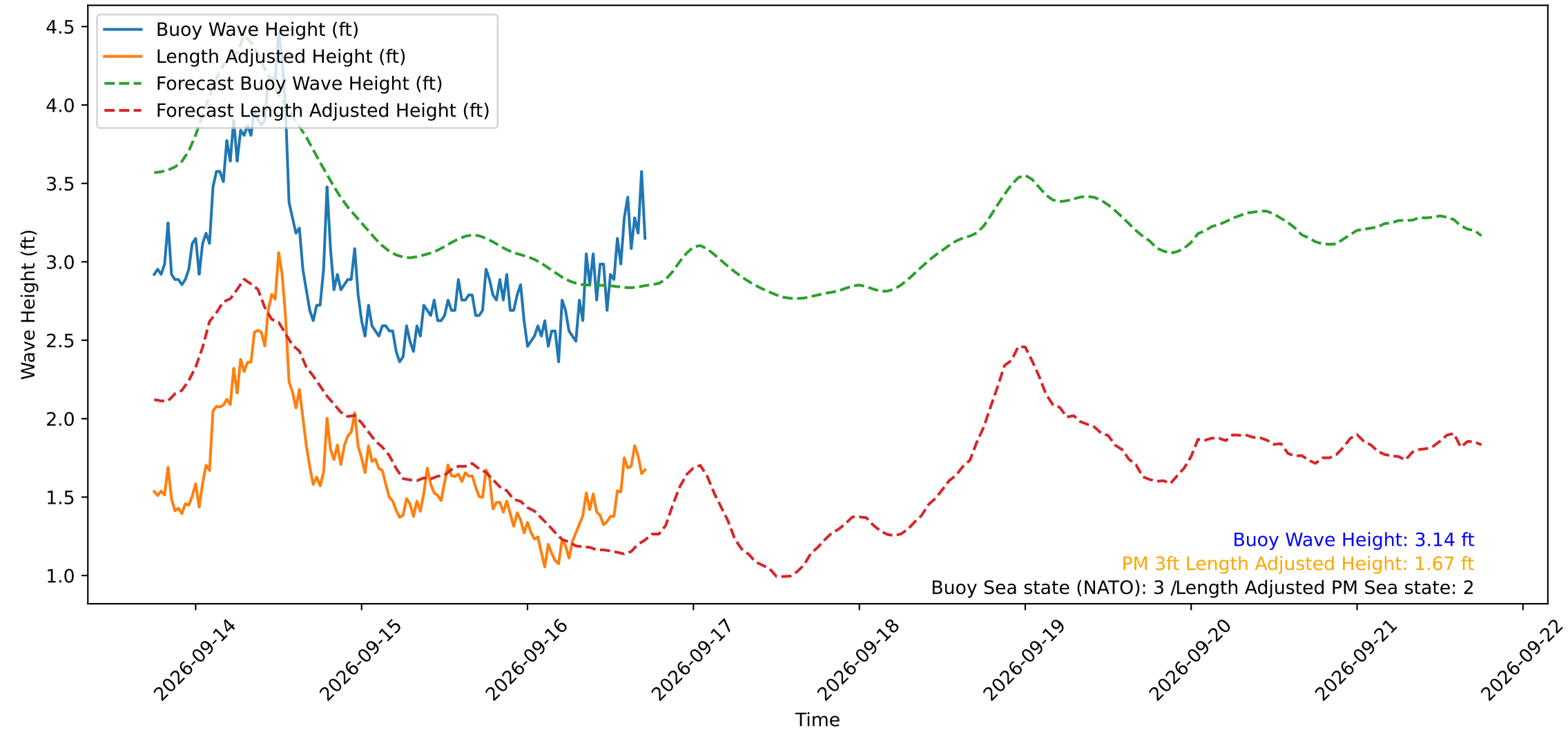
Wave Heights over Time for Oceanside Harbor at 2026-09-16 17:50:29
