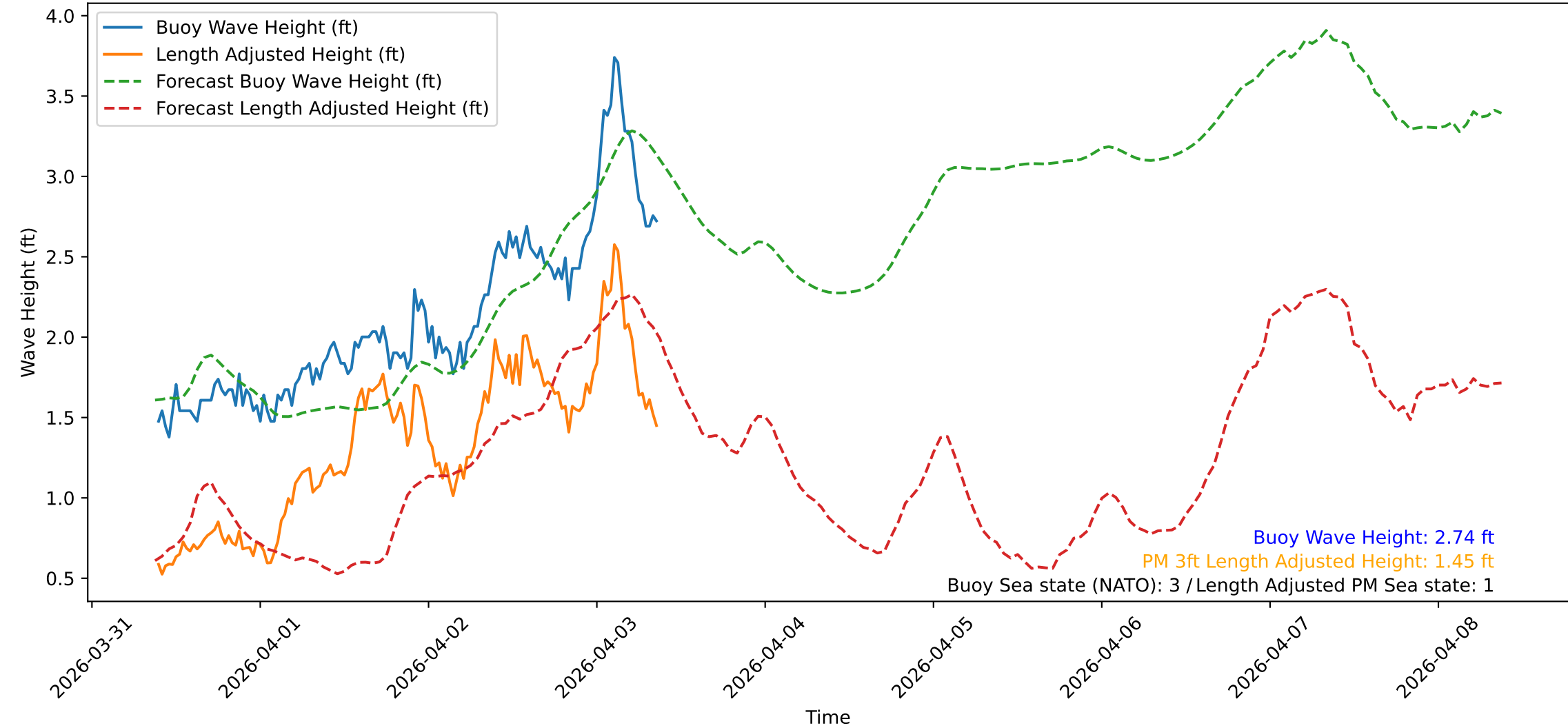
Wave Heights over Time for Red Beach at 2026-04-03 09:20:47
