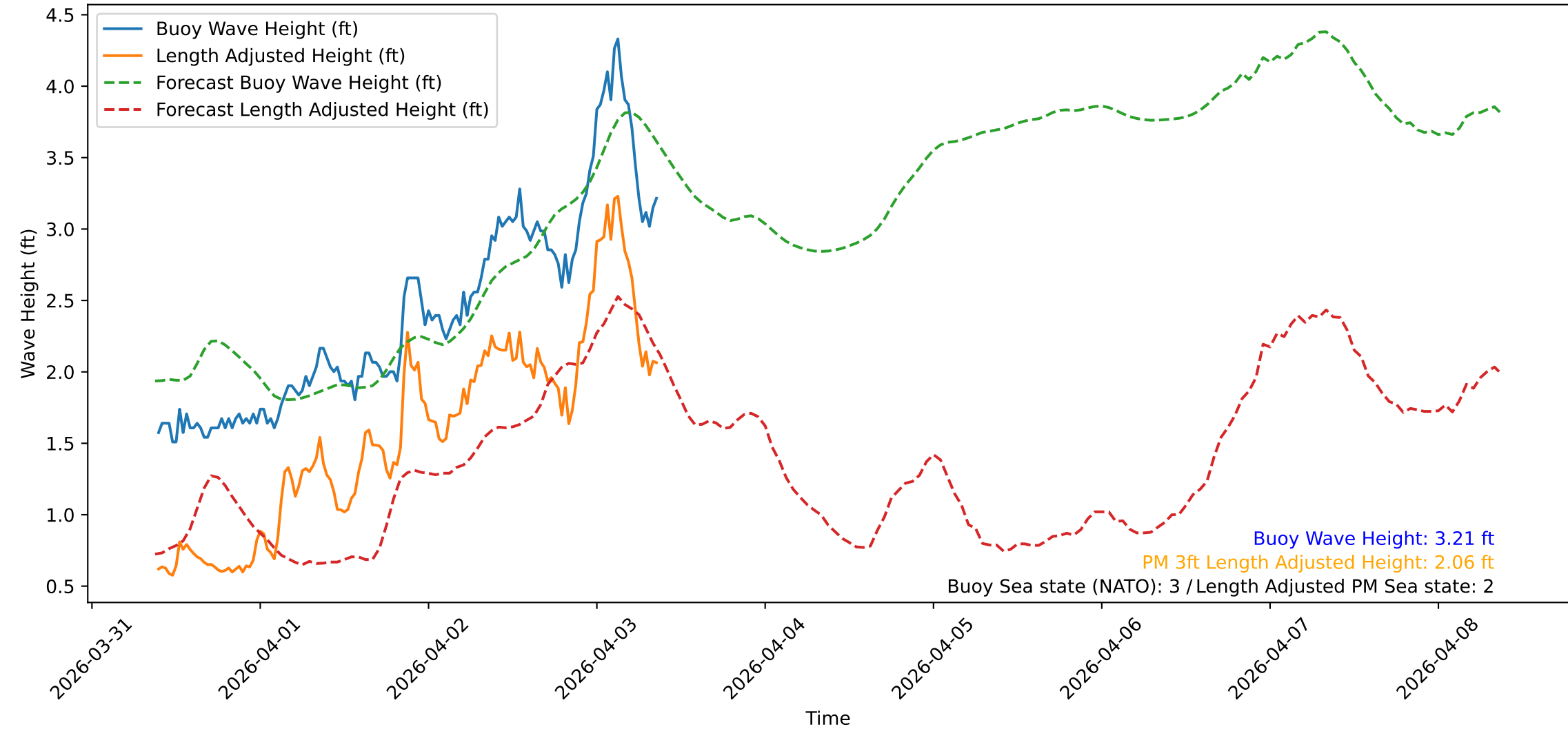
Wave Heights over Time for Green Beach at 2026-04-03 09:21:10
