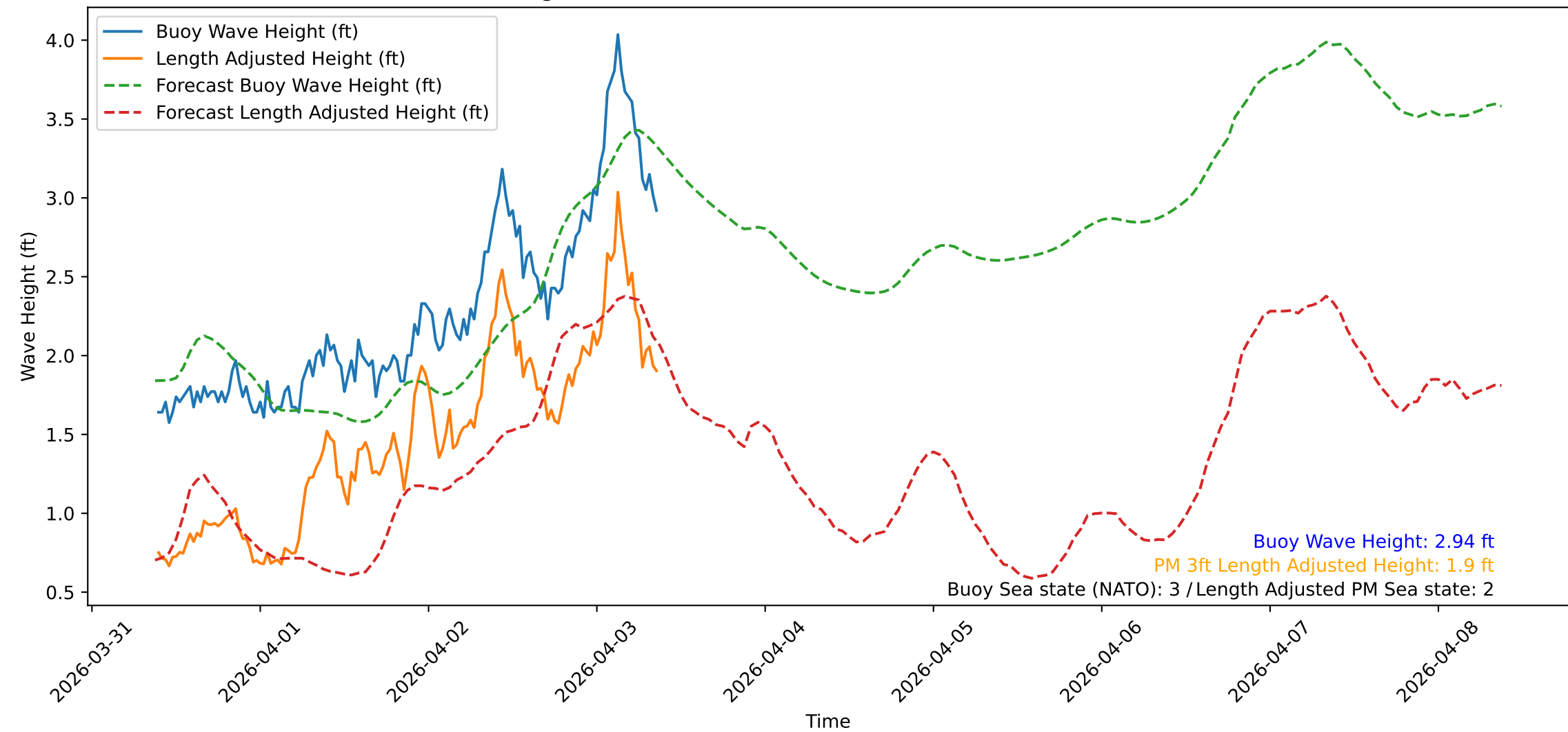
Wave Heights over Time for Oceanside Harbor at 2026-04-03 09:20:31
