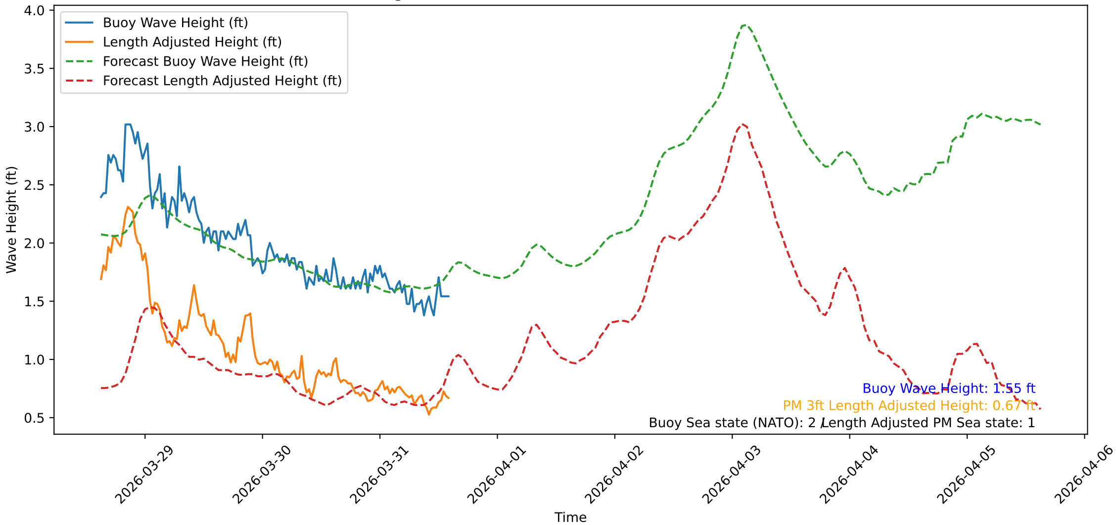
Wave Heights over Time for Red Beach at 2026-03-31 14:50:47
