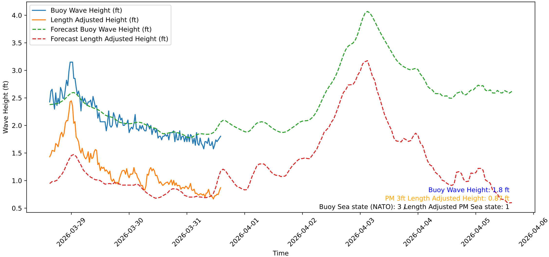
Wave Heights over Time for Oceanside Harbor at 2026-03-31 14:50:31
