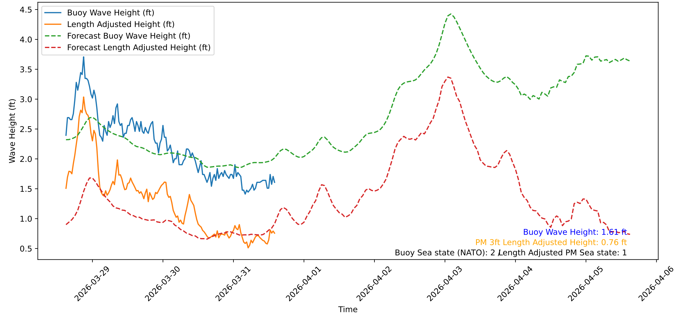
Wave Heights over Time for Green Beach at 2026-03-31 14:51:10
