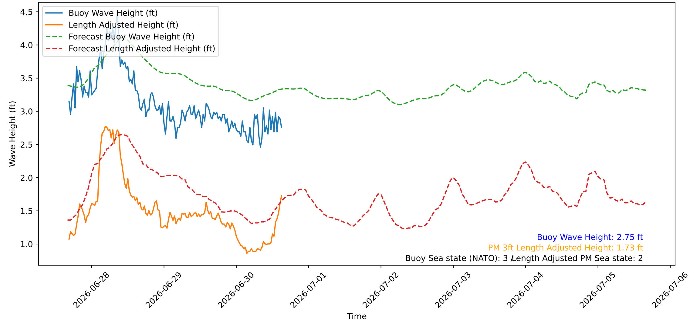
Wave Heights over Time for Red Beach at 2026-06-30 16:10:45
