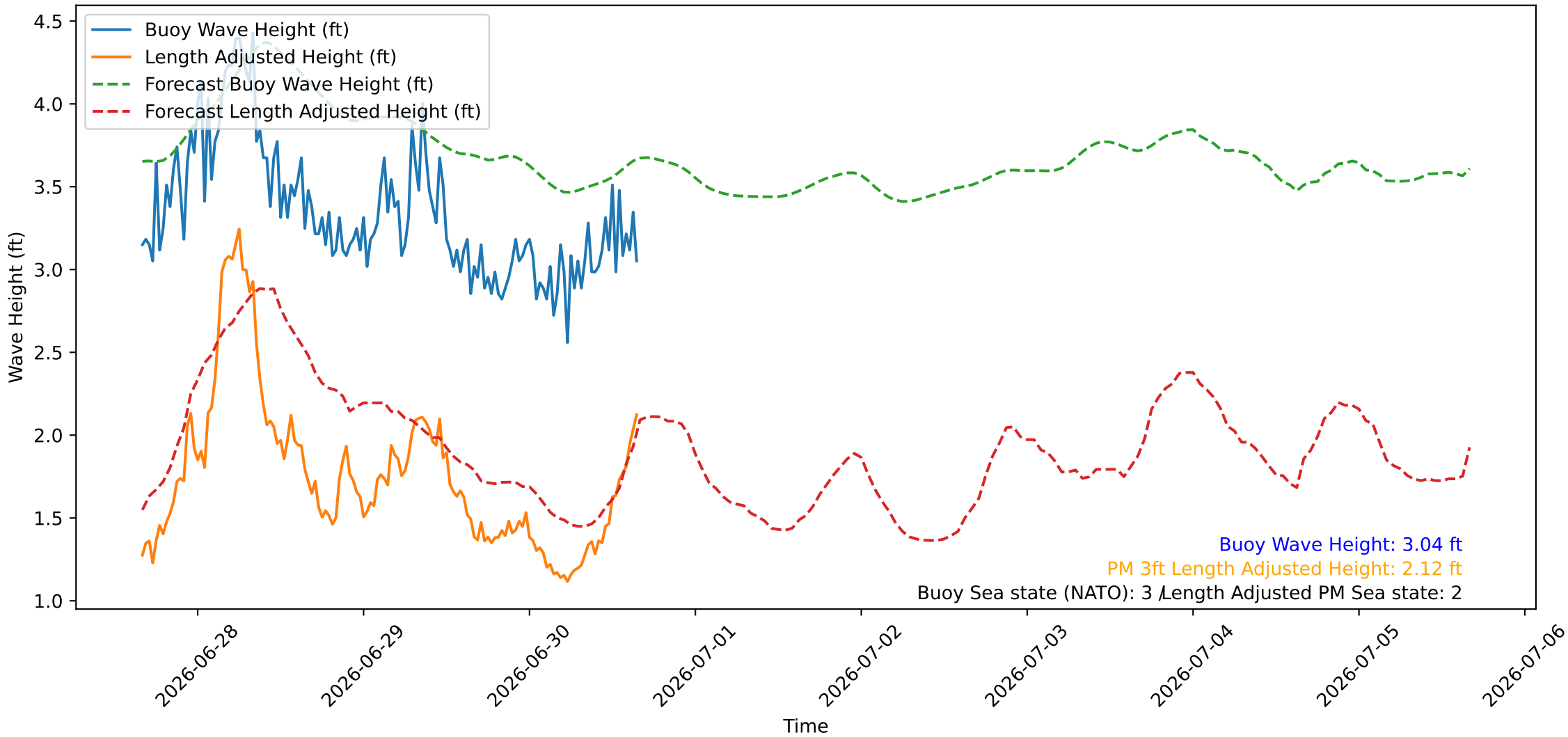
Wave Heights over Time for Oceanside Harbor at 2026-06-30 16:10:26
