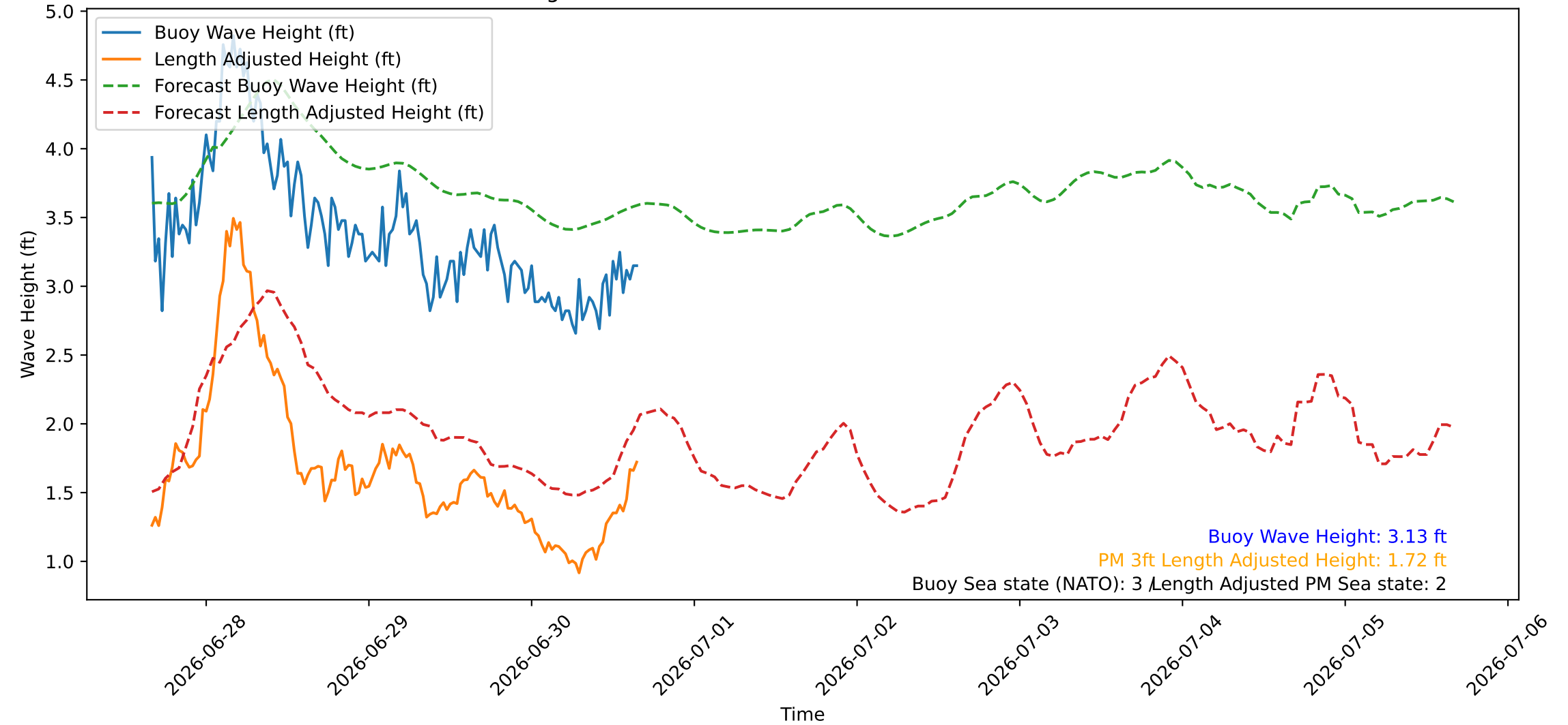
Wave Heights over Time for Green Beach at 2026-06-30 16:11:07
