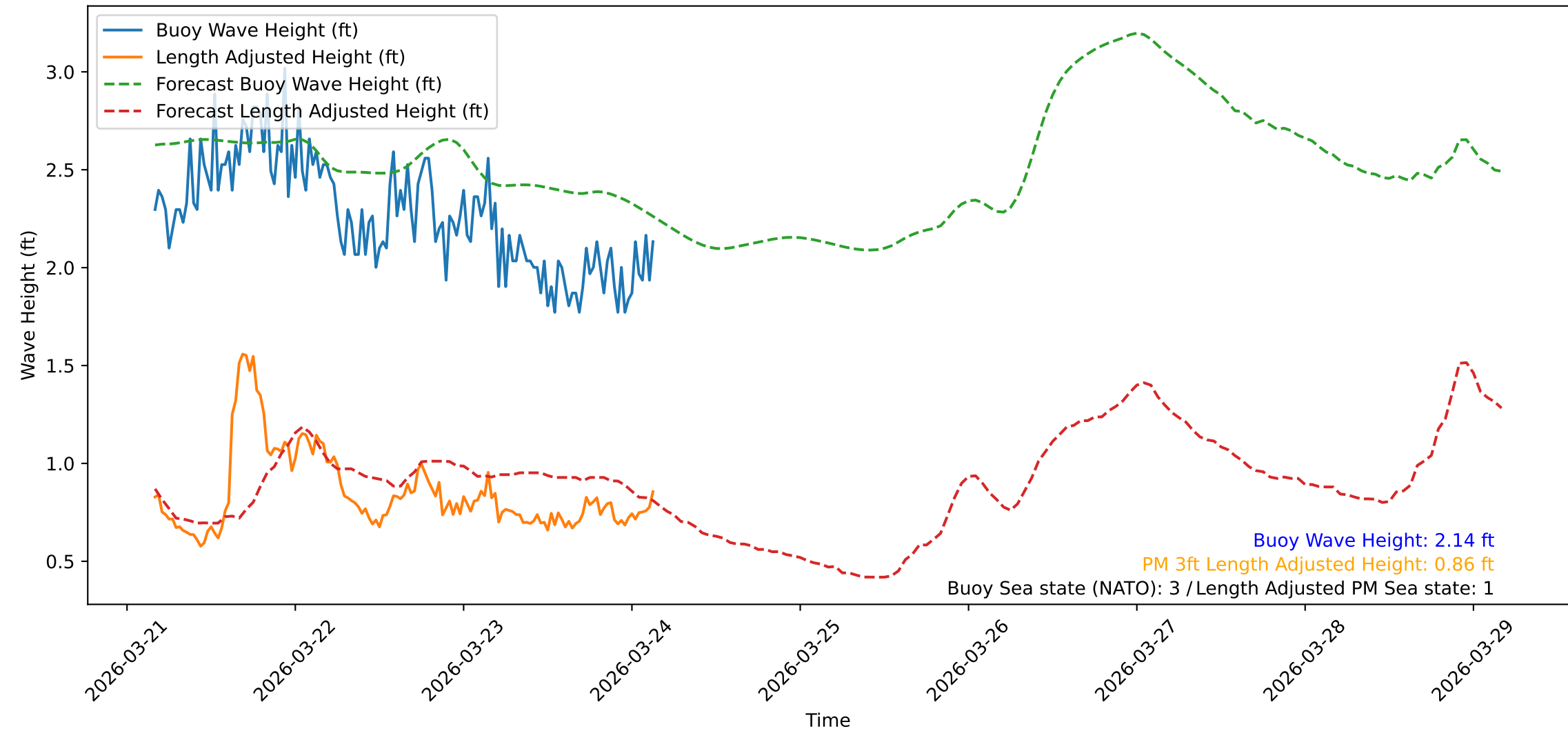
Wave Heights over Time for Oceanside Harbor at 2026-03-24 03:50:31
