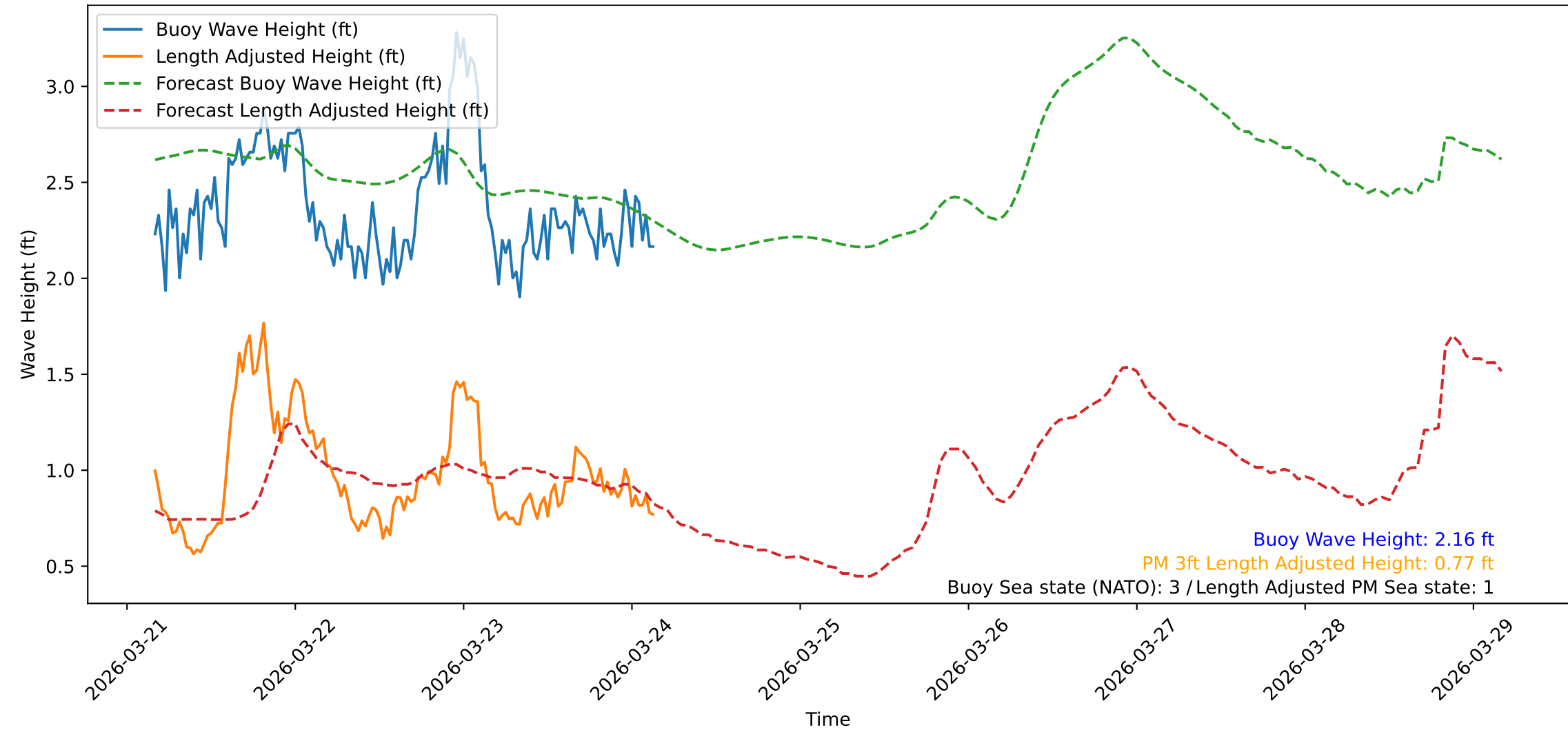
Wave Heights over Time for Green Beach at 2026-03-24 03:51:09
