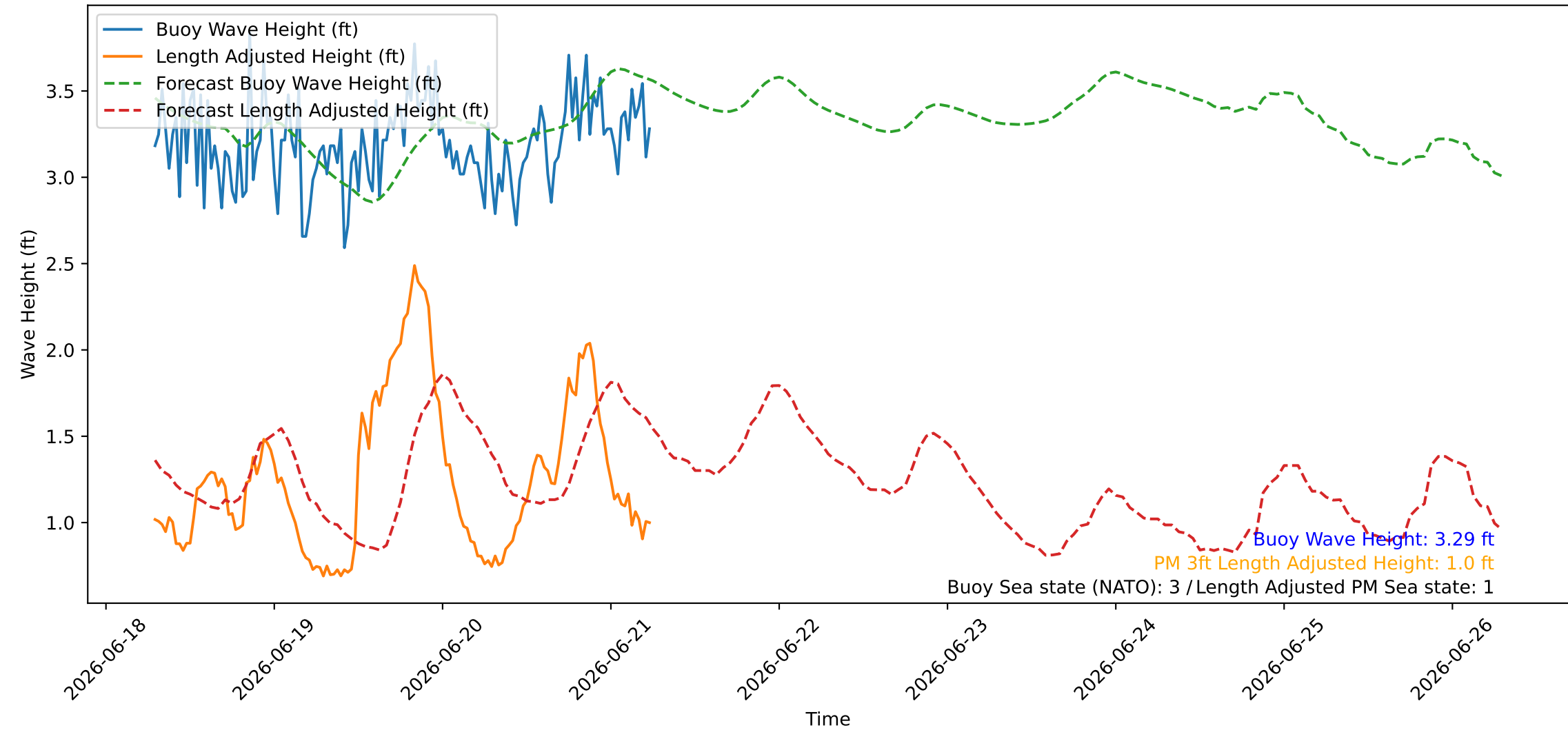
Wave Heights over Time for Red Beach at 2026-06-21 06:30:45
