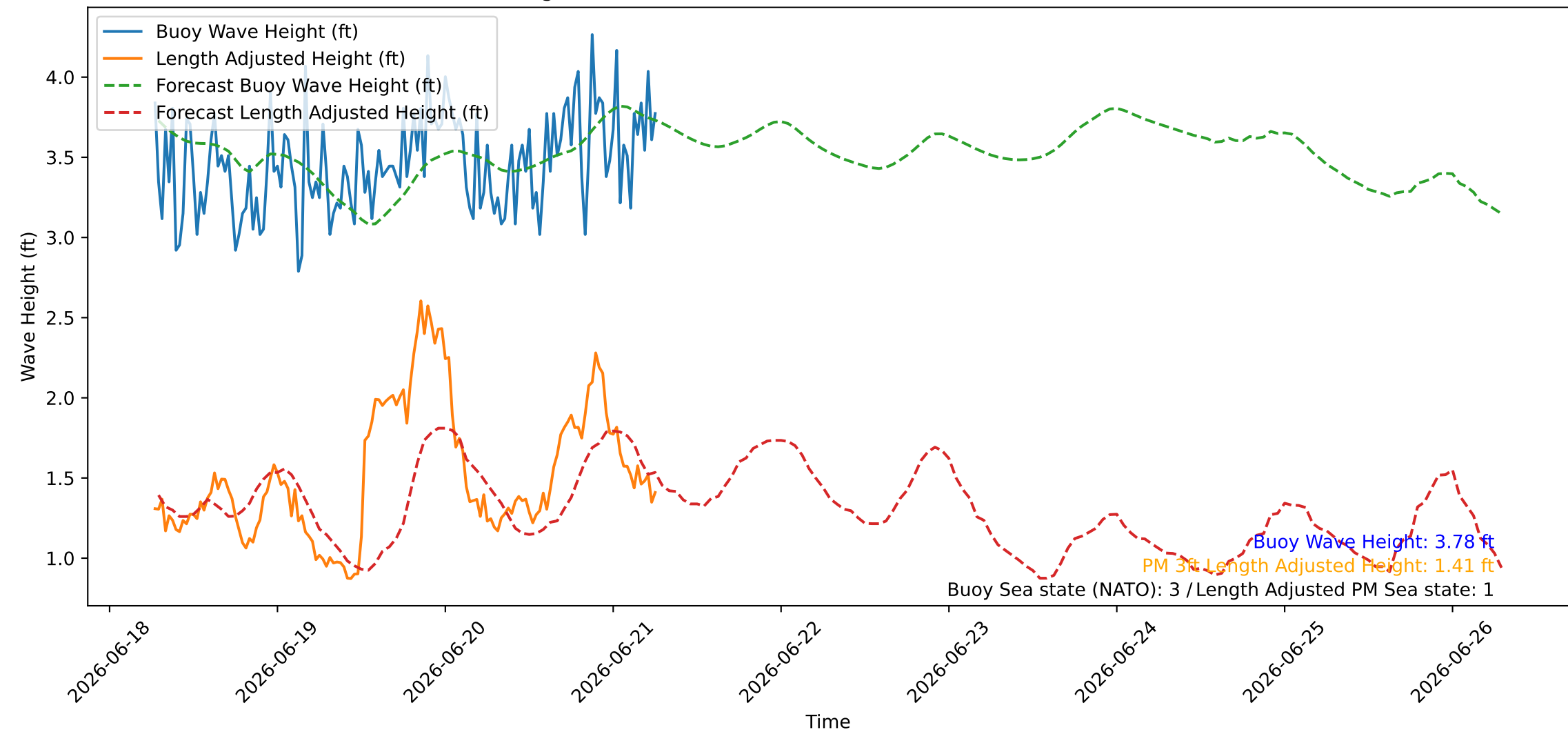
Wave Heights over Time for Oceanside Harbor at 2026-06-21 06:30:26
