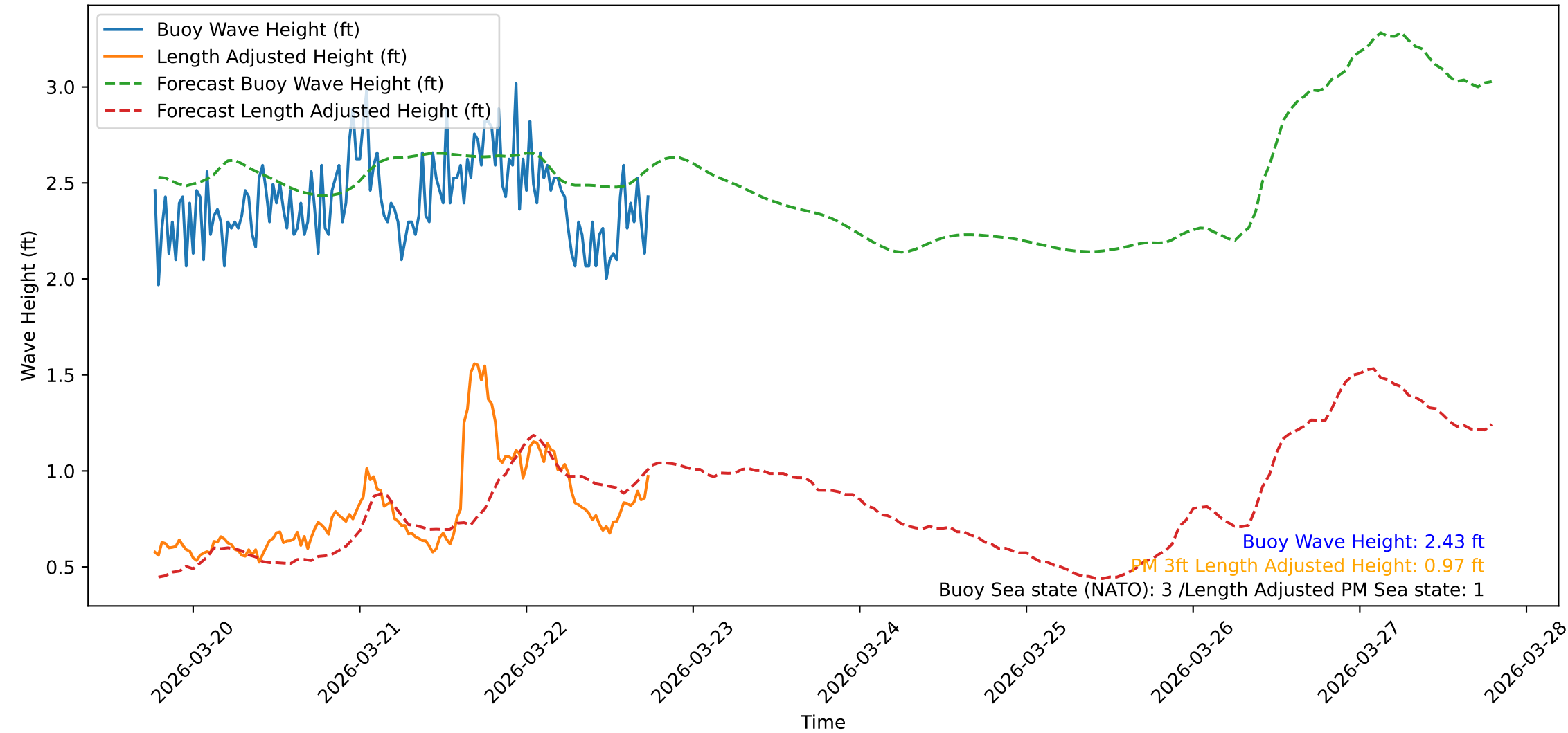
Wave Heights over Time for Oceanside Harbor at 2026-03-22 18:30:31
