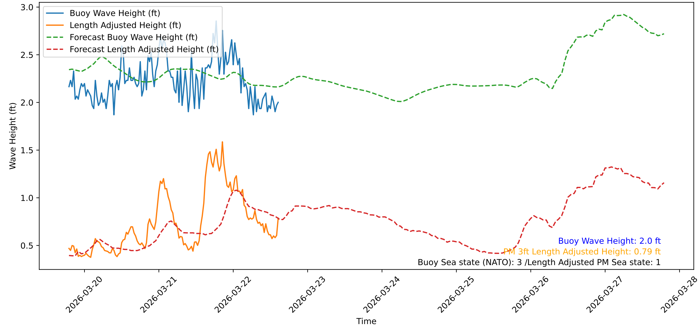
Wave Heights over Time for Red Beach at 2026-03-22 18:30:48
