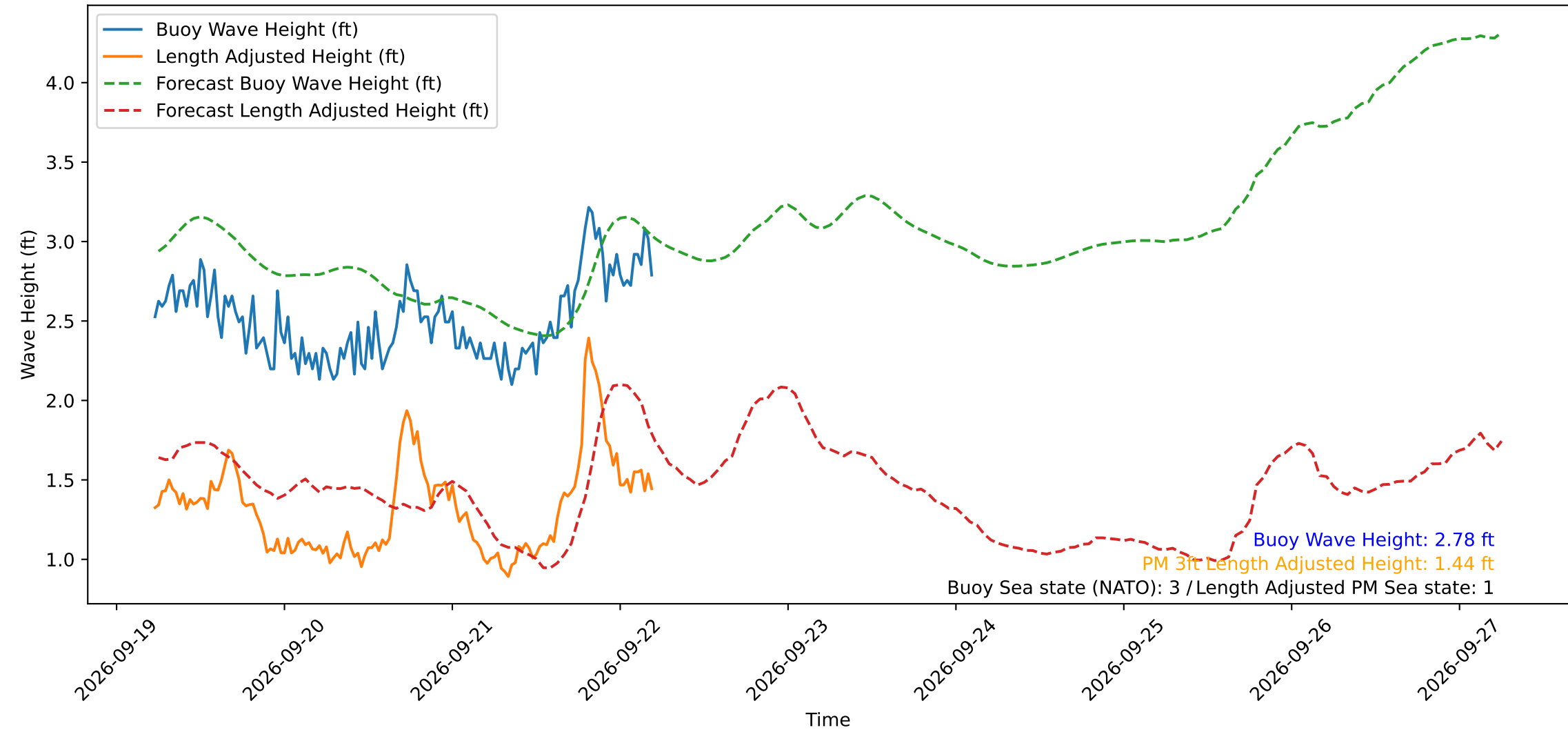
Wave Heights over Time for Oceanside Harbor at 2026-09-22 05:30:29
