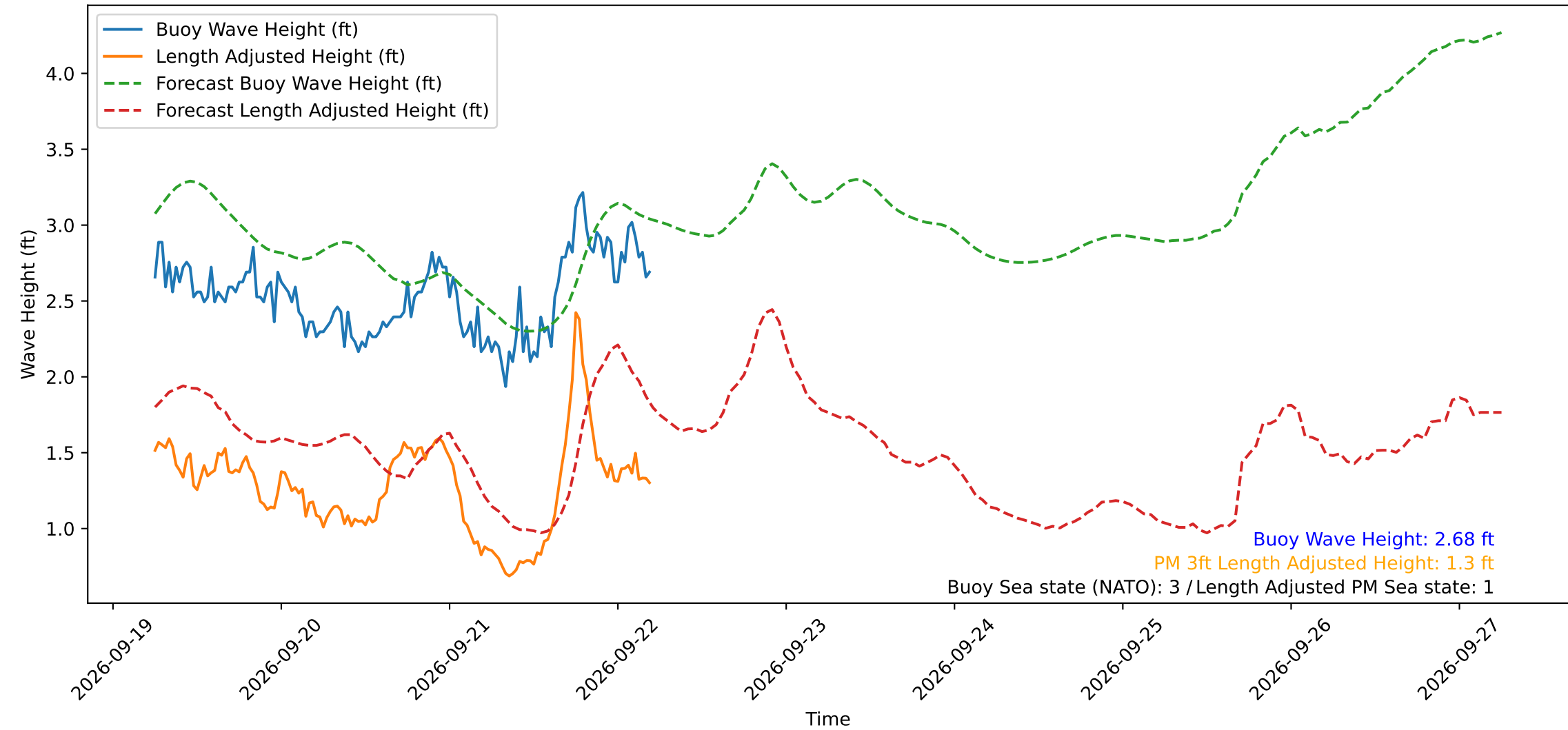
Wave Heights over Time for Green Beach at 2026-09-22 05:31:11
