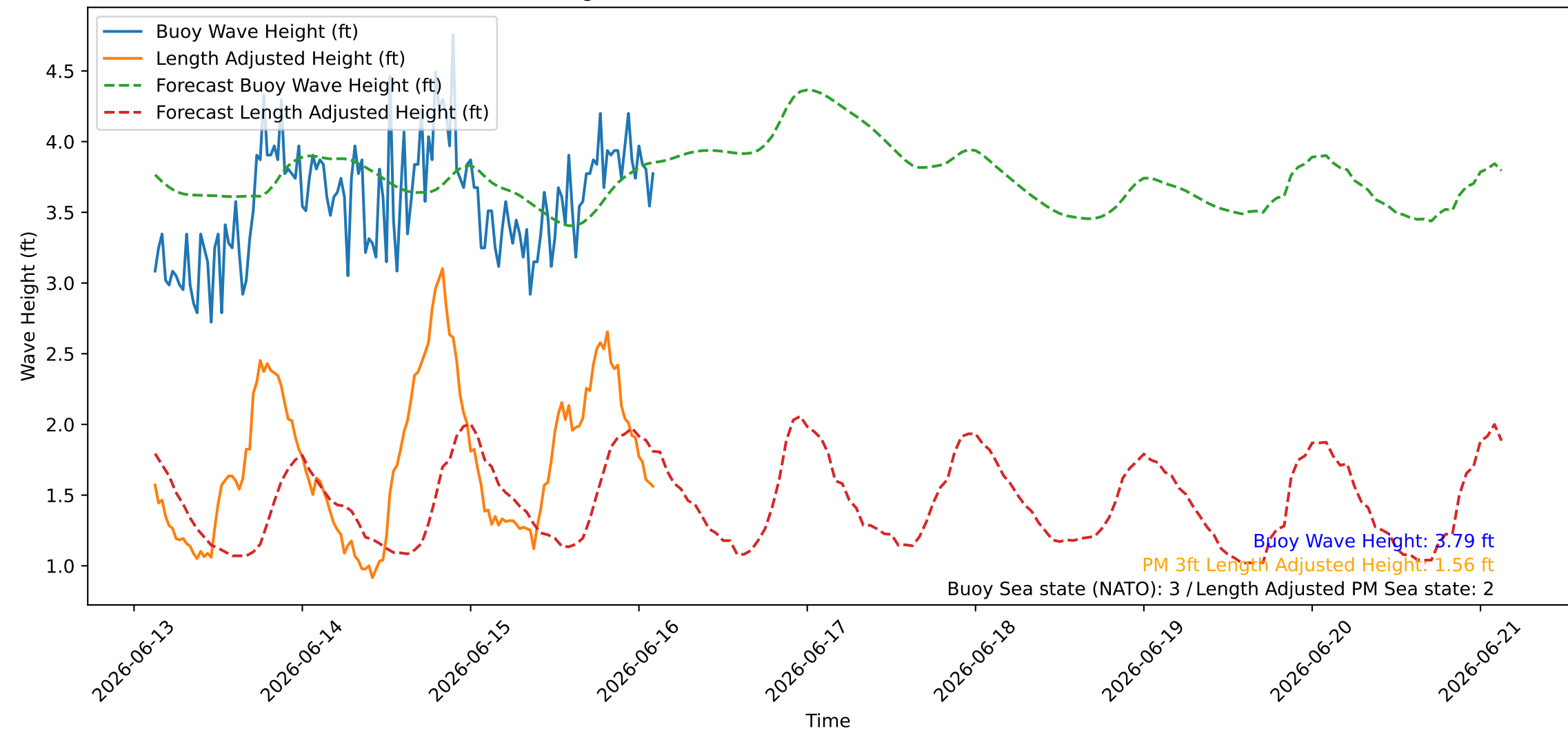
Wave Heights over Time for Red Beach at 2026-06-16 02:40:46
