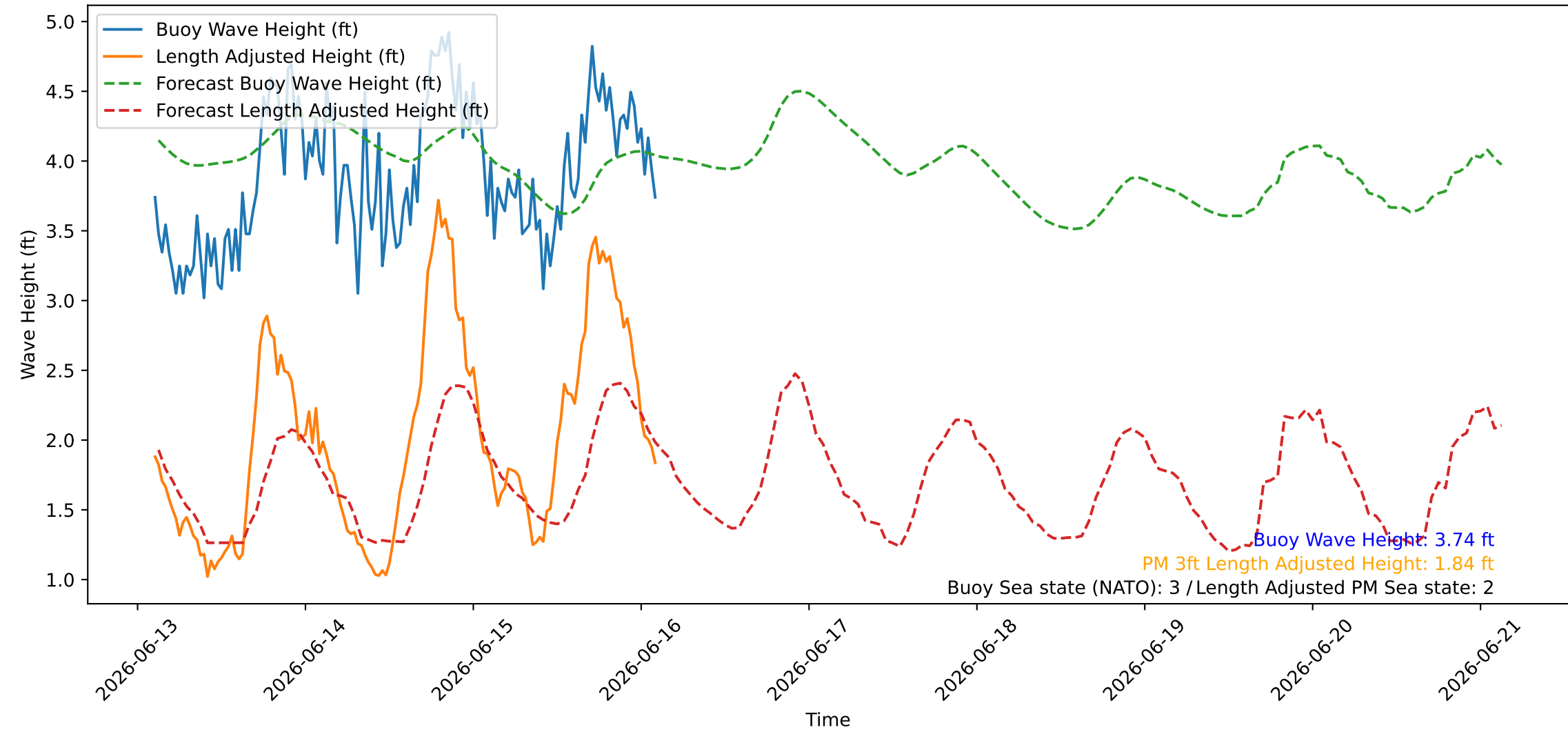
Wave Heights over Time for Green Beach at 2026-06-16 02:41:09
