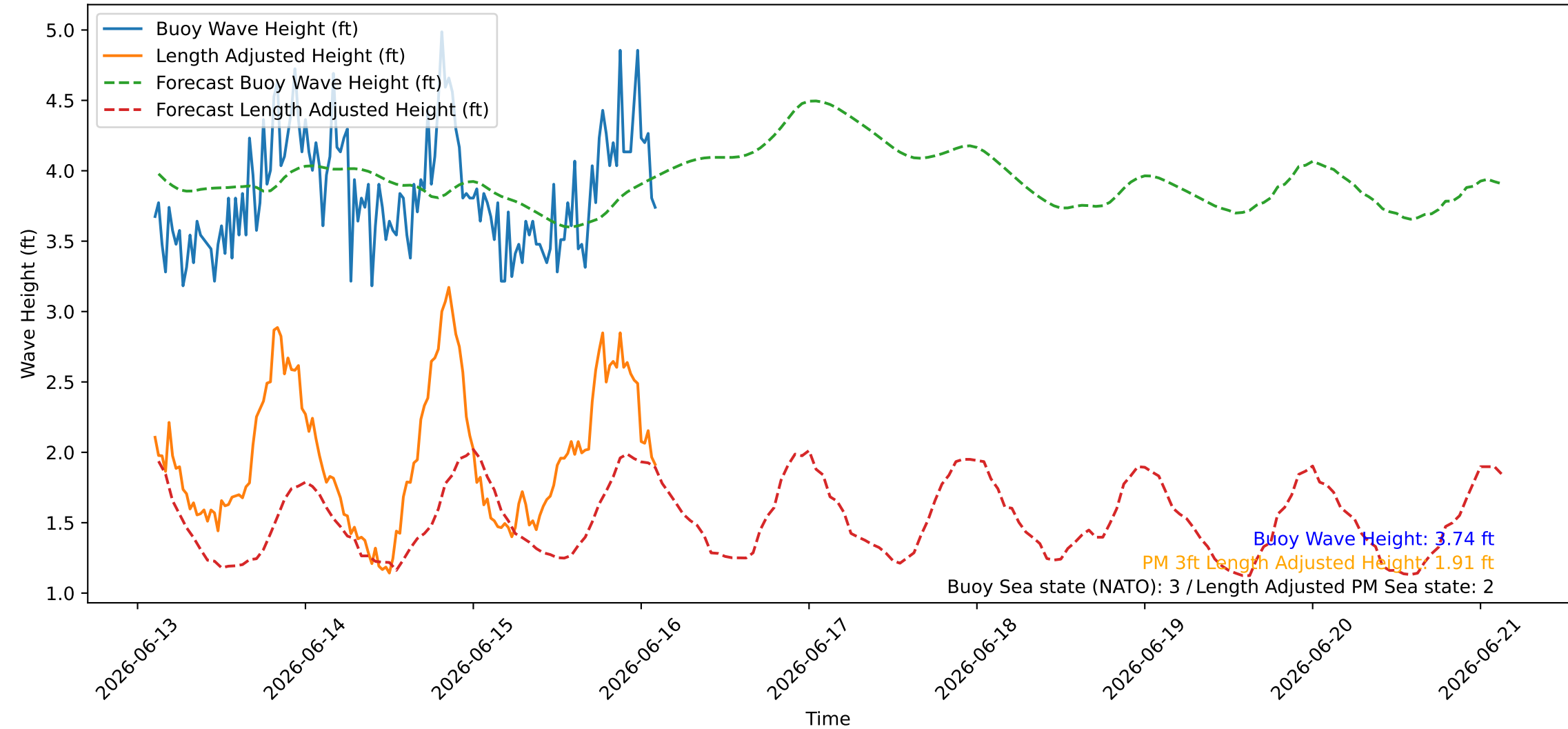
Wave Heights over Time for Oceanside Harbor at 2026-06-16 02:40:27
