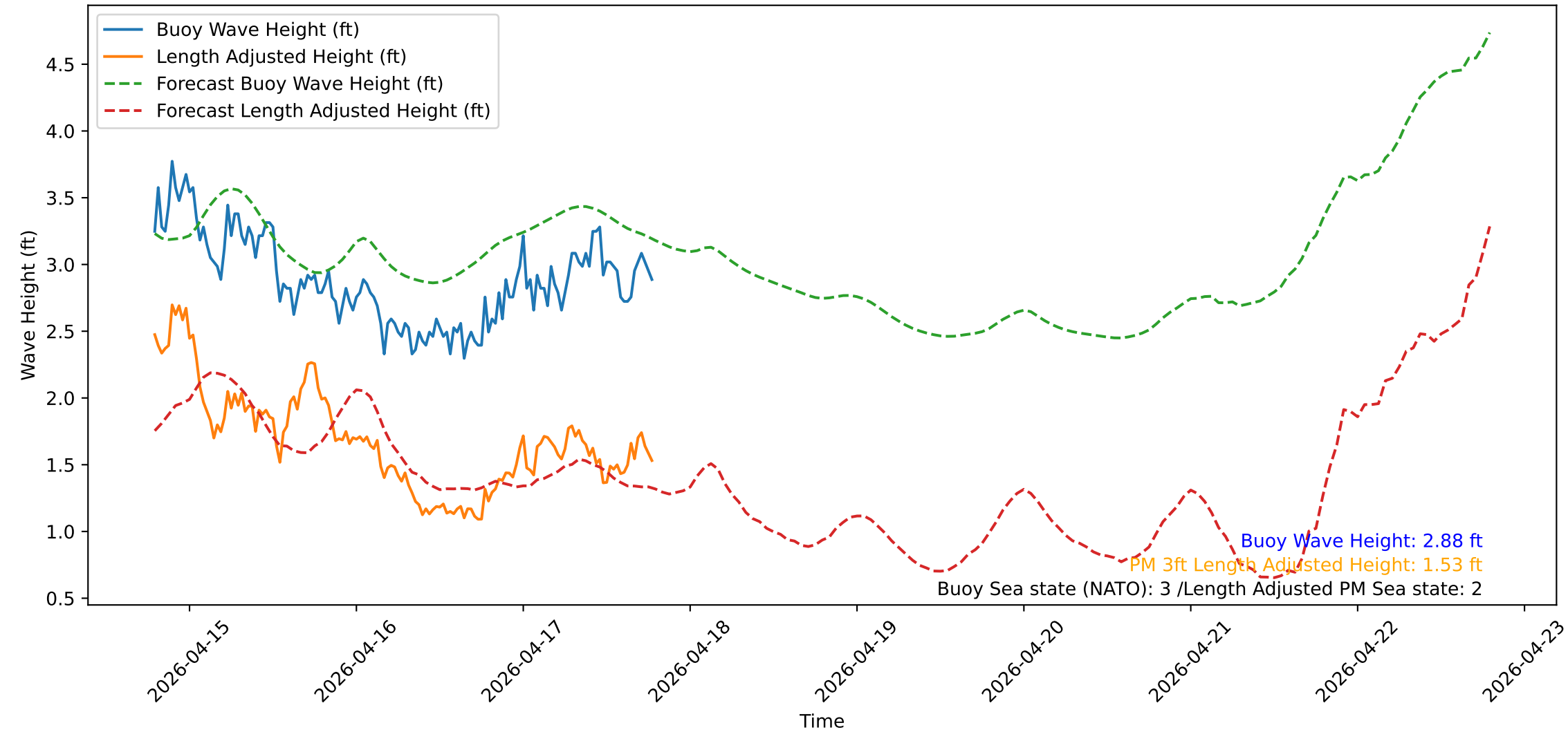
Wave Heights over Time for Oceanside Harbor at 2026-04-17 19:10:32
