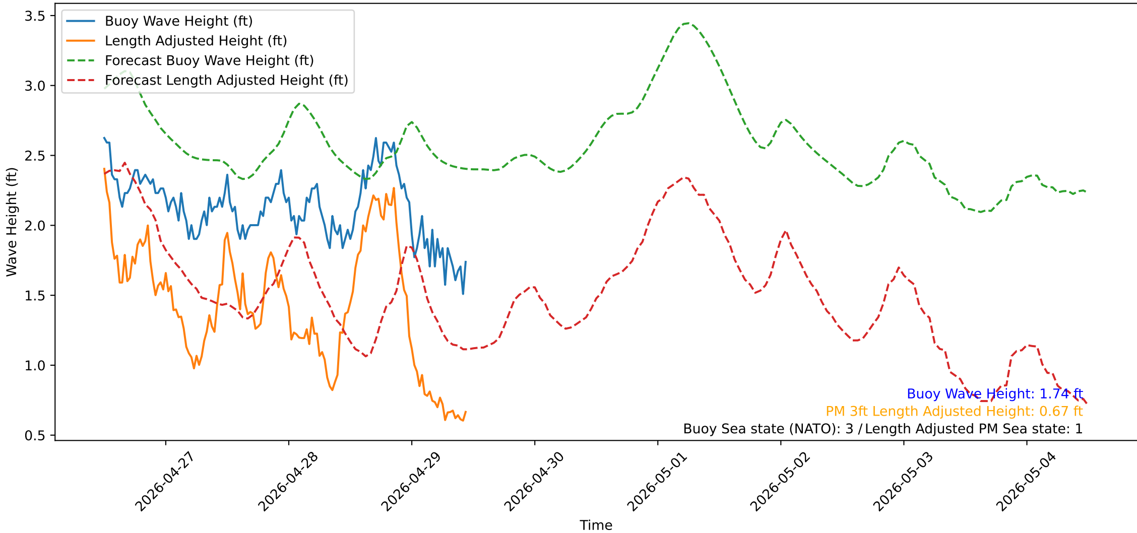
Wave Heights over Time for Red Beach at 2026-04-29 11:40:51
