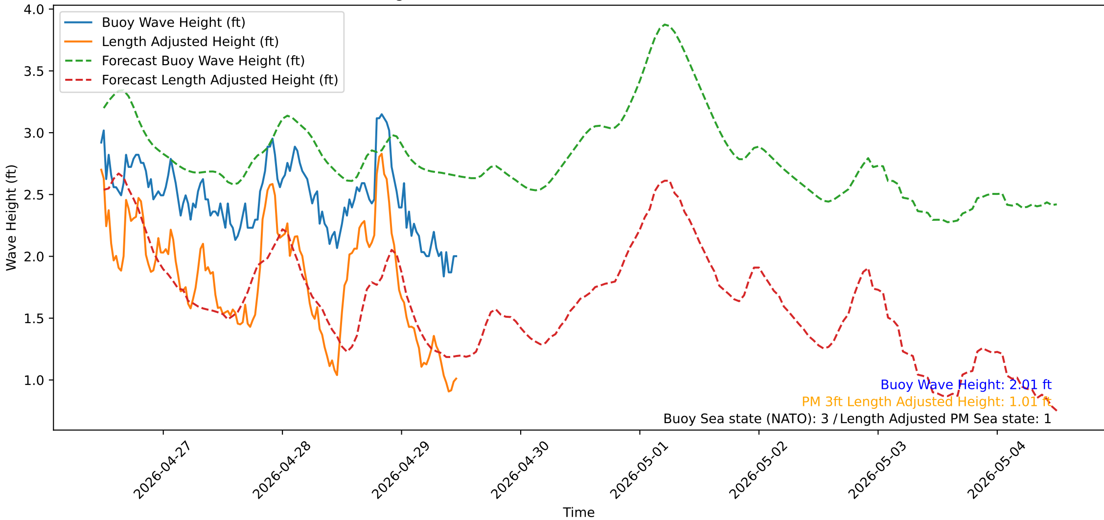
Wave Heights over Time for Green Beach at 2026-04-29 11:41:14
