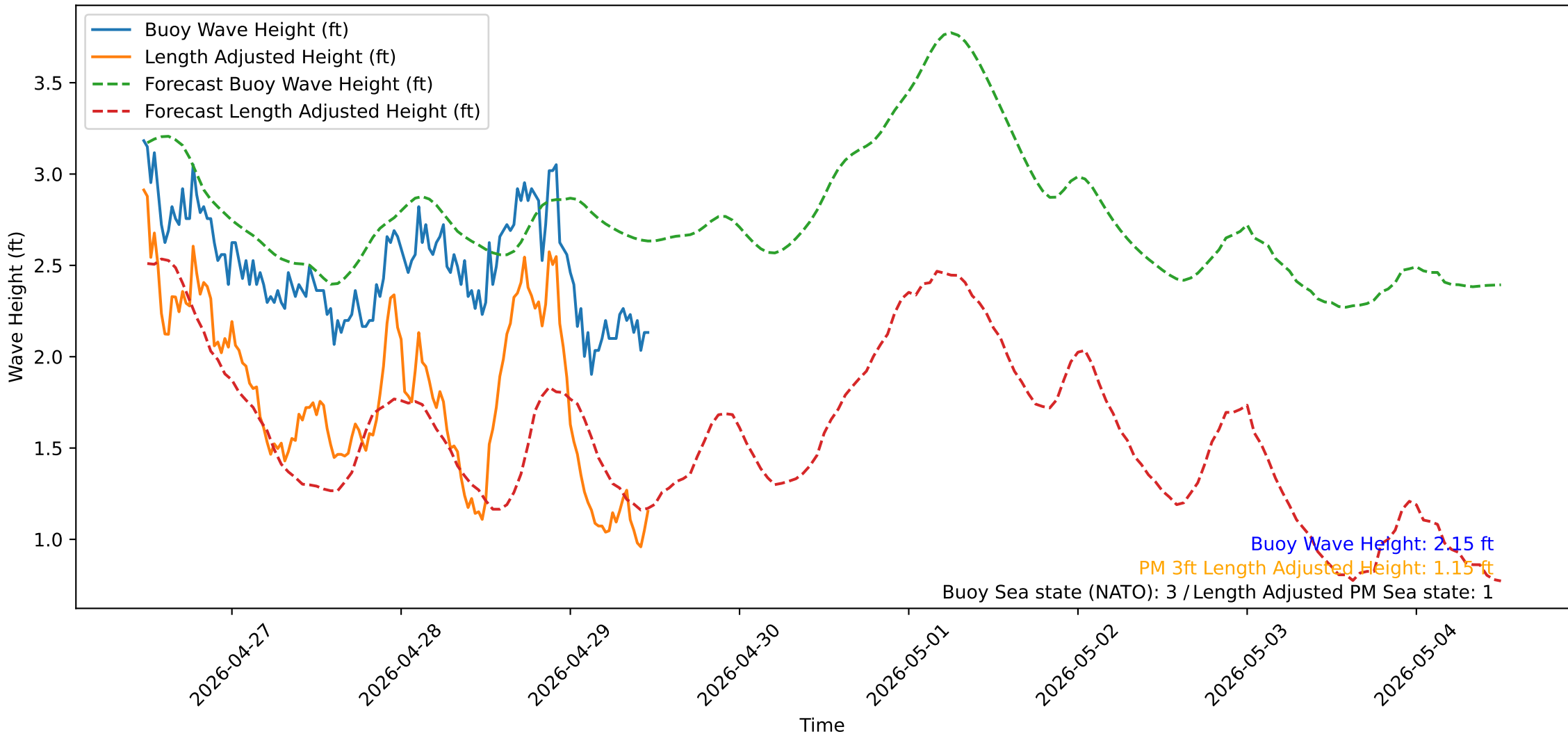
Wave Heights over Time for Oceanside Harbor at 2026-04-29 11:40:31
