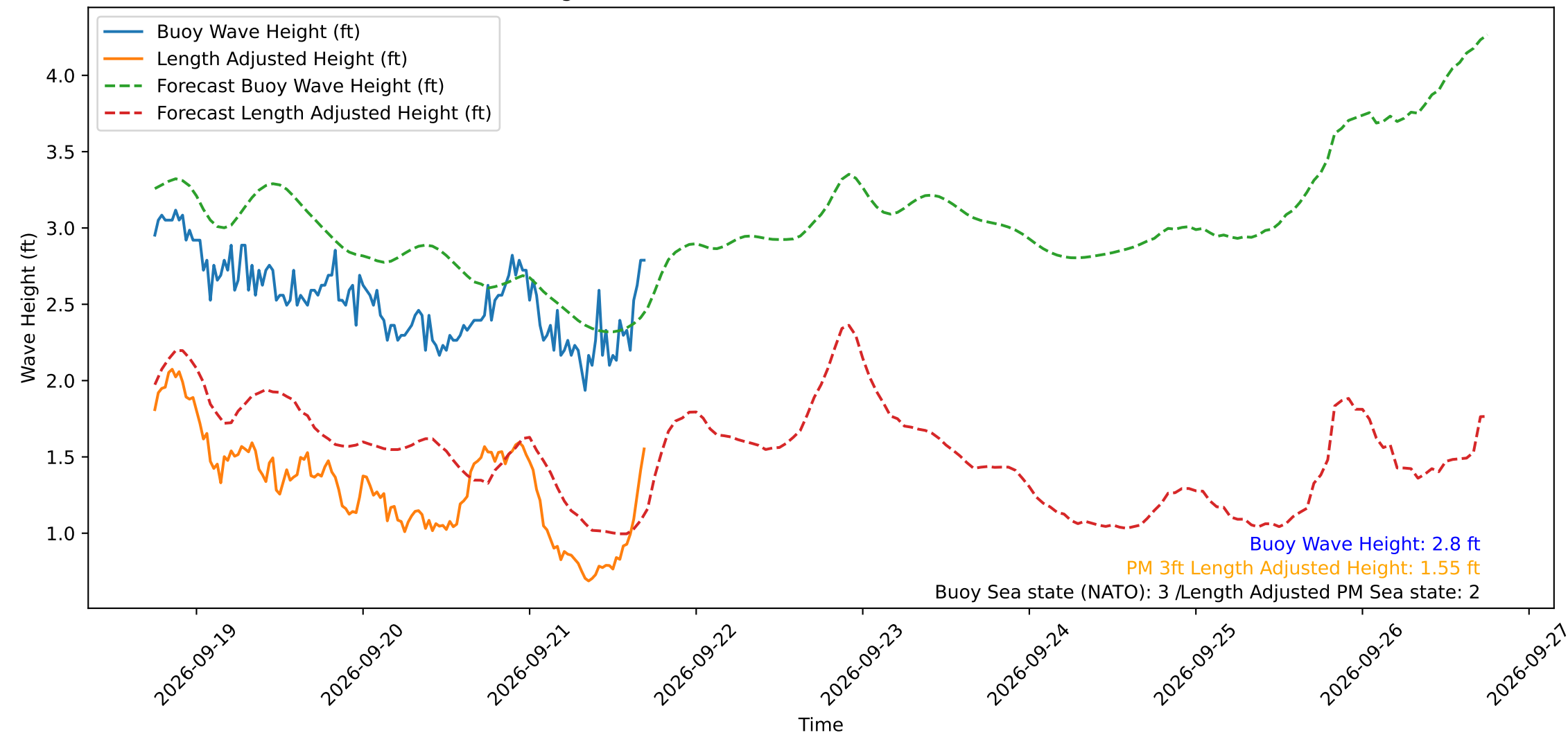
Wave Heights over Time for Green Beach at 2026-09-21 17:31:12
