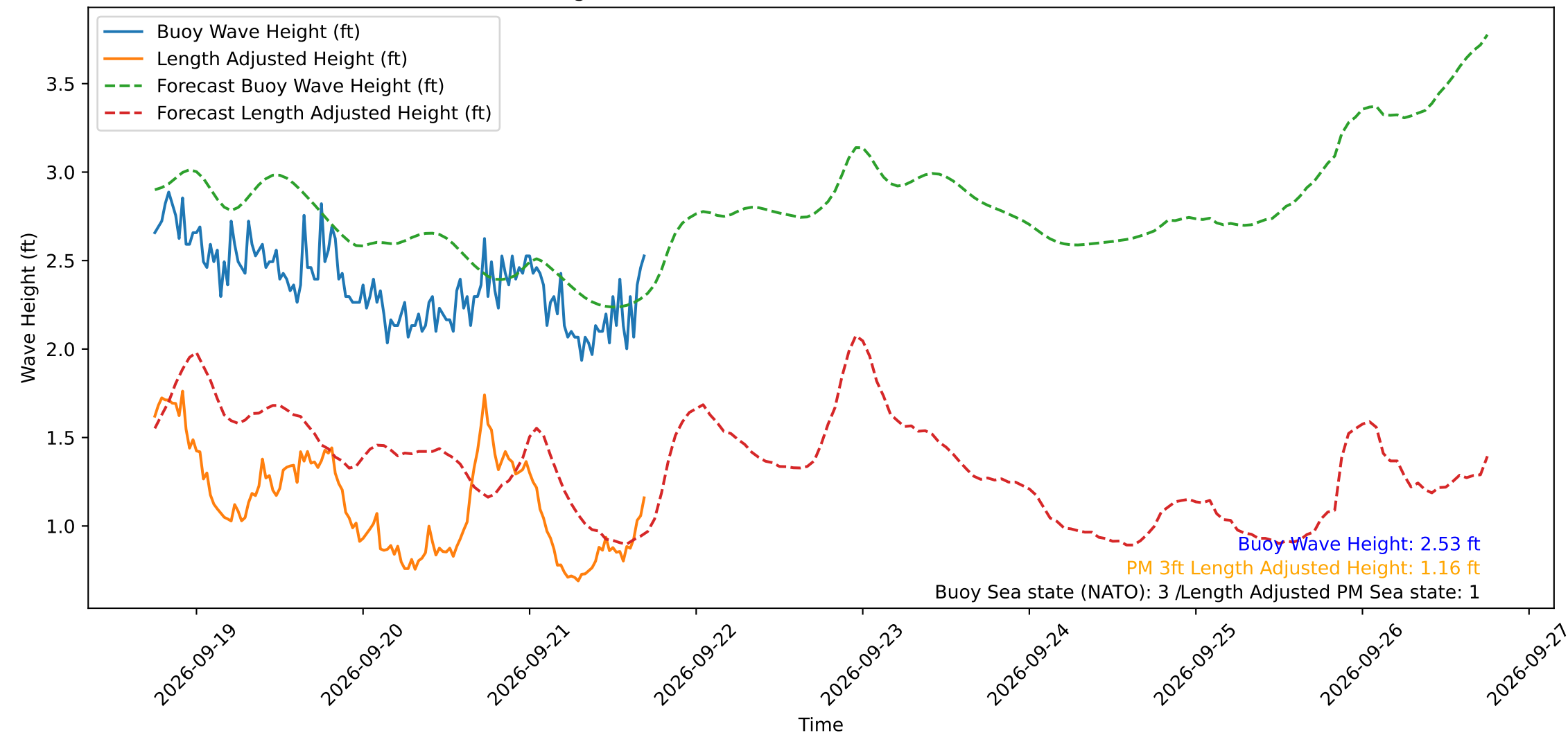
Wave Heights over Time for Red Beach at 2026-09-21 17:30:50
