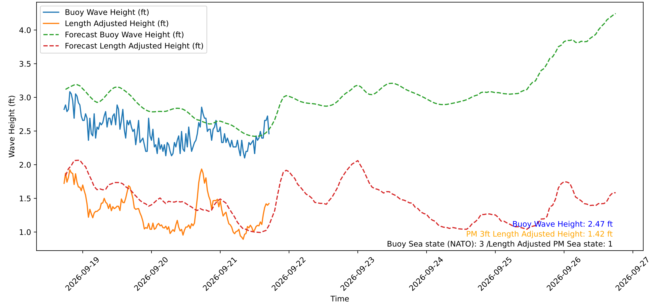
Wave Heights over Time for Oceanside Harbor at 2026-09-21 17:30:30
