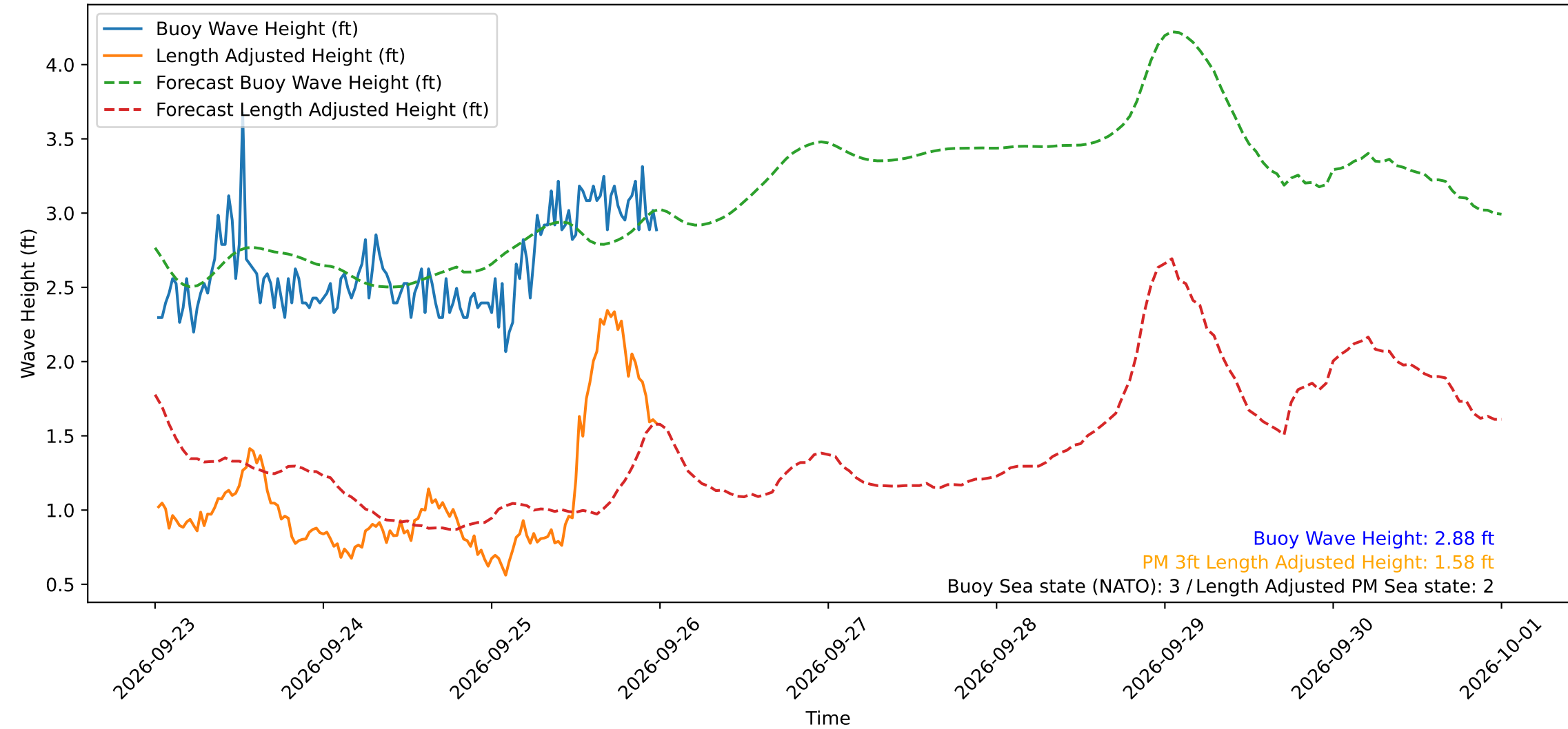
Wave Heights over Time for Red Beach at 2026-09-26 00:10:50
