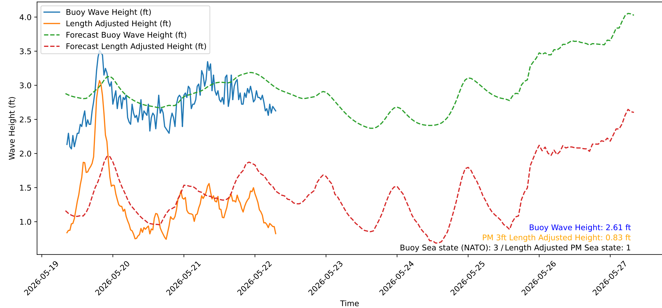
Wave Heights over Time for Red Beach at 2026-05-22 08:10:52
