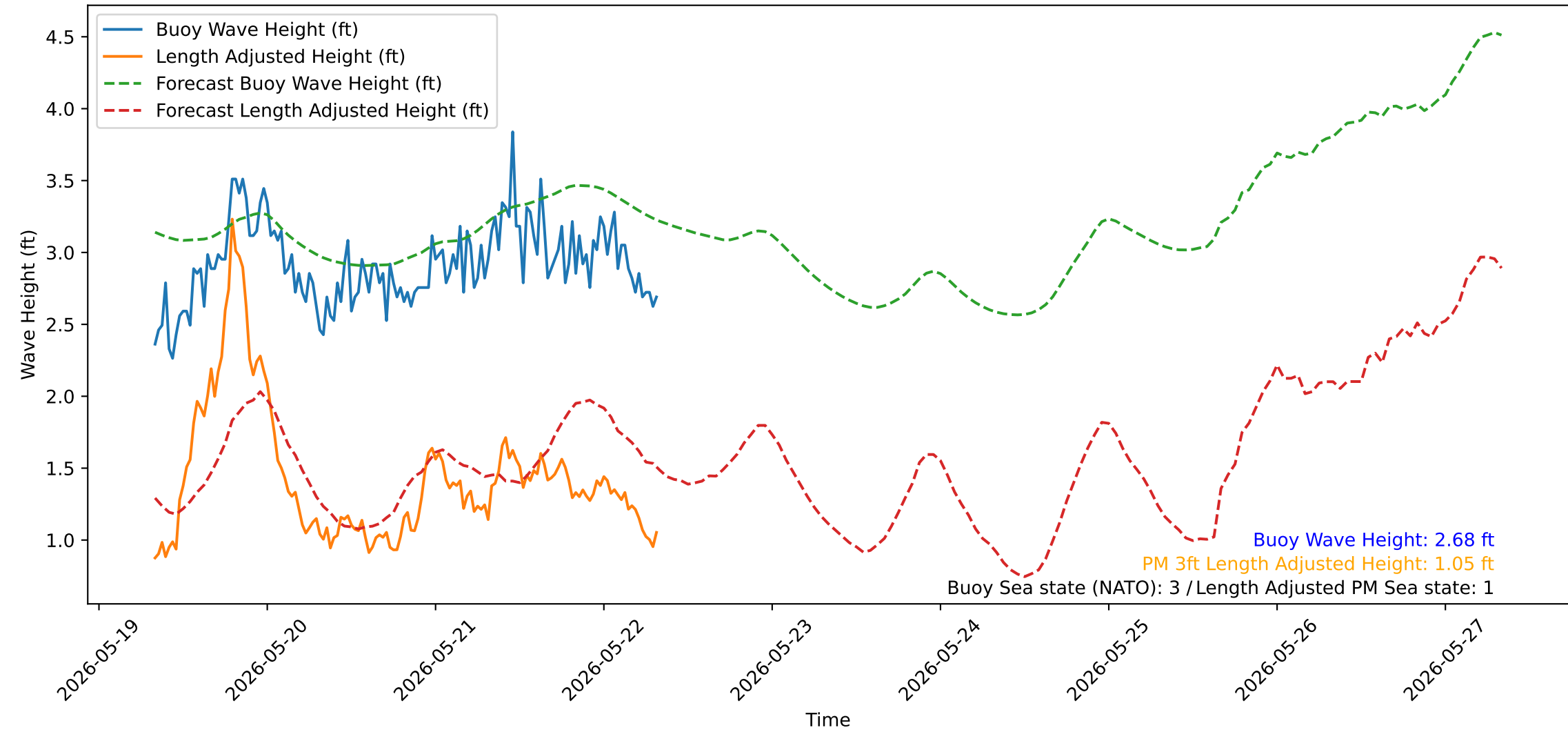
Wave Heights over Time for Oceanside Harbor at 2026-05-22 08:10:32
