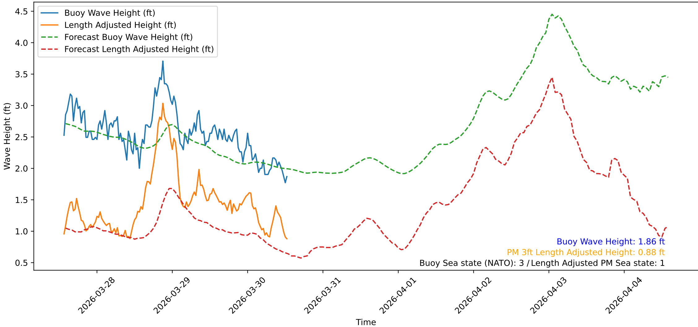
Wave Heights over Time for Green Beach at 2026-03-30 13:31:10
