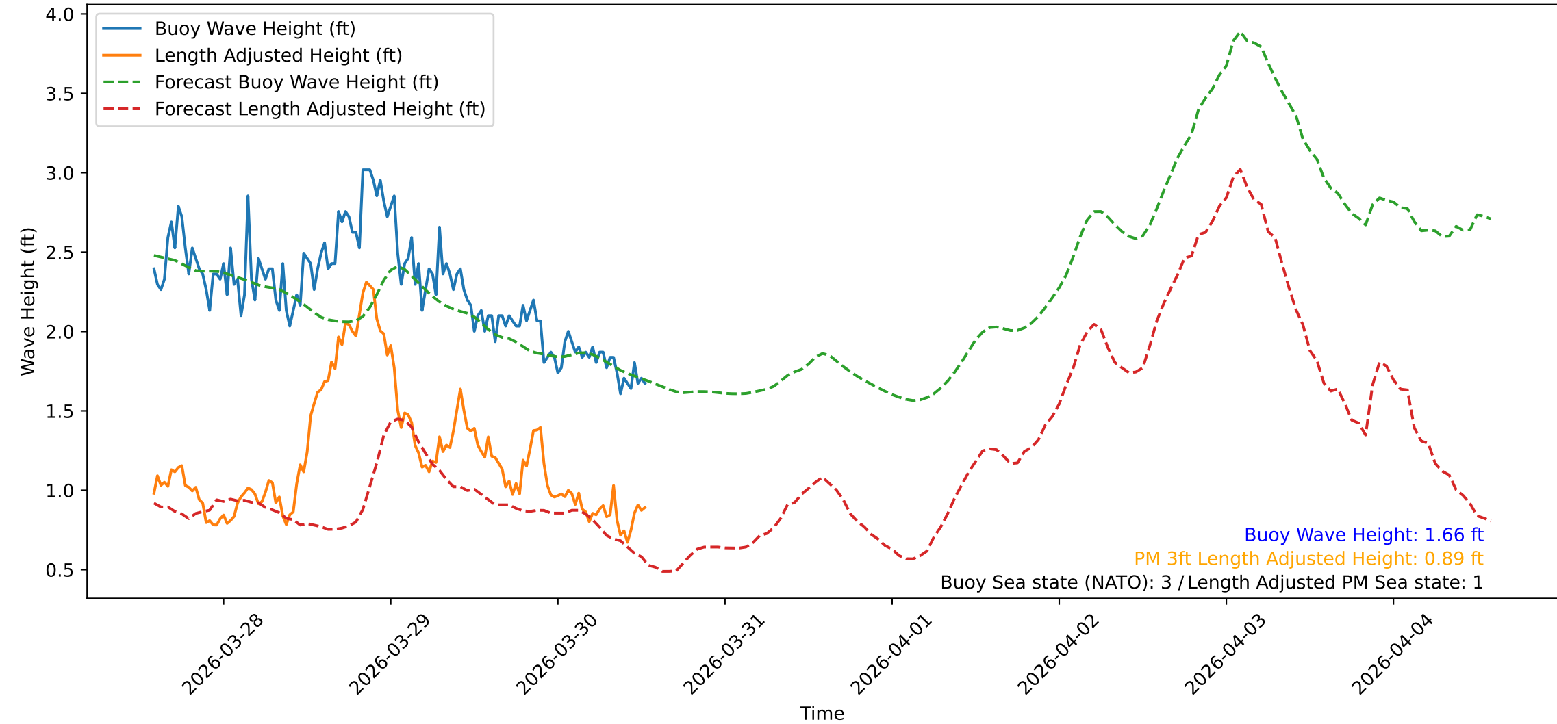
Wave Heights over Time for Red Beach at 2026-03-30 13:30:48
