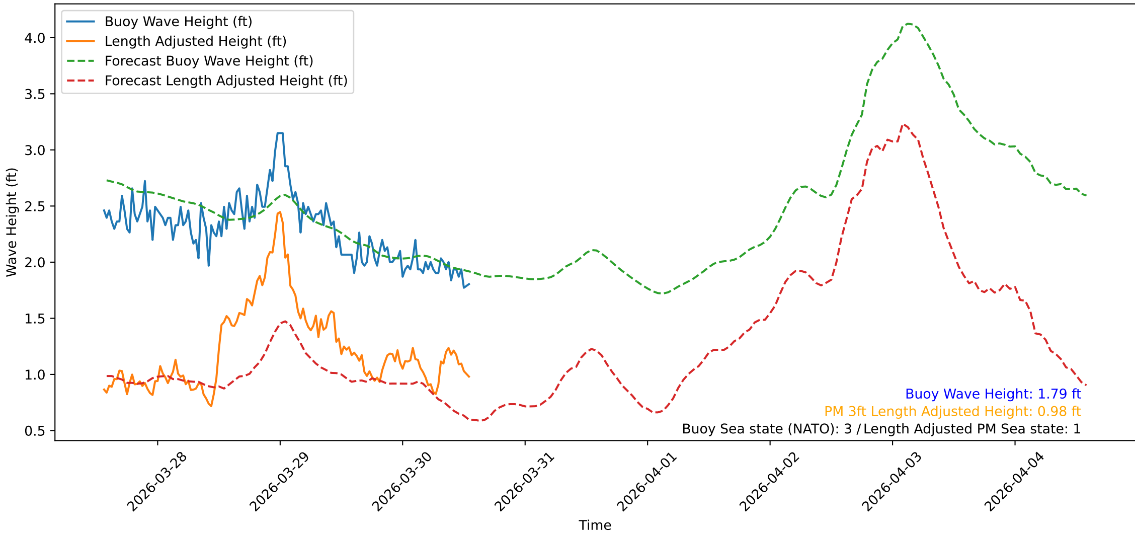
Wave Heights over Time for Oceanside Harbor at 2026-03-30 13:30:32
