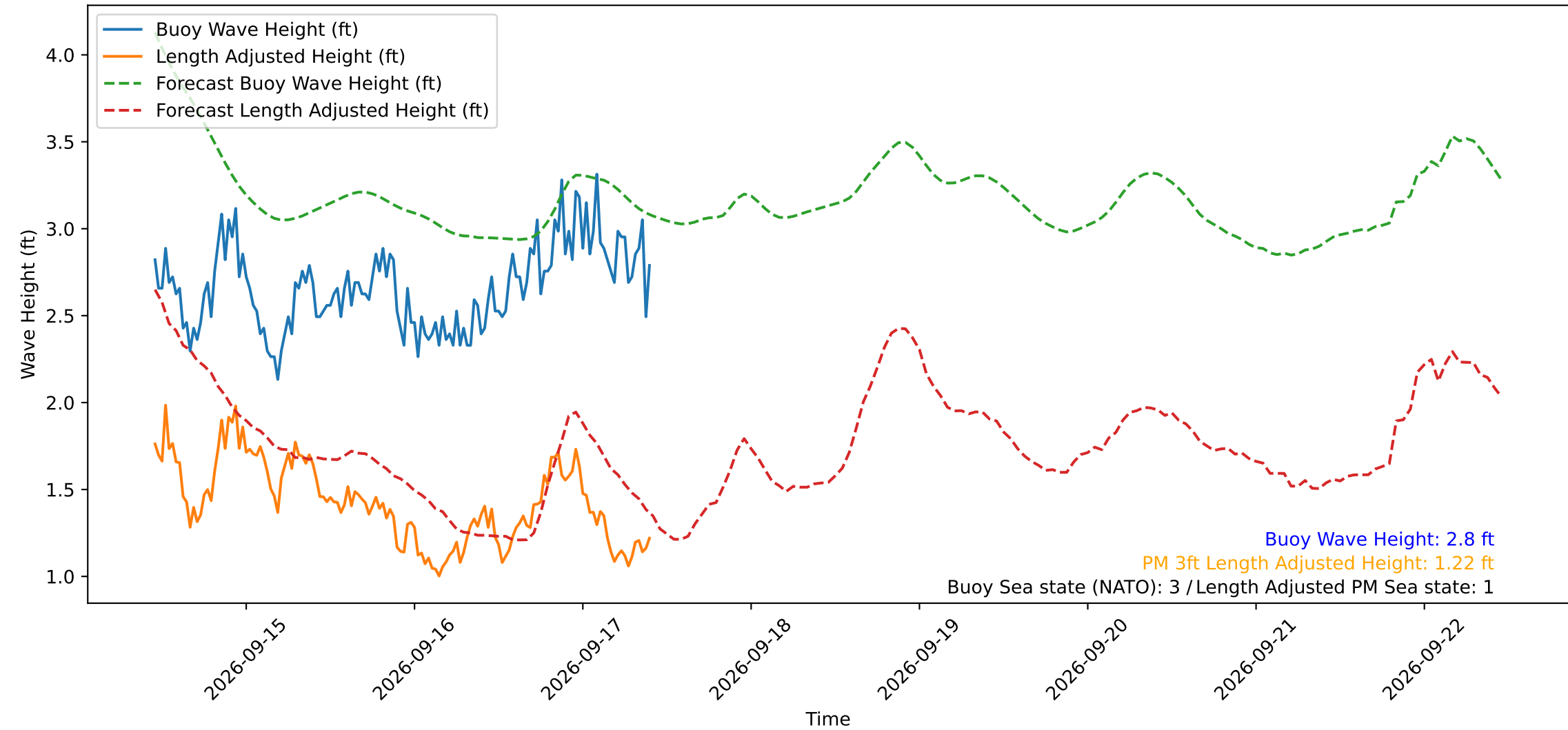
Wave Heights over Time for Green Beach at 2026-09-17 10:31:11
