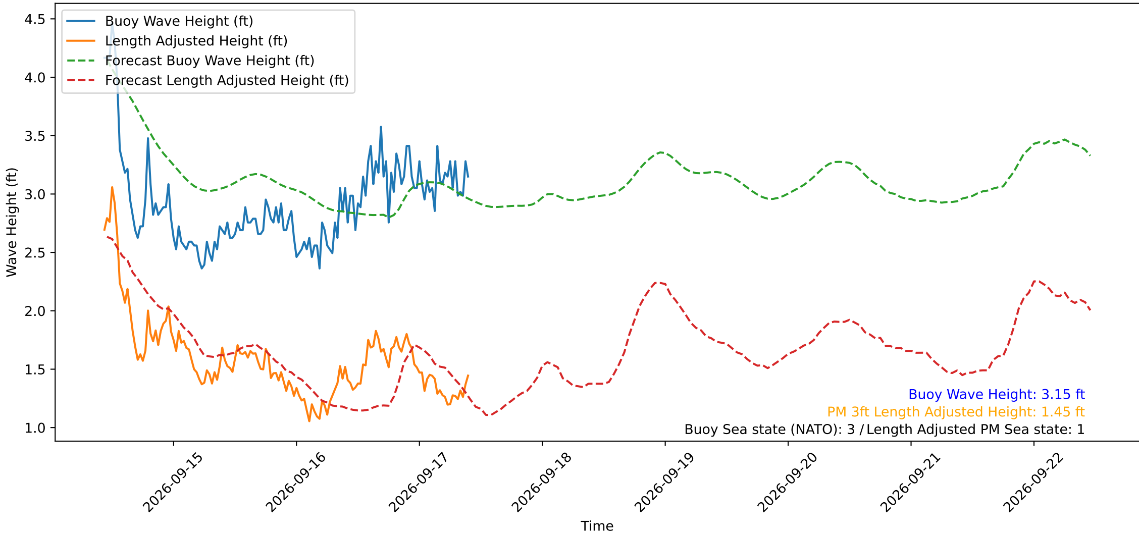
Wave Heights over Time for Oceanside Harbor at 2026-09-17 10:30:29
