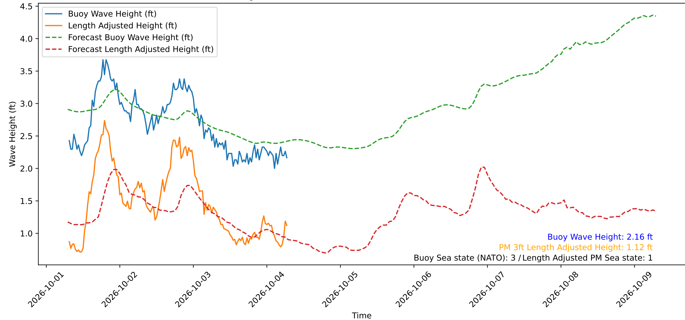
Wave Heights over Time for Green Beach at 2026-10-04 07:11:11
