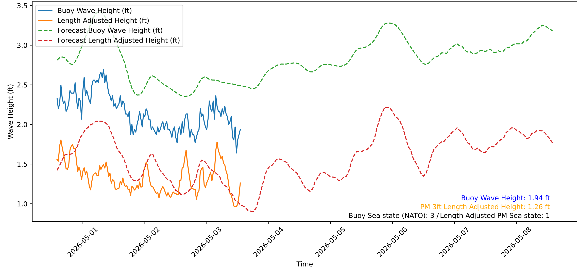
Wave Heights over Time for Oceanside Harbor at 2026-05-03 13:50:32
