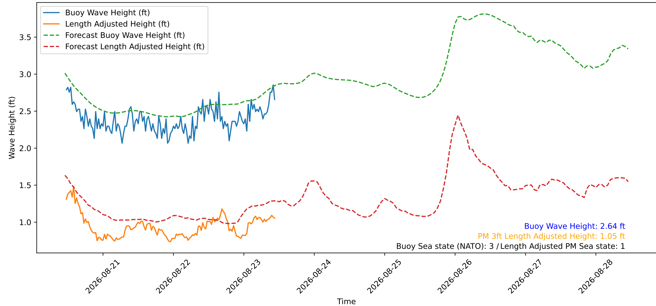
Wave Heights over Time for Red Beach at 2026-08-23 11:20:51
