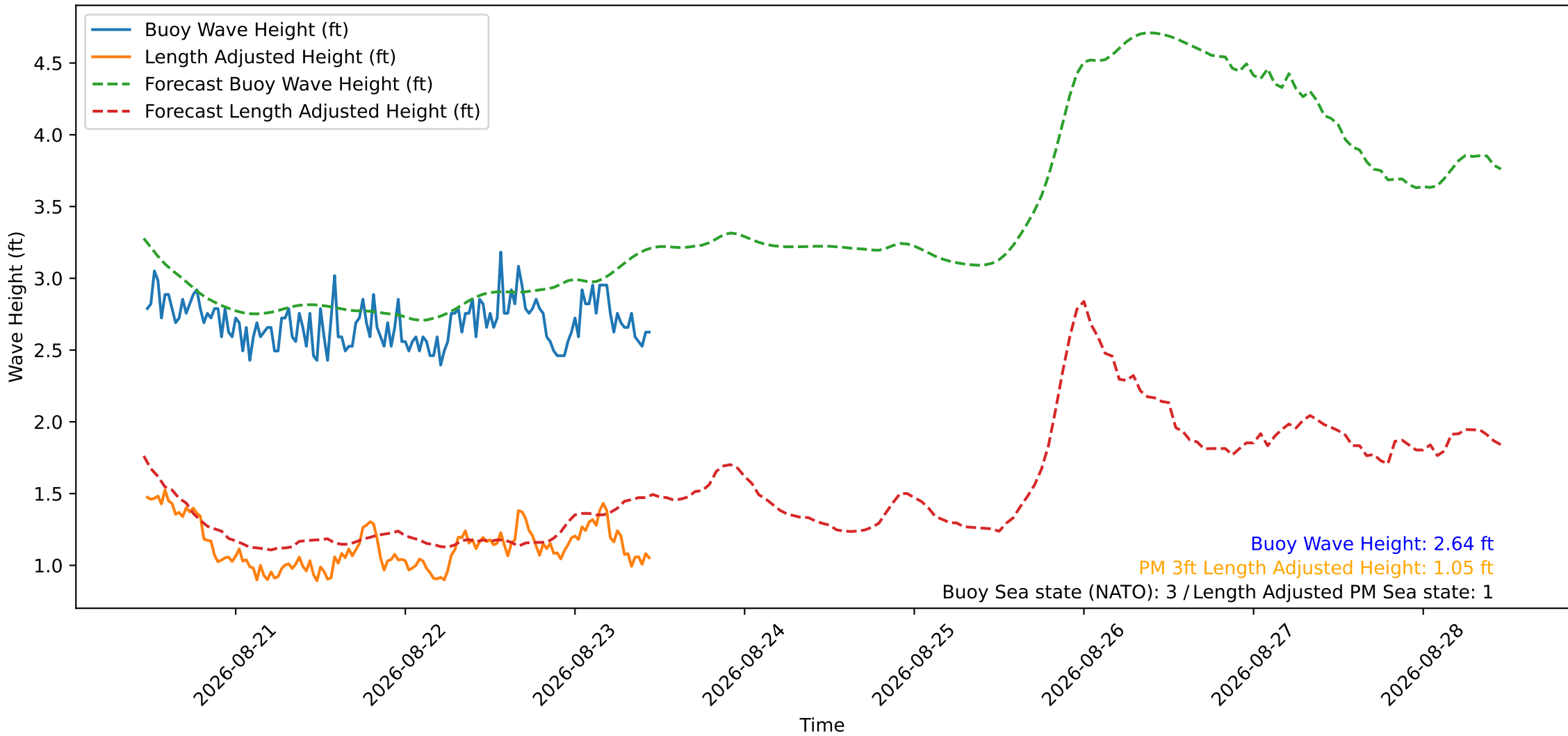
Wave Heights over Time for Green Beach at 2026-08-23 11:21:15
