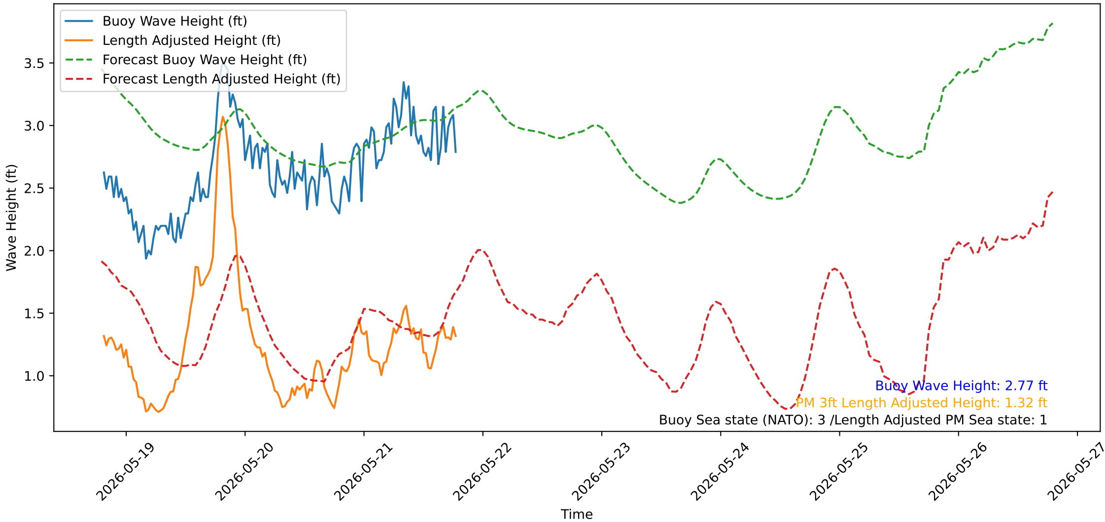
Wave Heights over Time for Red Beach at 2026-05-21 19:10:50
