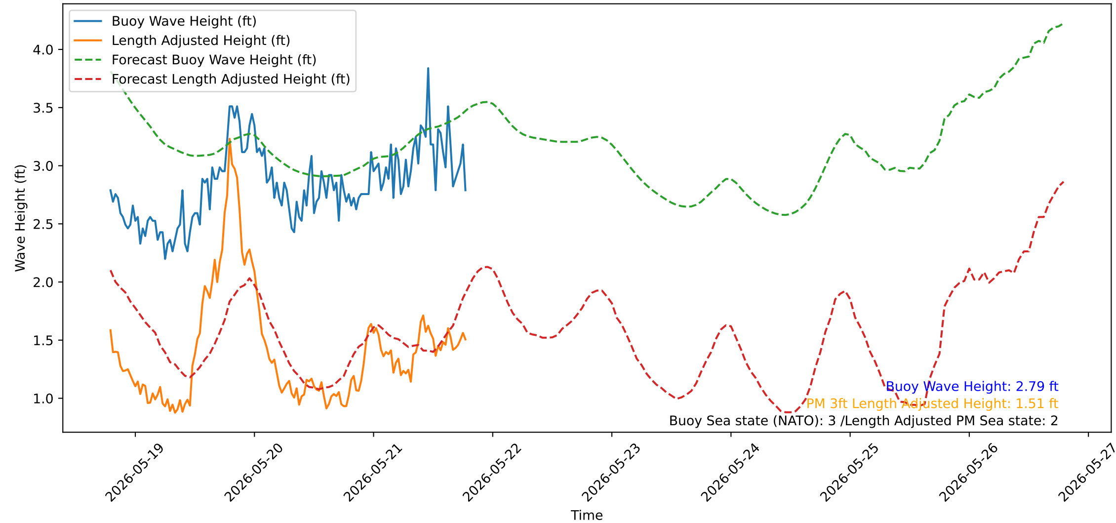
Wave Heights over Time for Oceanside Harbor at 2026-05-21 19:10:31
