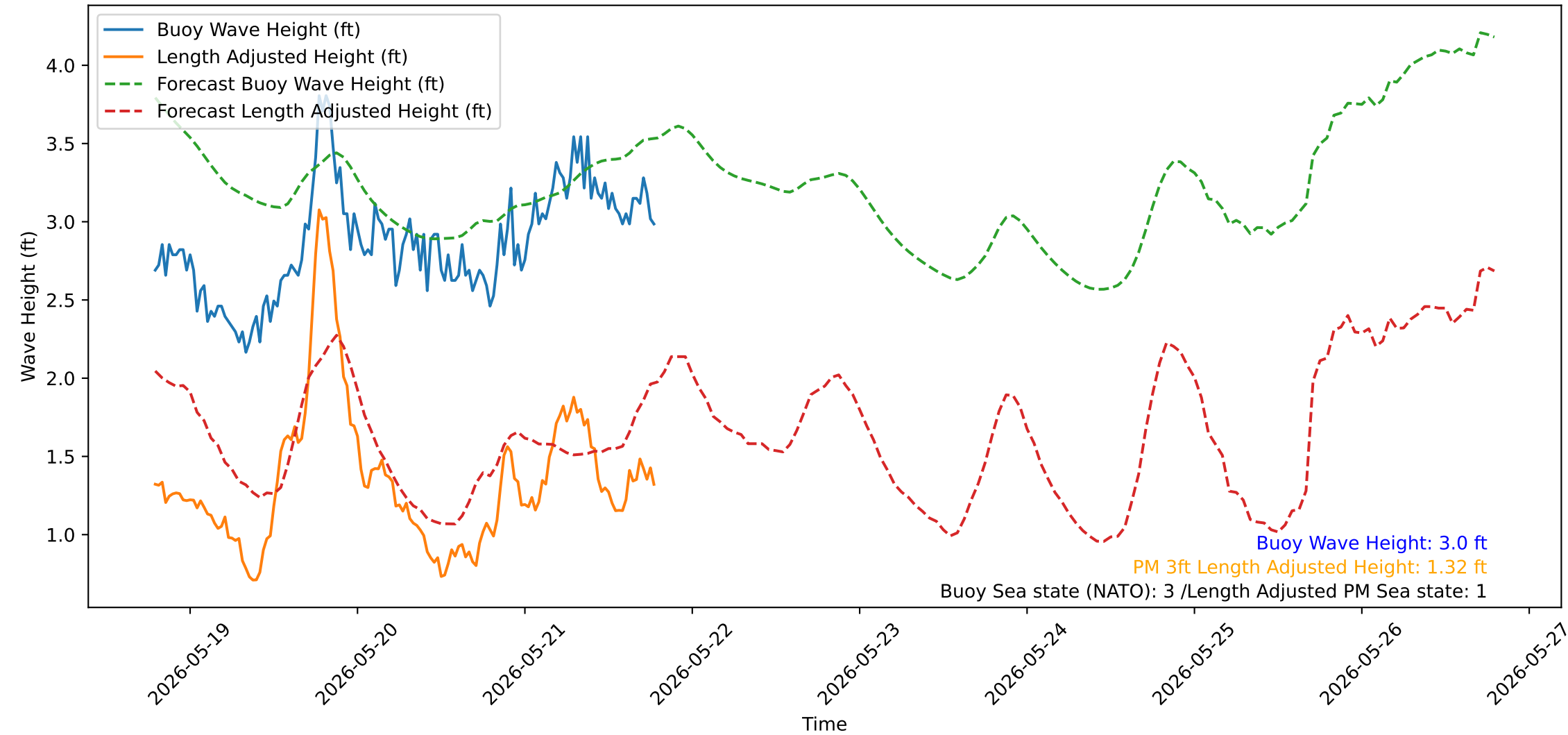
Wave Heights over Time for Green Beach at 2026-05-21 19:11:13
