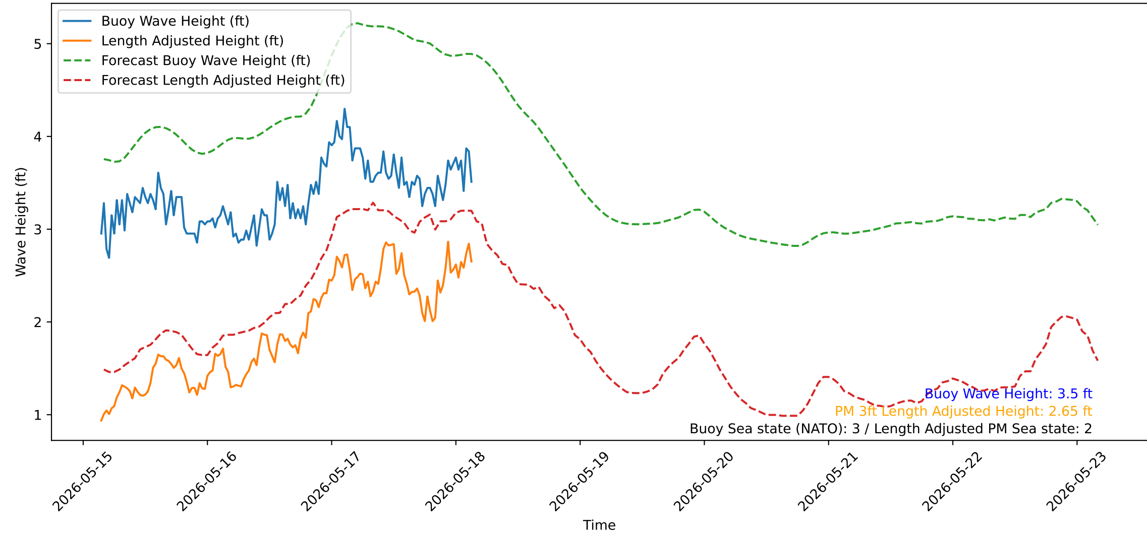
Wave Heights over Time for Oceanside Harbor at 2026-05-18 03:40:31
