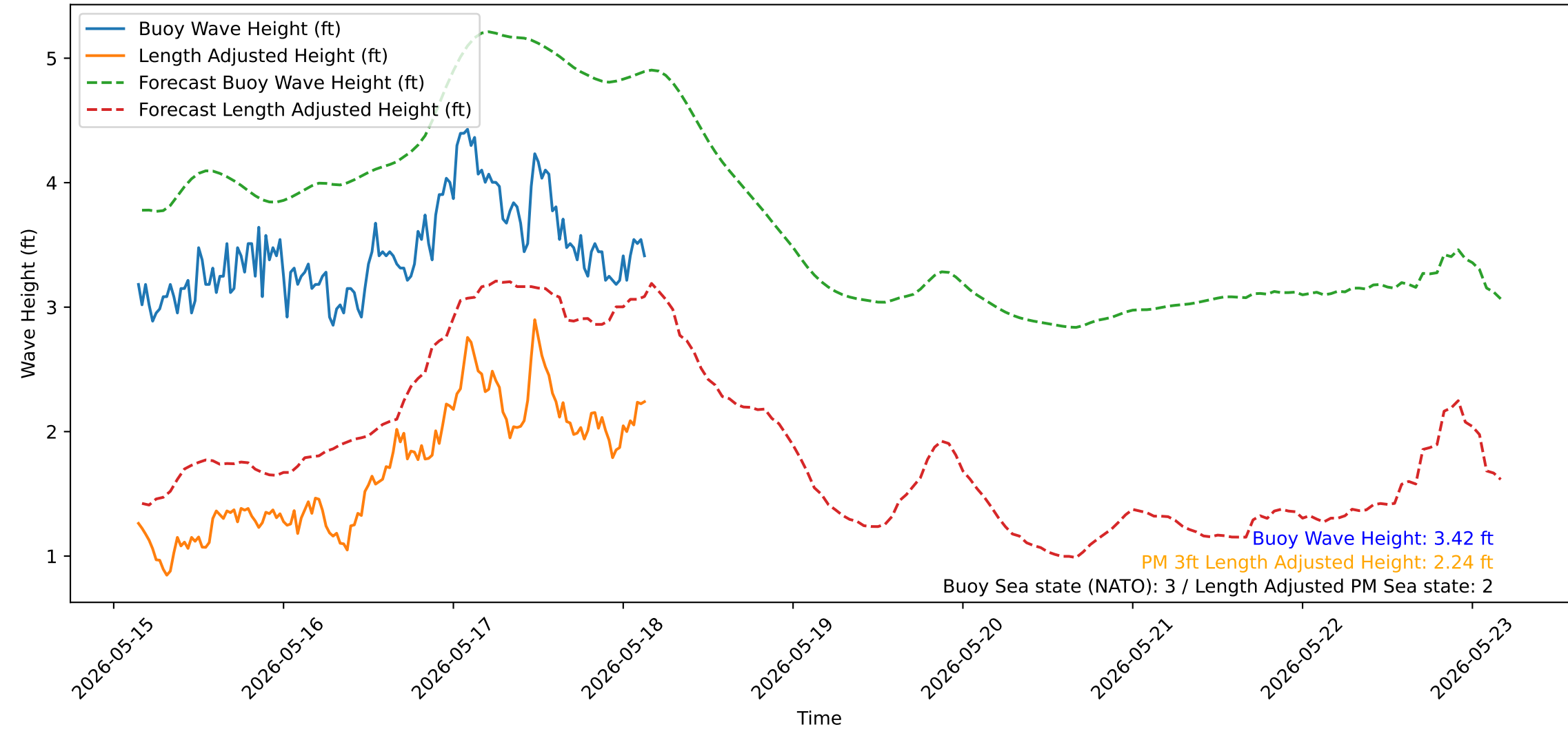
Wave Heights over Time for Green Beach at 2026-05-18 03:41:13
