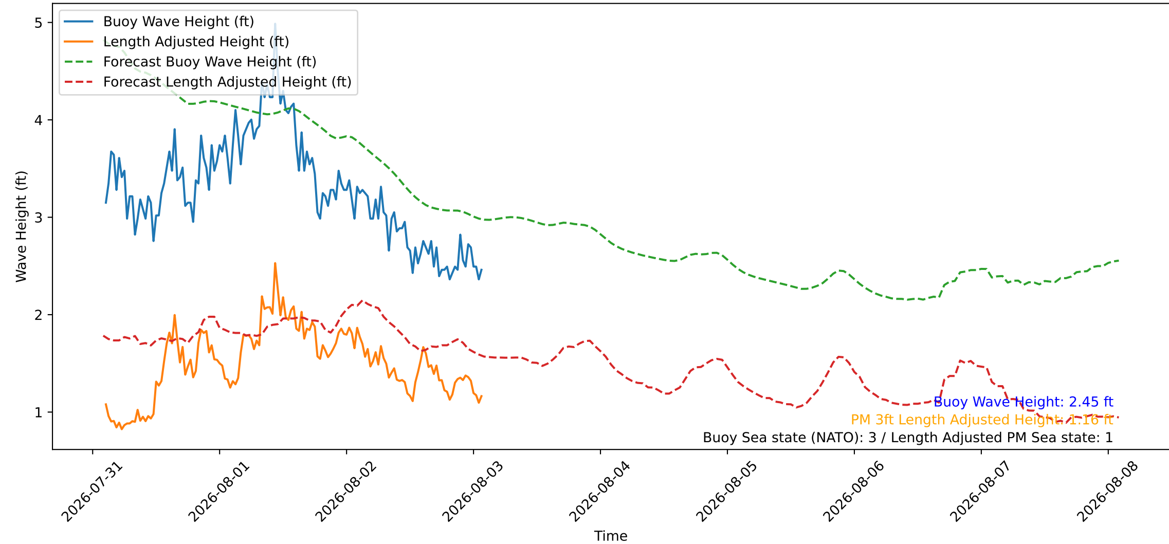
Wave Heights over Time for Green Beach at 2026-08-03 02:21:10
