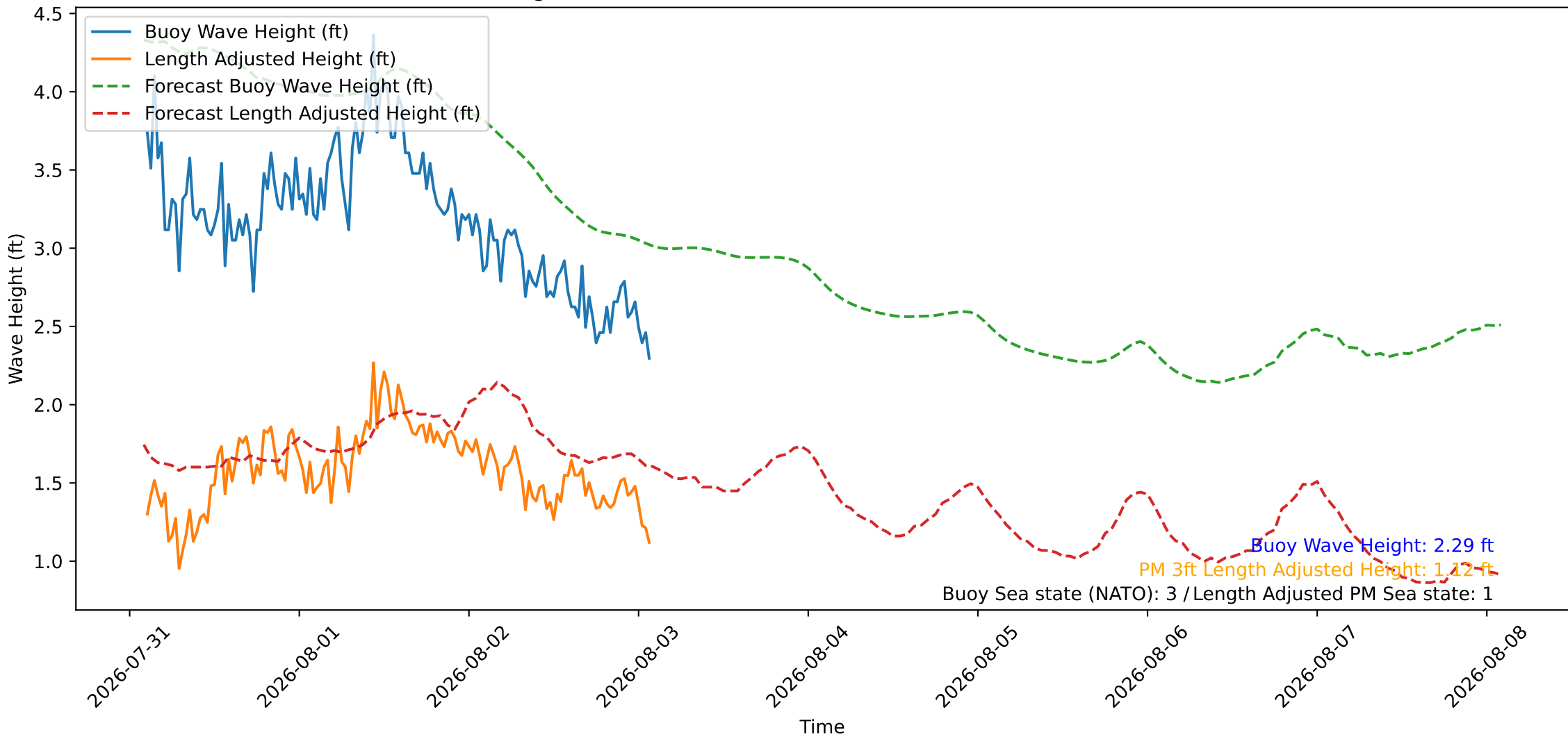
Wave Heights over Time for Oceanside Harbor at 2026-08-03 02:20:26
