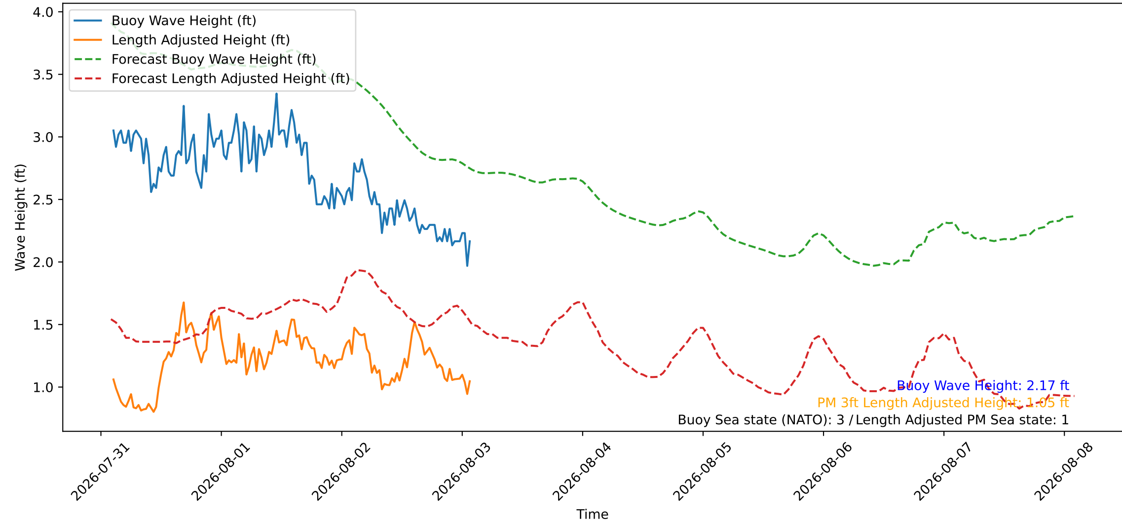
Wave Heights over Time for Red Beach at 2026-08-03 02:20:47
