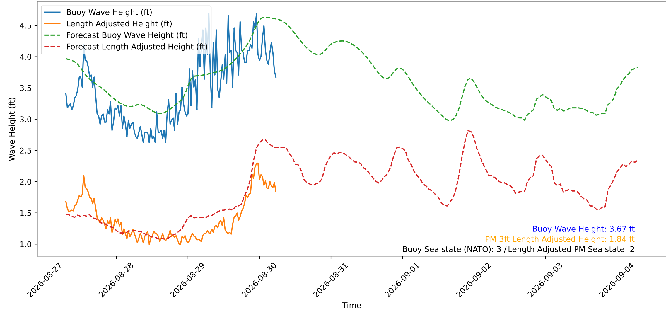
Wave Heights over Time for Red Beach at 2026-08-30 06:30:49
