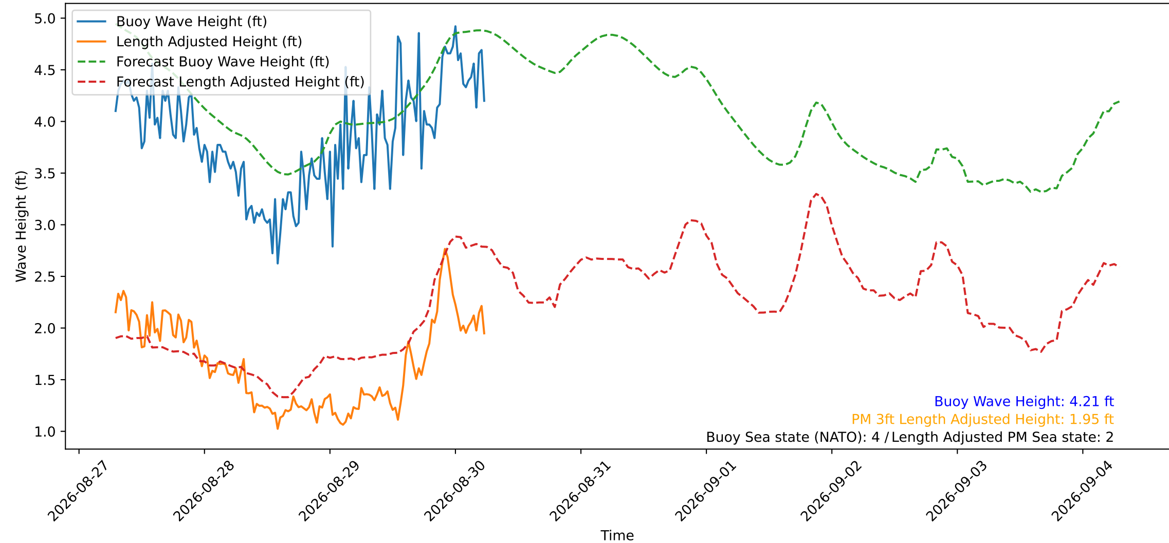
Wave Heights over Time for Green Beach at 2026-08-30 06:31:11
