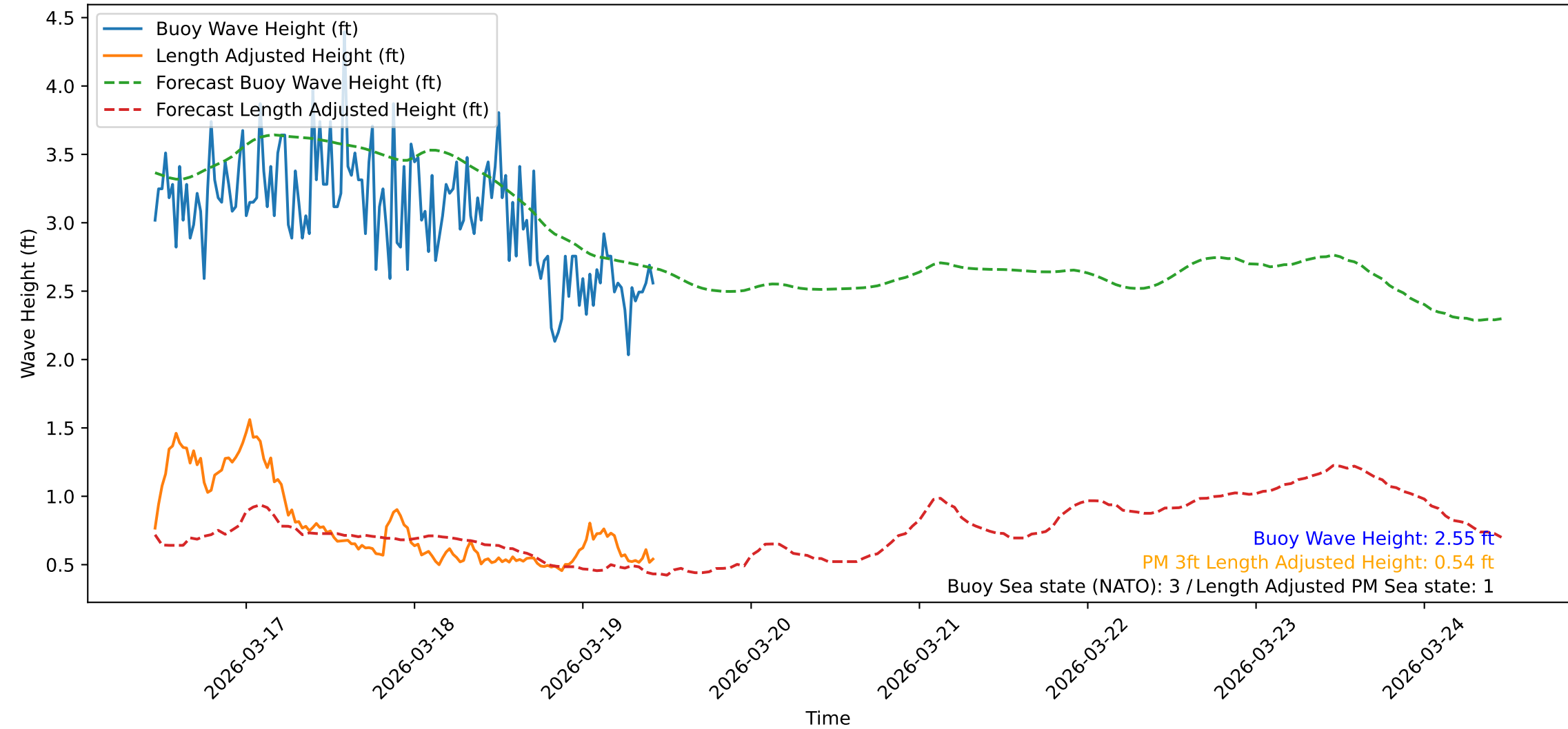
Wave Heights over Time for Oceanside Harbor at 2026-03-19 10:50:31
