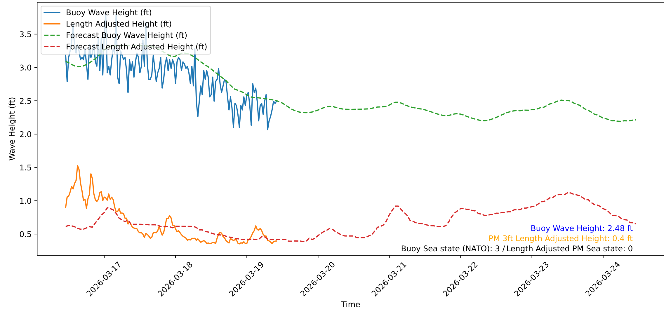
Wave Heights over Time for Red Beach at 2026-03-19 10:50:47
