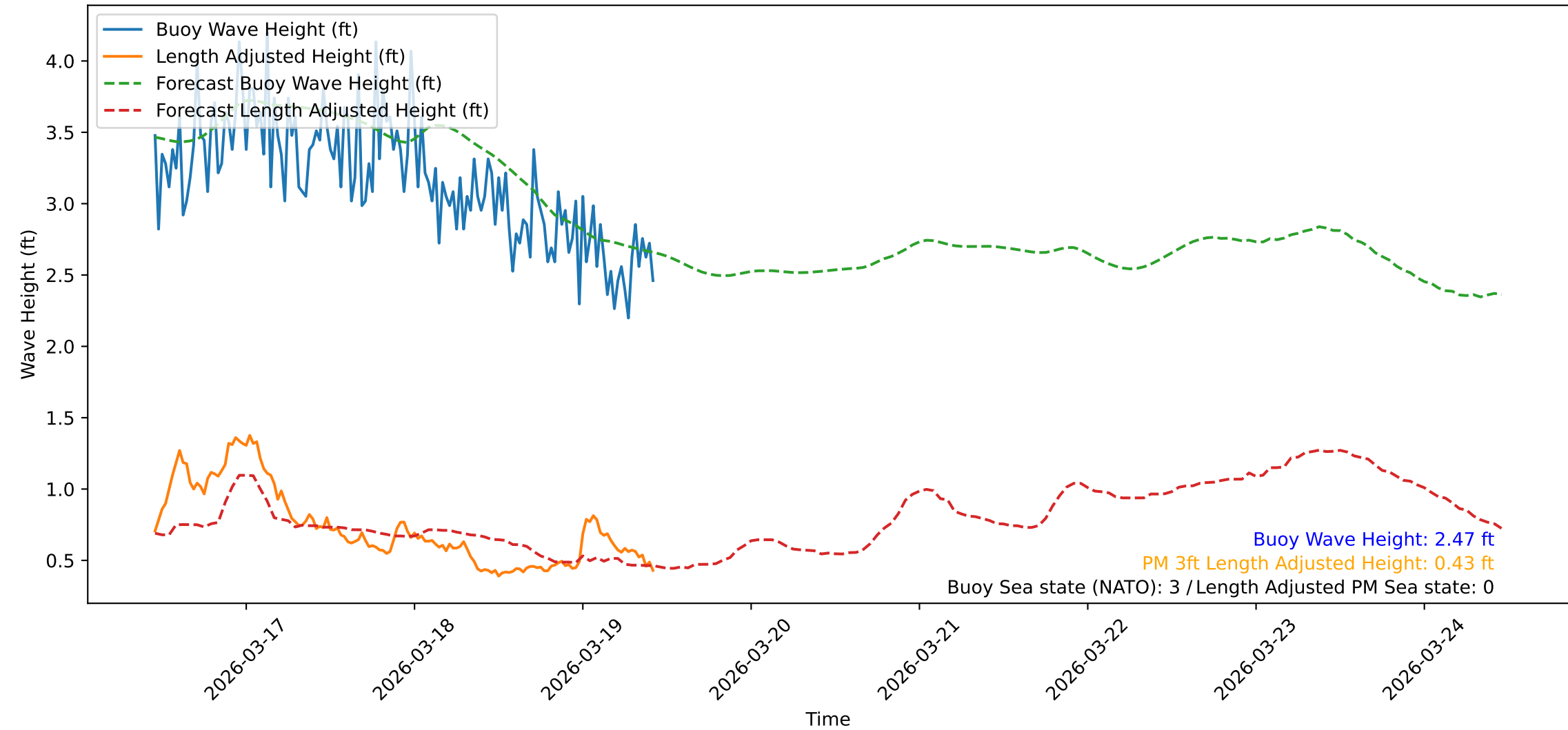
Wave Heights over Time for Green Beach at 2026-03-19 10:51:10
