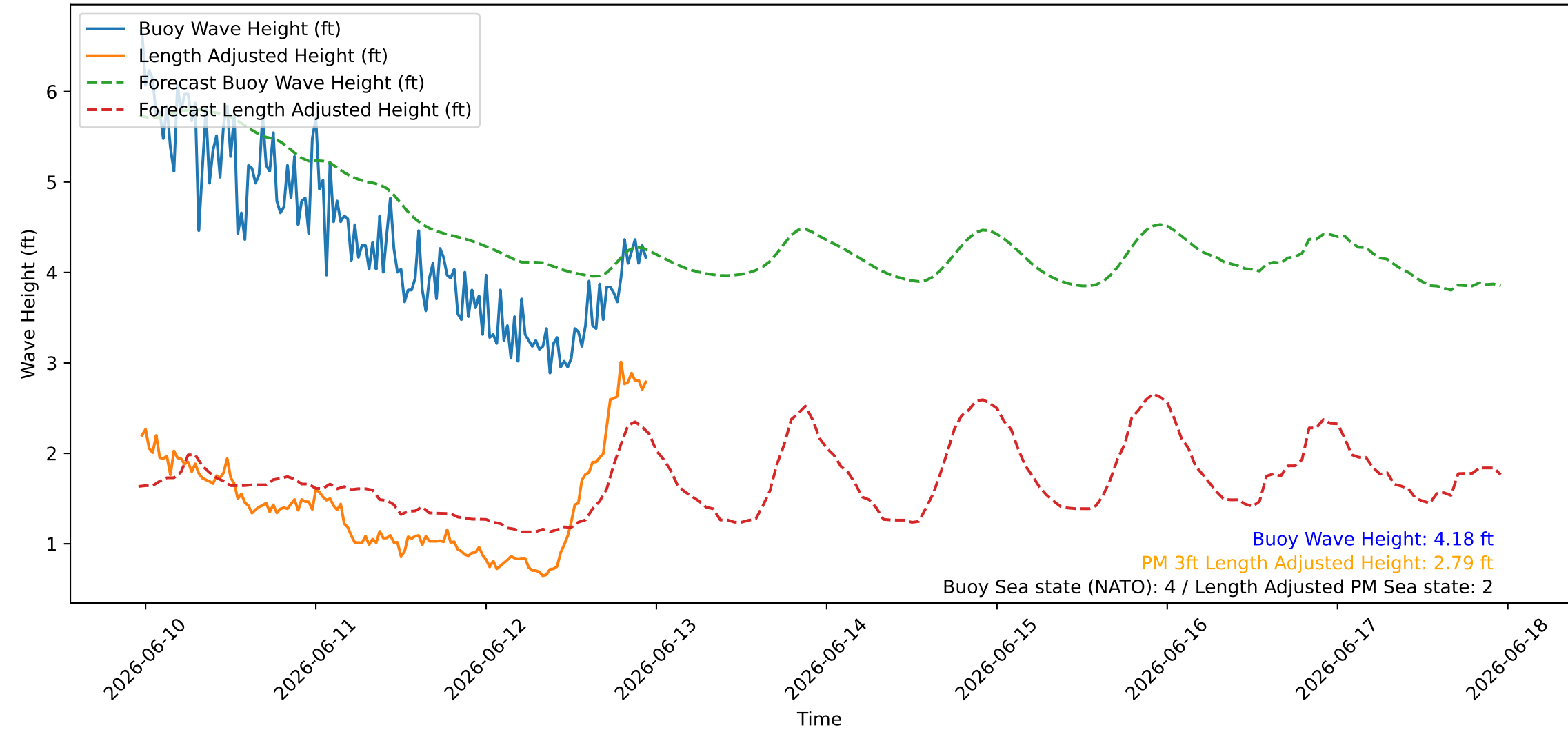
Wave Heights over Time for Green Beach at 2026-06-12 23:21:09
