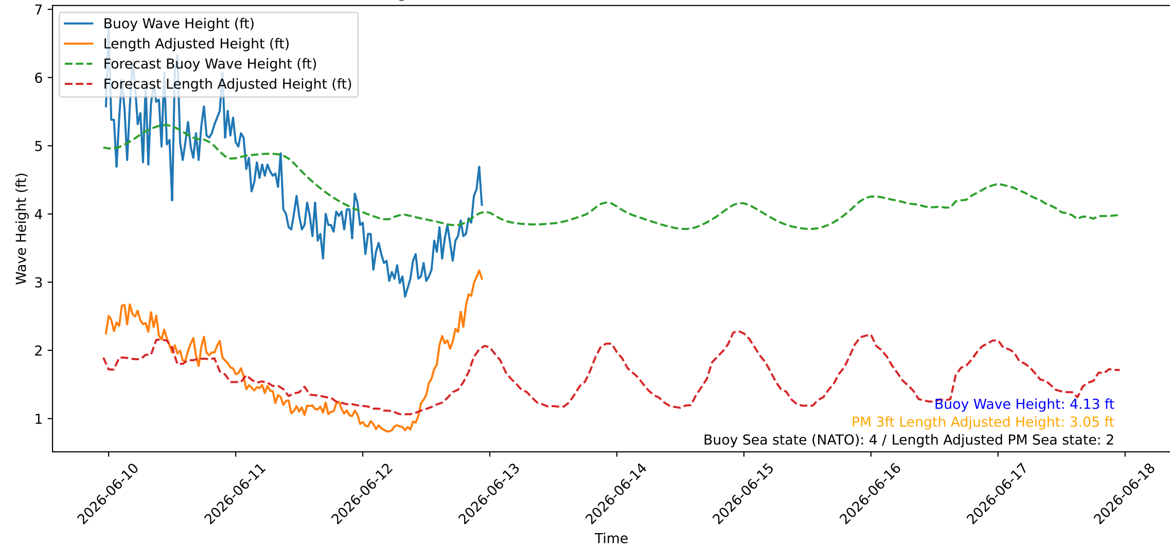
Wave Heights over Time for Oceanside Harbor at 2026-06-12 23:20:26
