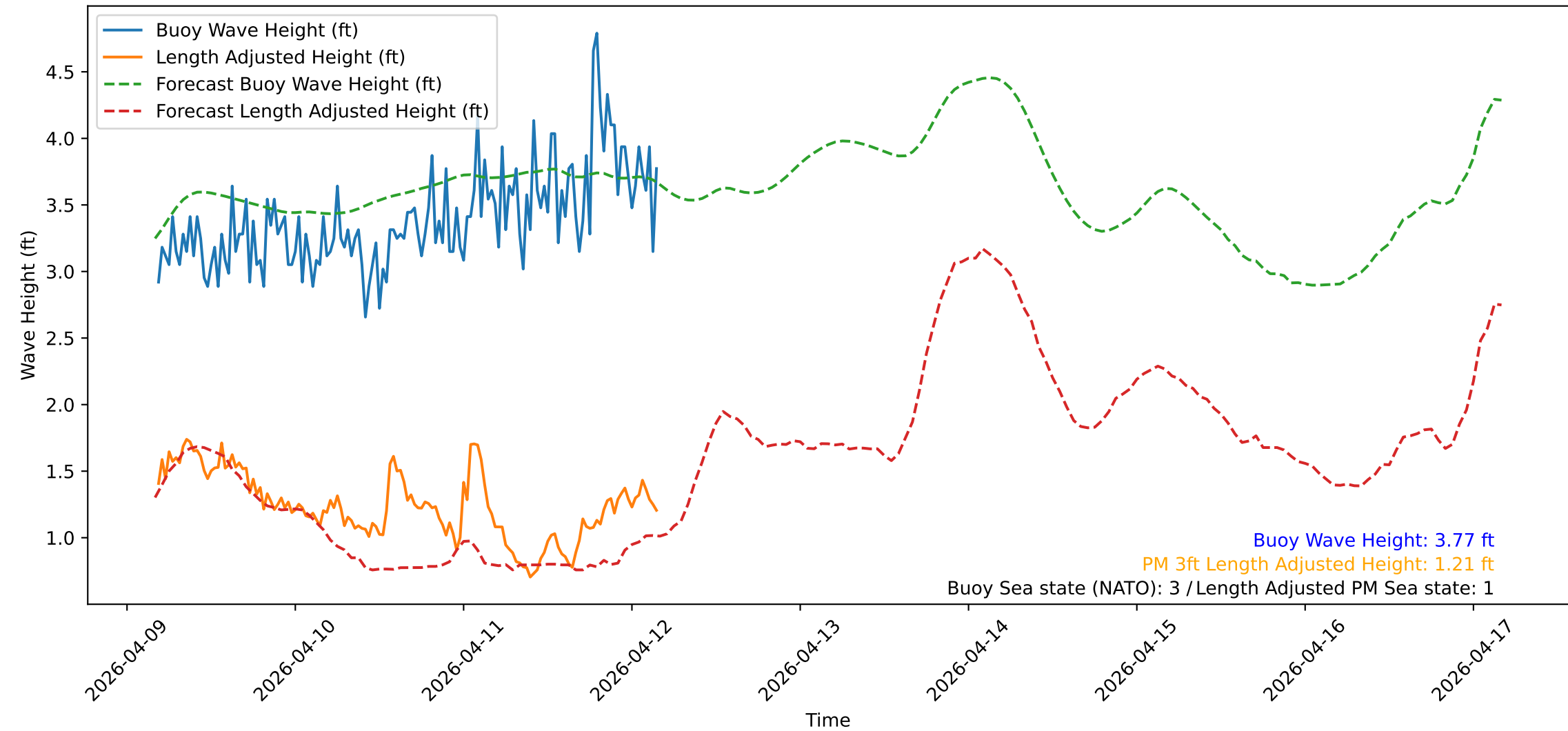
Wave Heights over Time for Oceanside Harbor at 2026-04-12 04:20:31
