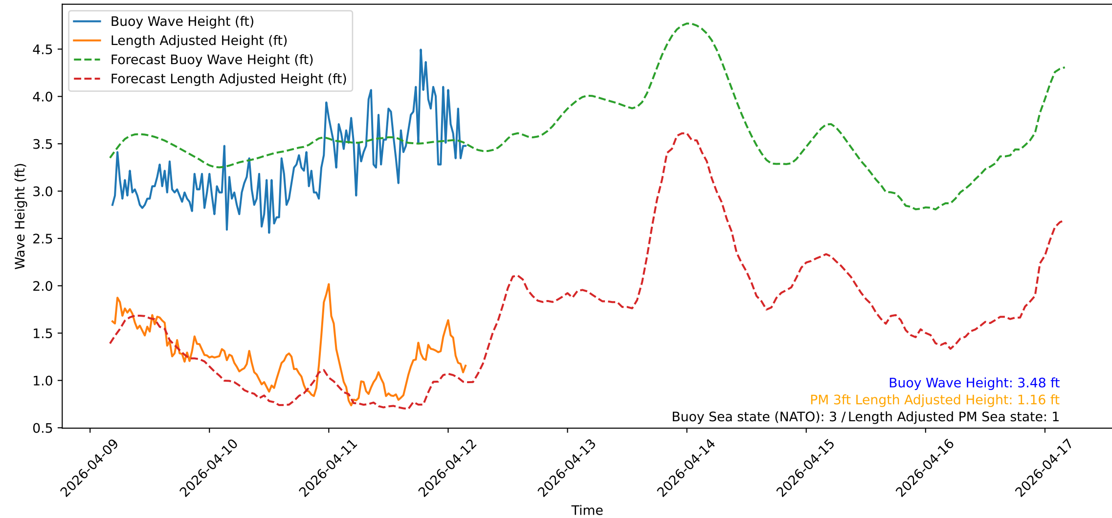
Wave Heights over Time for Green Beach at 2026-04-12 04:21:14
